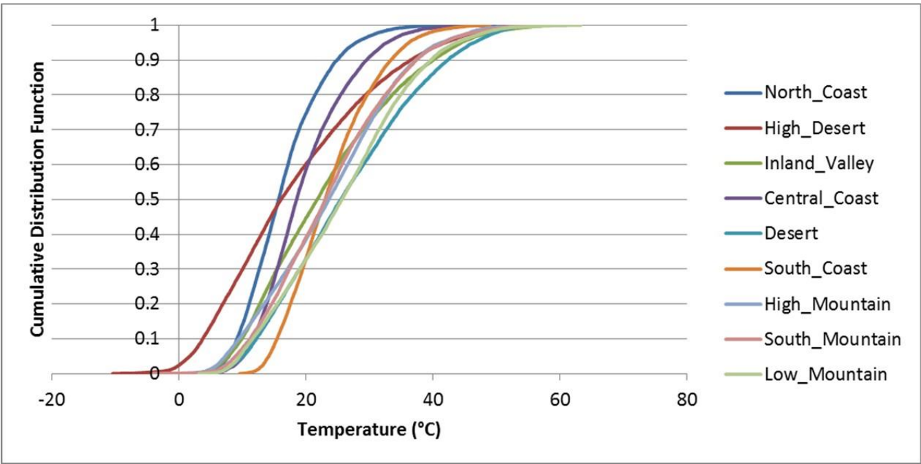
PD 08 - Pavement Temperature (1/3 Depth)
