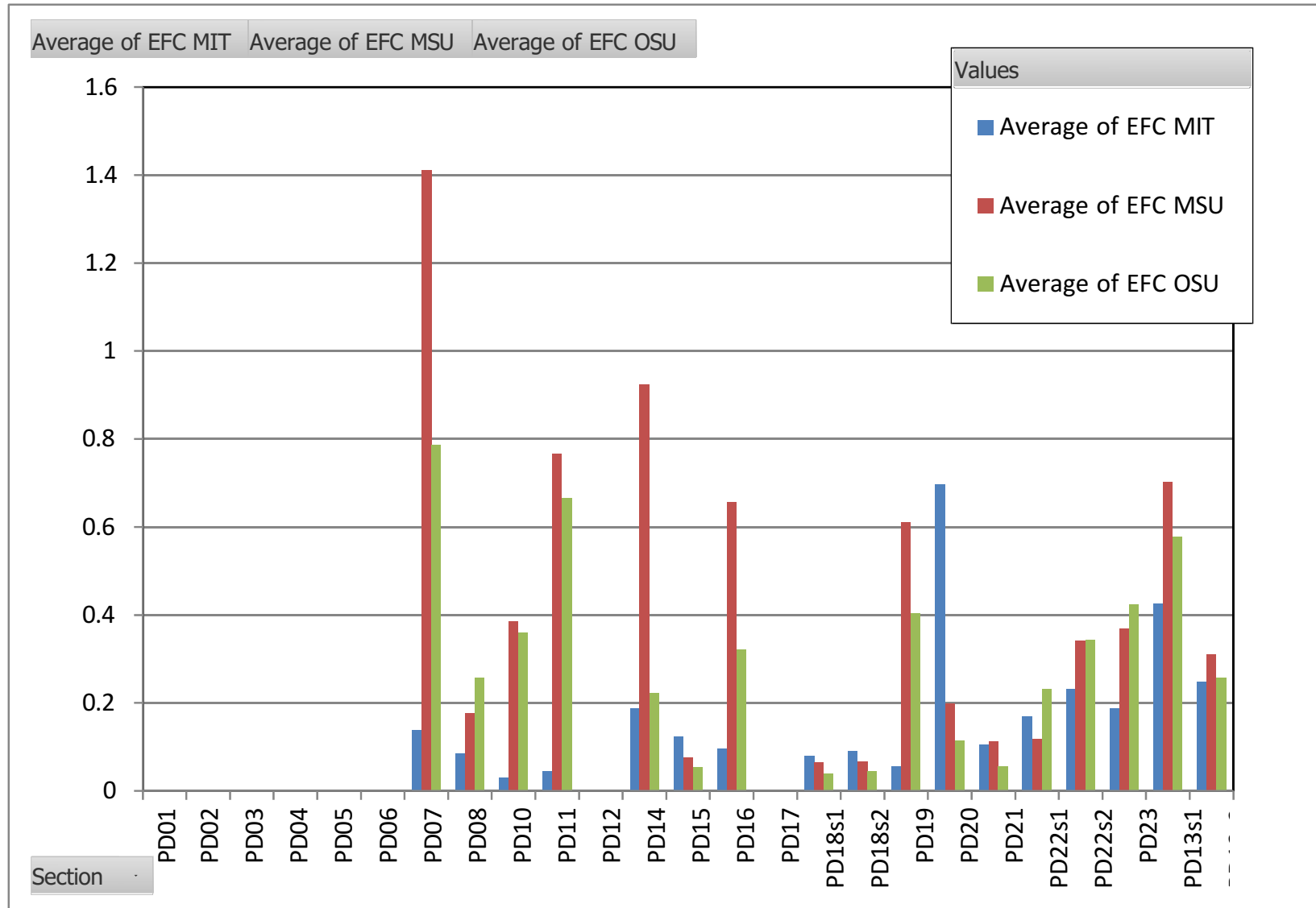
Figure 3.2: Average structural response simulation results in terms of Excess Fuel Consumption due to structural response (EFCs) by asphalt section relative to no structural response effect (avg mL/km/veh EFC) across traffic and climate factorial.
