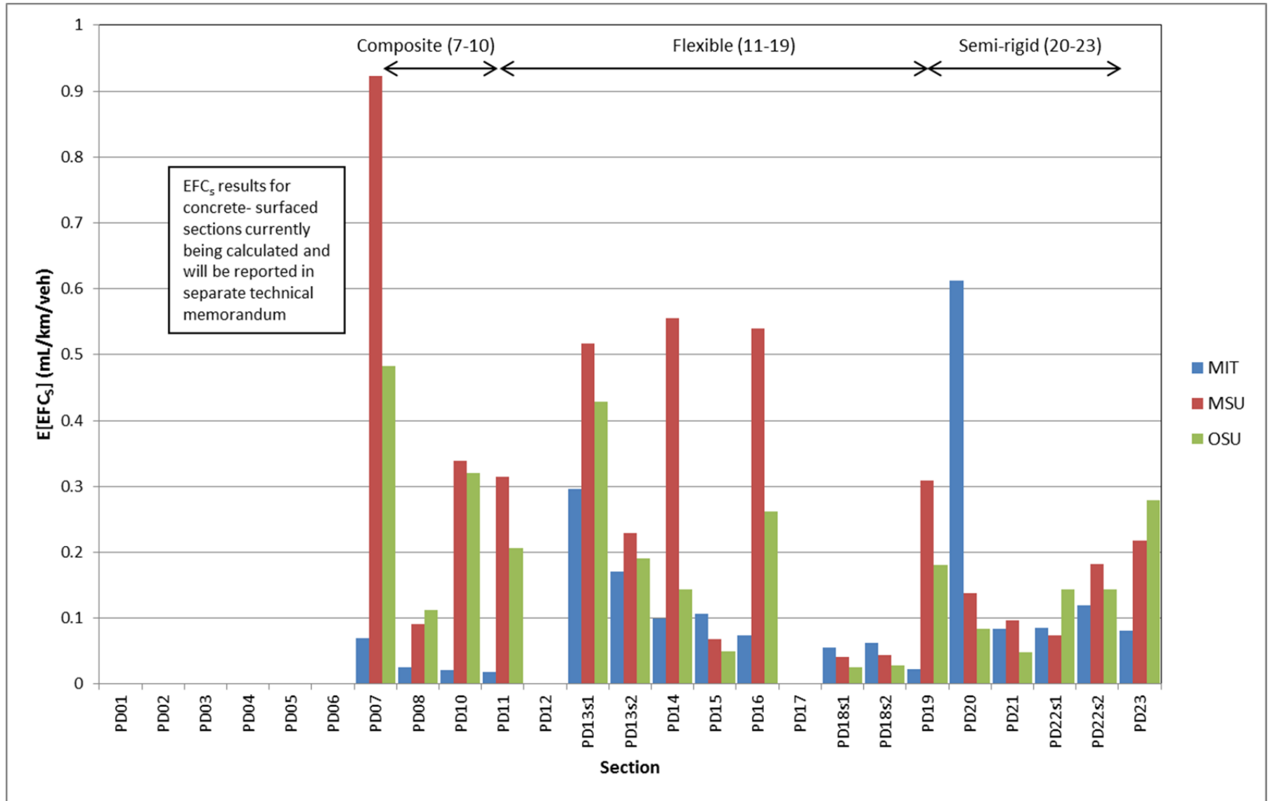
Figure 3.1: Average structural response simulation results in terms of Excess Fuel Consumption due to structural response (EFCs) by asphalt section relative to no structural response effect (avg mL/km/veh EFC) simulated with section-specific traffic and climate.
