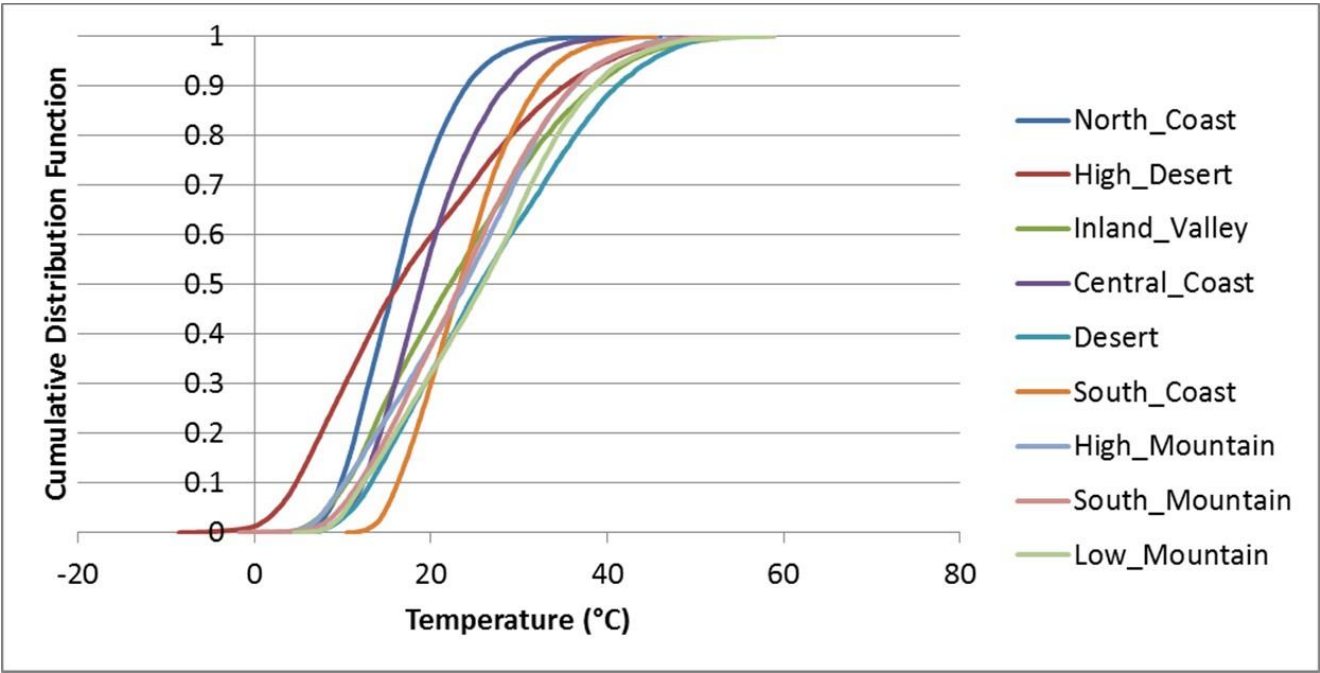
PD 18s2 - Pavement Temperature (1/3 Depth)
