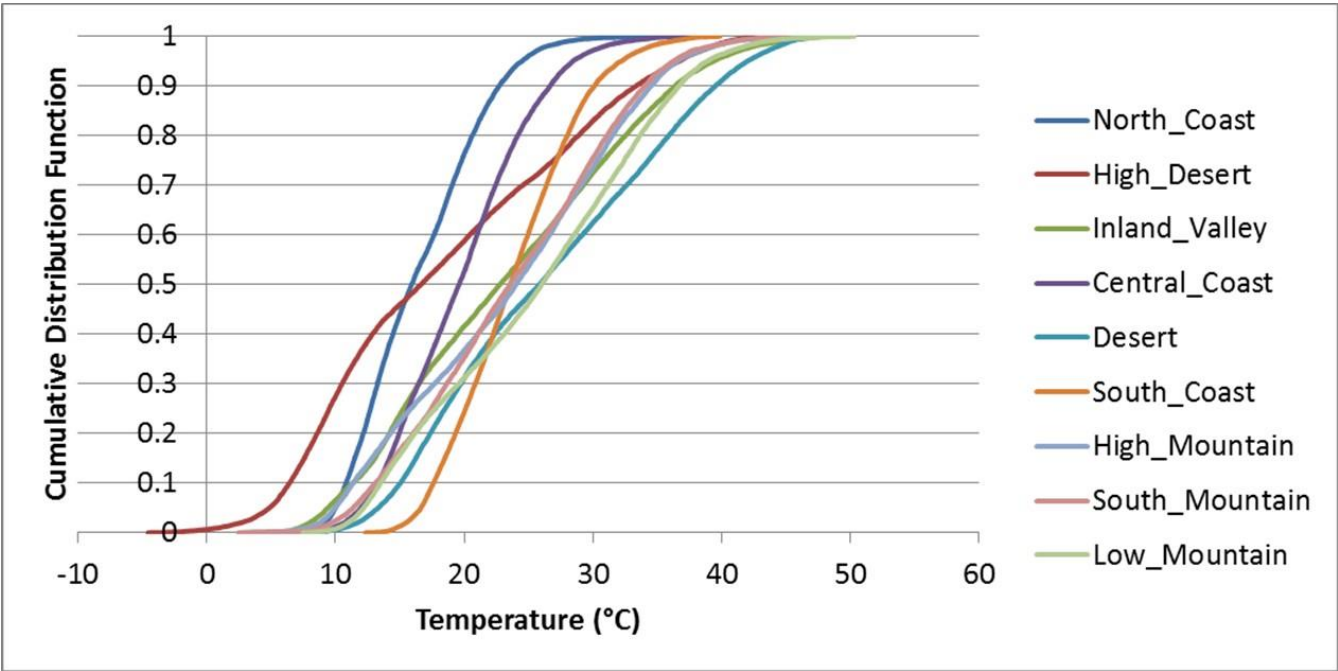
PD 13s1 - Pavement Temperature (1/3 Depth)
