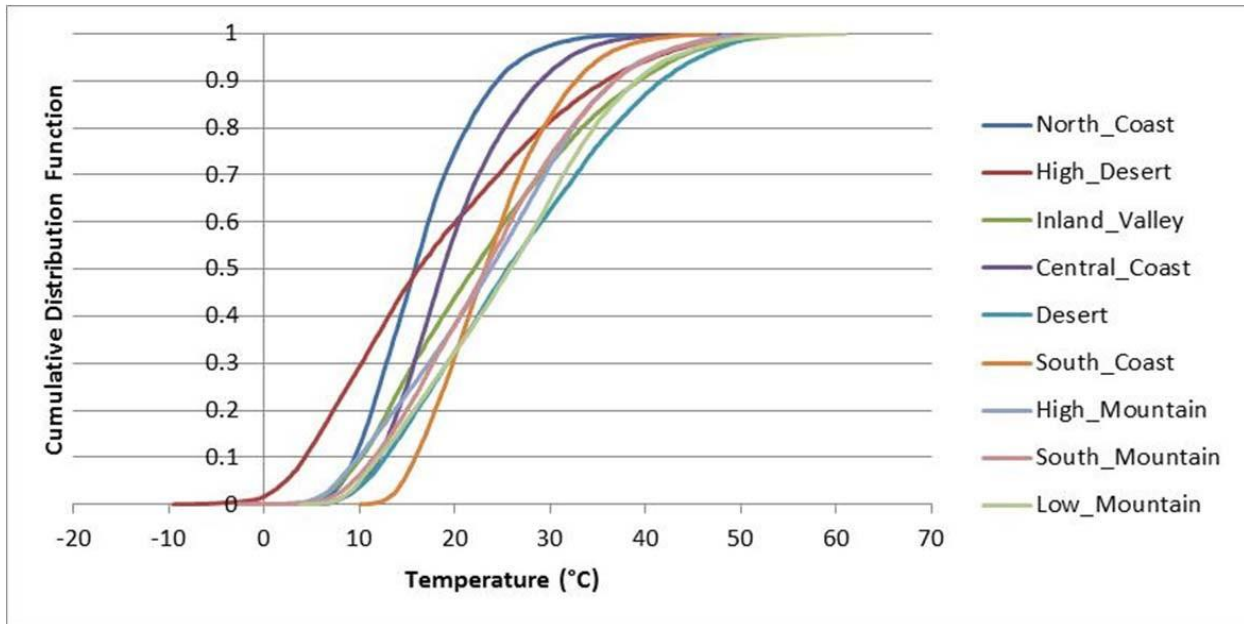
Figure 2.7: Example cumulative distributions of pavement temperature at one-third of asphalt depth from CalME 1-d approximation and interpolation based on database of EICM runs for nine California climate regions (PD 7 example shown). (Note: 0°C = 32°F, 20°C = 67°F, 40°C = 104°F, 60°C = 140°F.)
