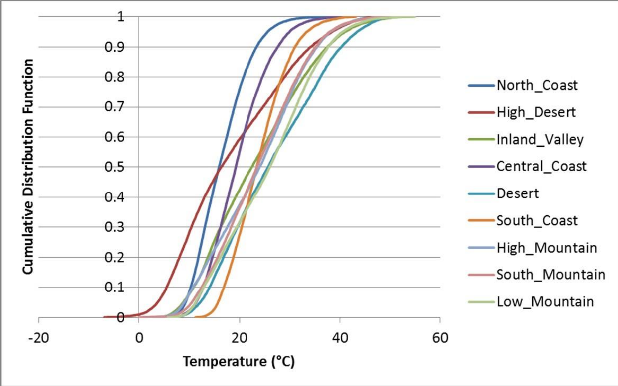
PD 21 - Pavement Temperature (1/3 Depth)
