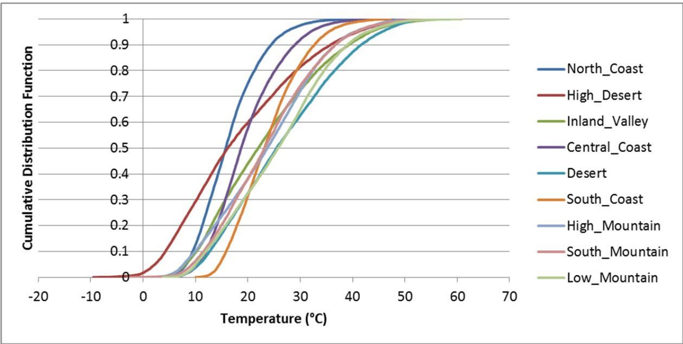
PD 07 - Pavement Temperature (1/3 Depth)
