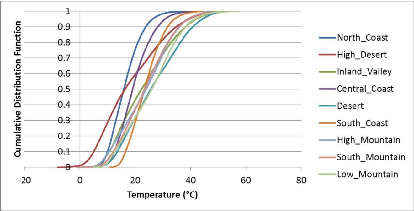
PD 15 - Pavement Temperature (1/3 Depth)
