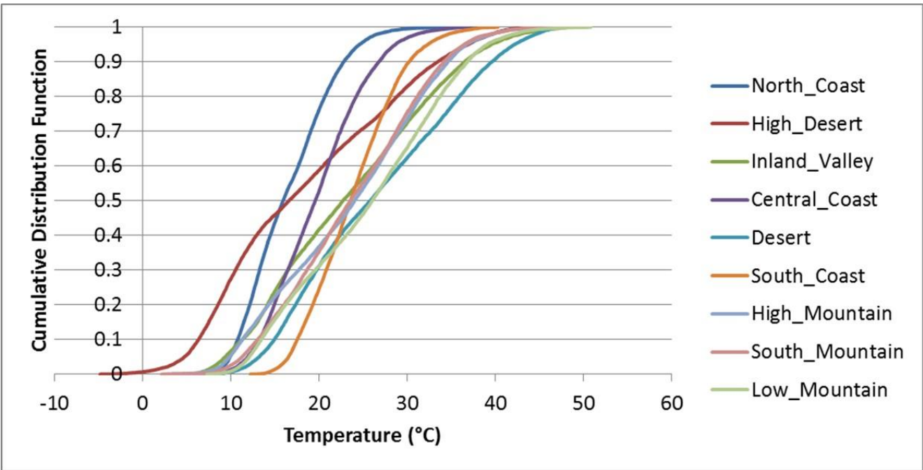
PD 13s2 - Pavement Temperature (1/3 Depth)
