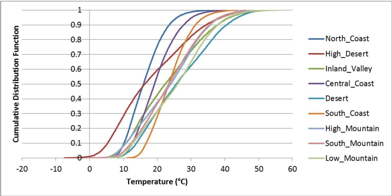
PD 10 - Pavement Temperature (1/3 Depth)
