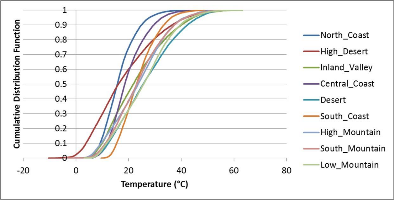
PD 20 - Pavement Temperature (1/3 Depth)
