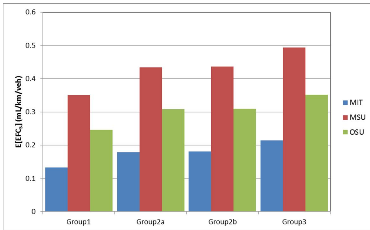
Figure 4.4: Average structural response simulation results by axle load spectrum group across factorial.
