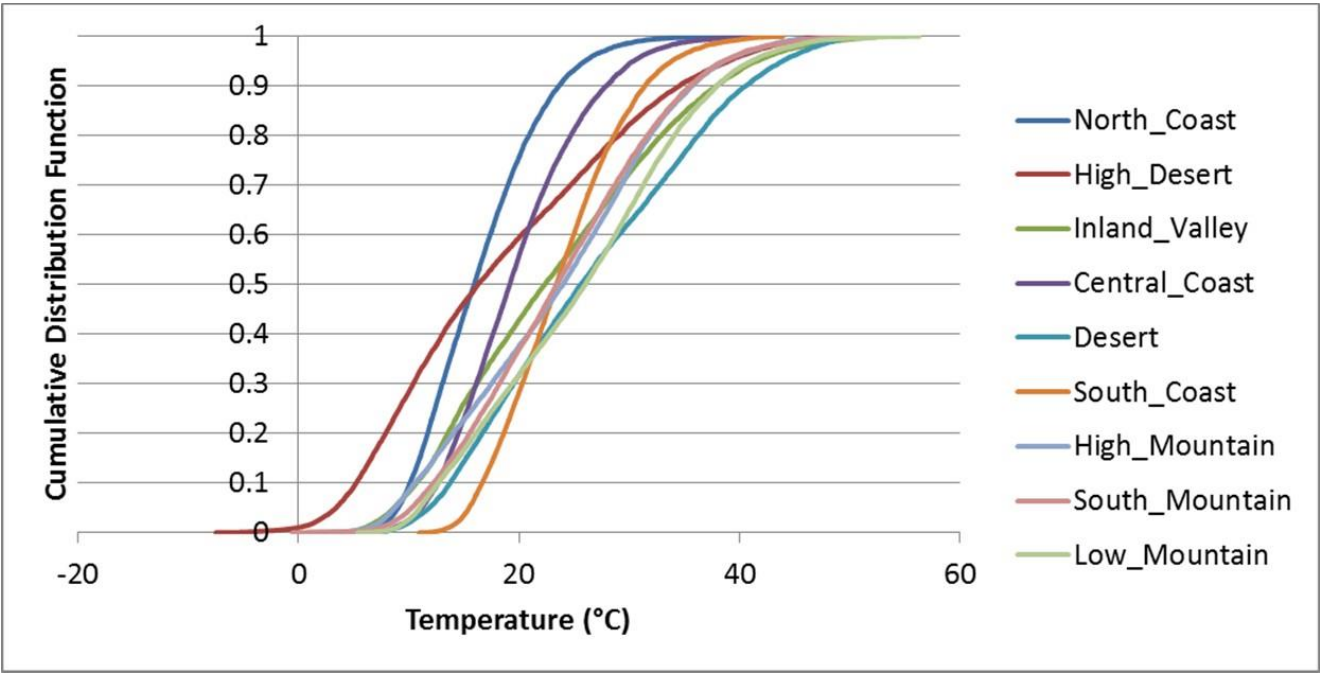
PD 14 - Pavement Temperature (1/3 Depth)
