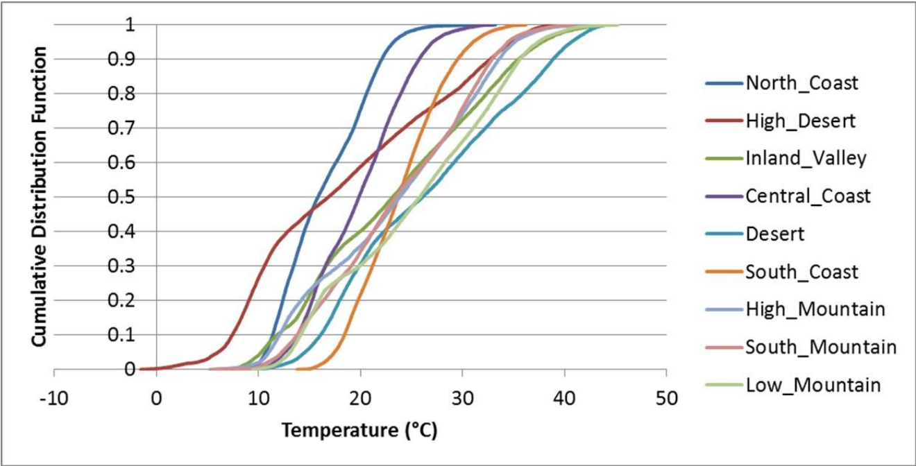
PD 19 - Pavement Temperature (1/3 Depth)
