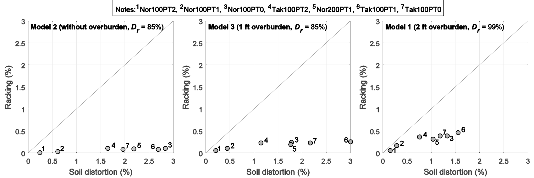
Figure 3–12: Relationship of the peak racking and the ground distortion between top and bottom of the tunnel
