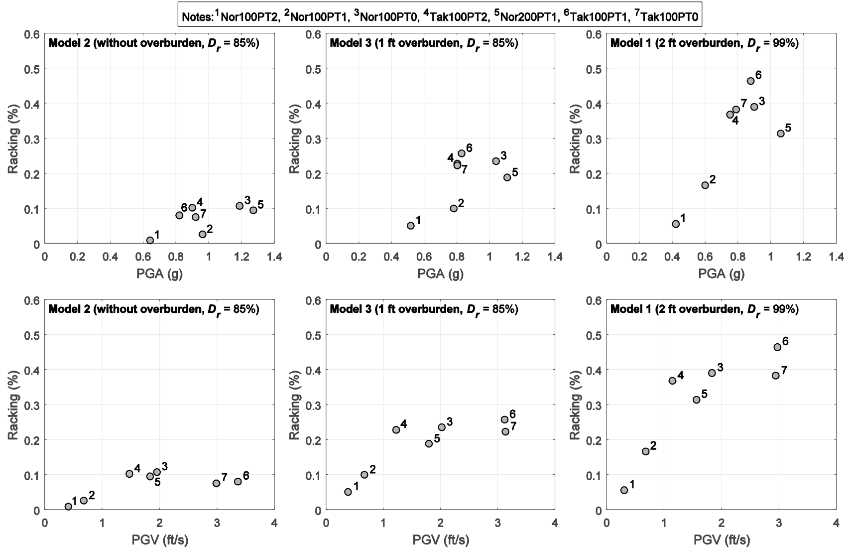
Figure 3–10: Correlation of peak racking with peak ground acceleration (top) and peak ground velocity (bottom)
