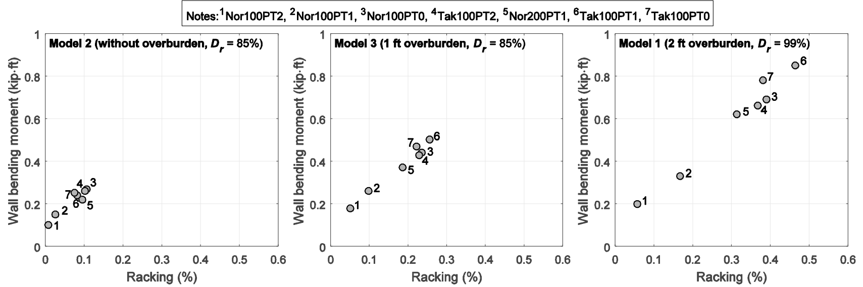
Figure 3–11: Relationship between the peak racking and the peak wall bending moment
