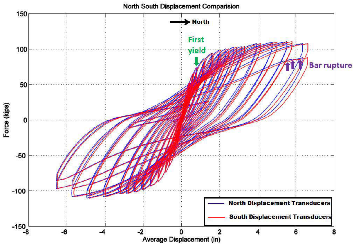
Figure G-5: Relationship of laterl force and displacement in model scale
