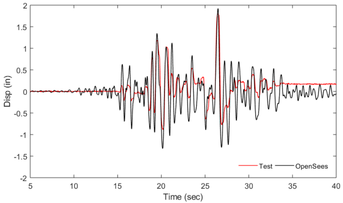
Figure F-11: Racking time history from Model 1 Nor100PT1 in prototype scale
