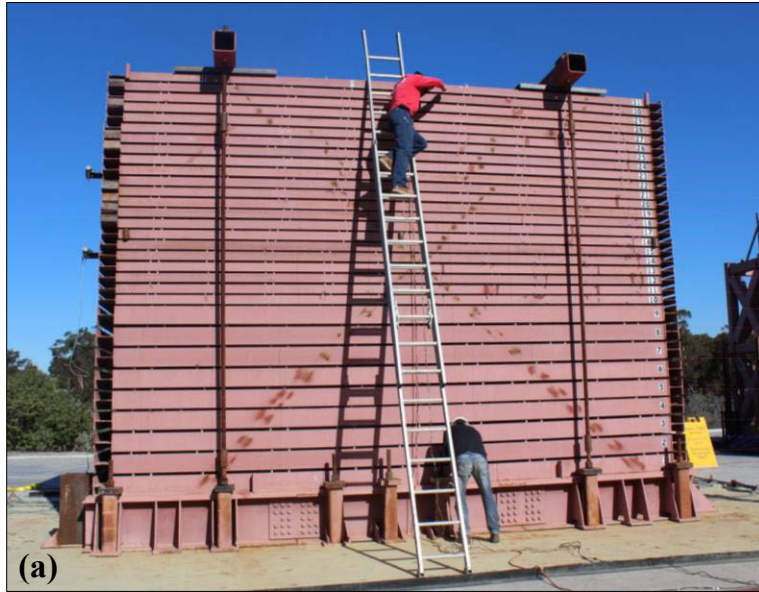
Figure 2-1: Pictures of shake table test model; (a) North view and (b) East view
