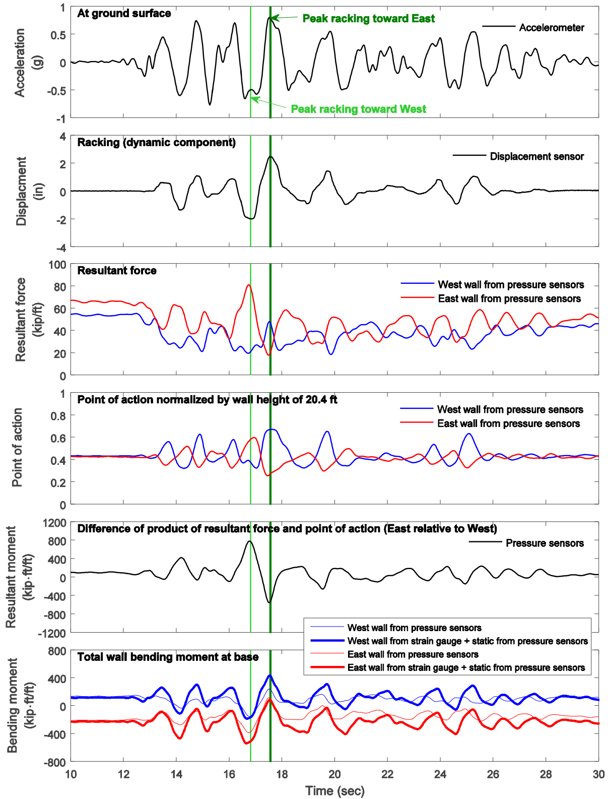
Figure 5–13: Model 3 resultant earth pressure force, point of action, and total wall bending moment at wall base for Tak100PT2 in prototype scale (9 ft overburden soil)
