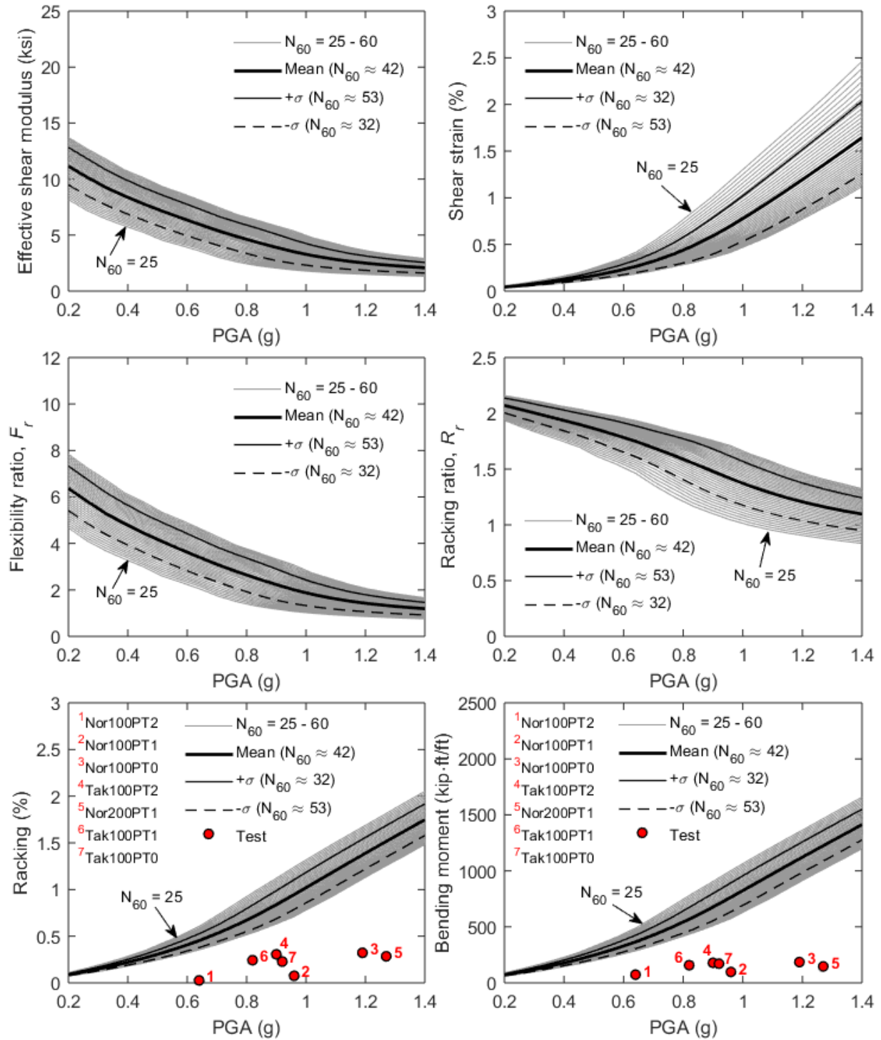
Figure 6–8: Model 2 without overburden soil: variation of FHWA parameters varied with N_{60} from 25 to 60 along with test results (marked in red dots) in prototype scale
