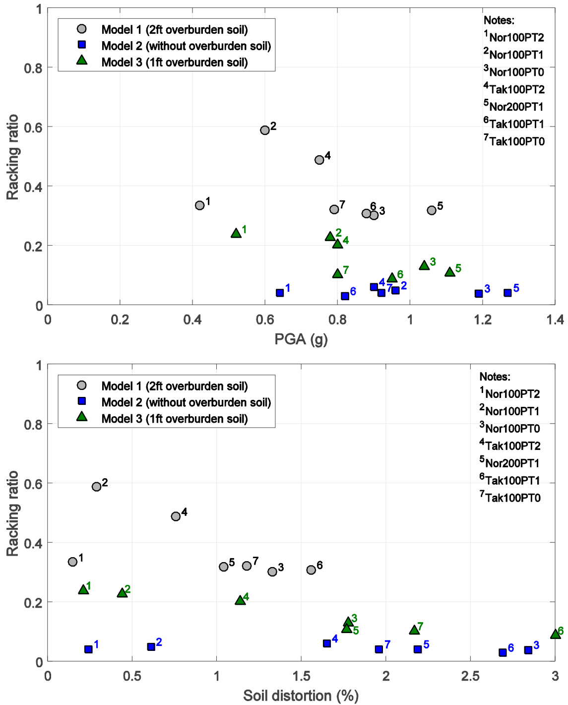
Figure 3–13: Relationship of racking ratio with peak ground acceleration (top) and soil distortion between top and bottom of tunnel (bottom)
