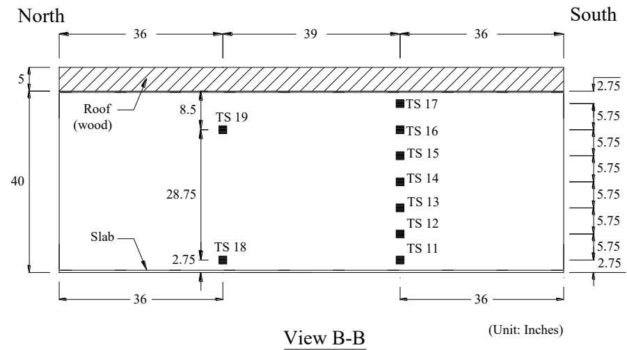
Figure 4-1: Tactilus pressure sensor (TS) layout along the tunnel walls
