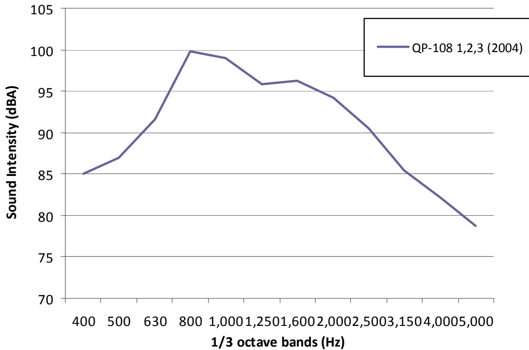
Figure 3.14: OBSI spectral content for longitudinally timed sections, texture worn out .
