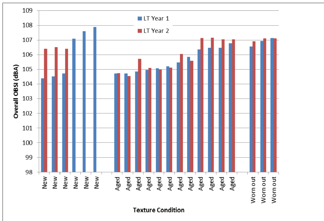
Figure E.8: Compare with Figure 3.38: Longitudinally tined Year 1 and Year 2 results for all texture conditions ( new, aged, worn out ).
