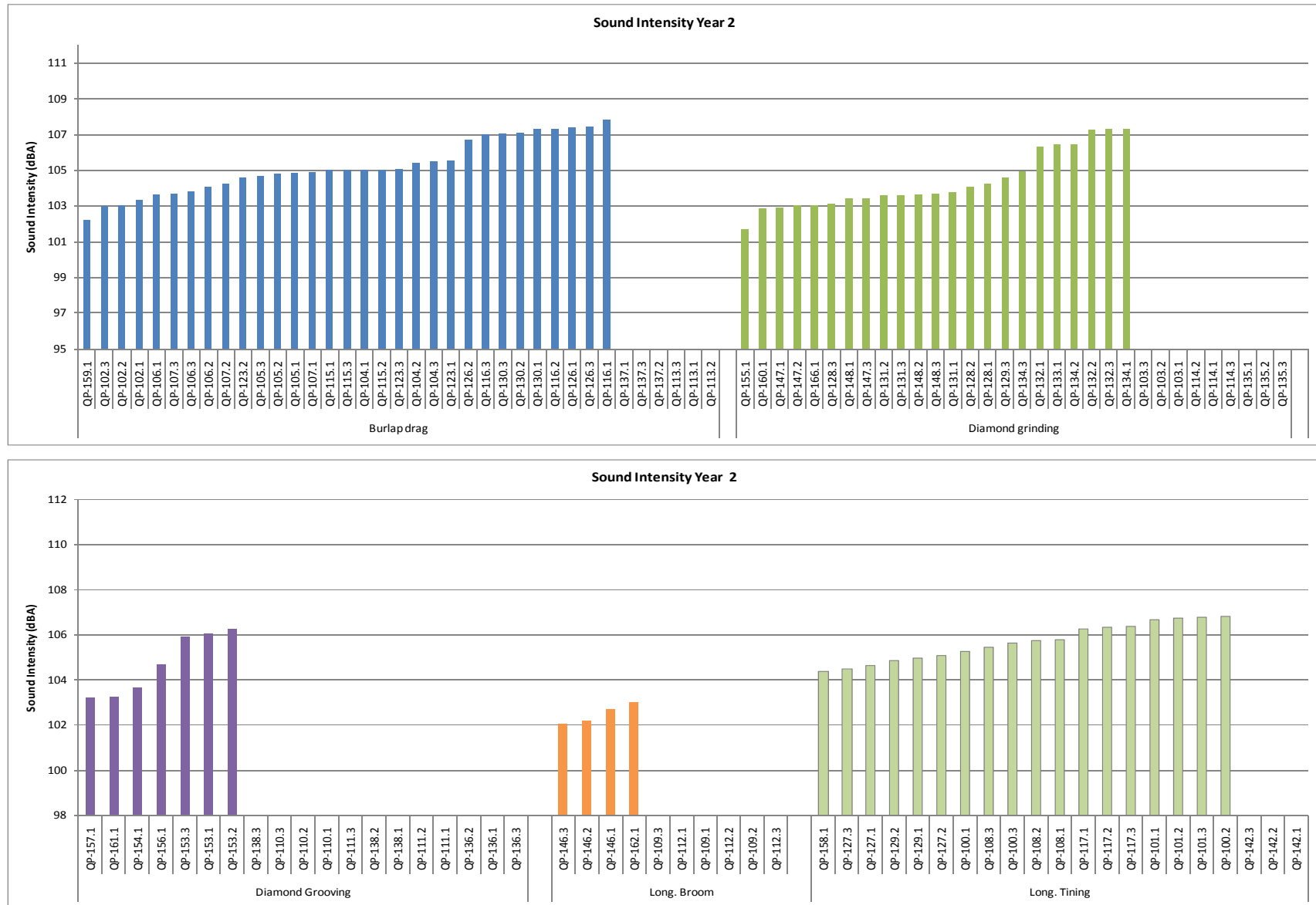
Figure B.2: On-board Sound Intensity levels of all sections as measured in Year 2.
