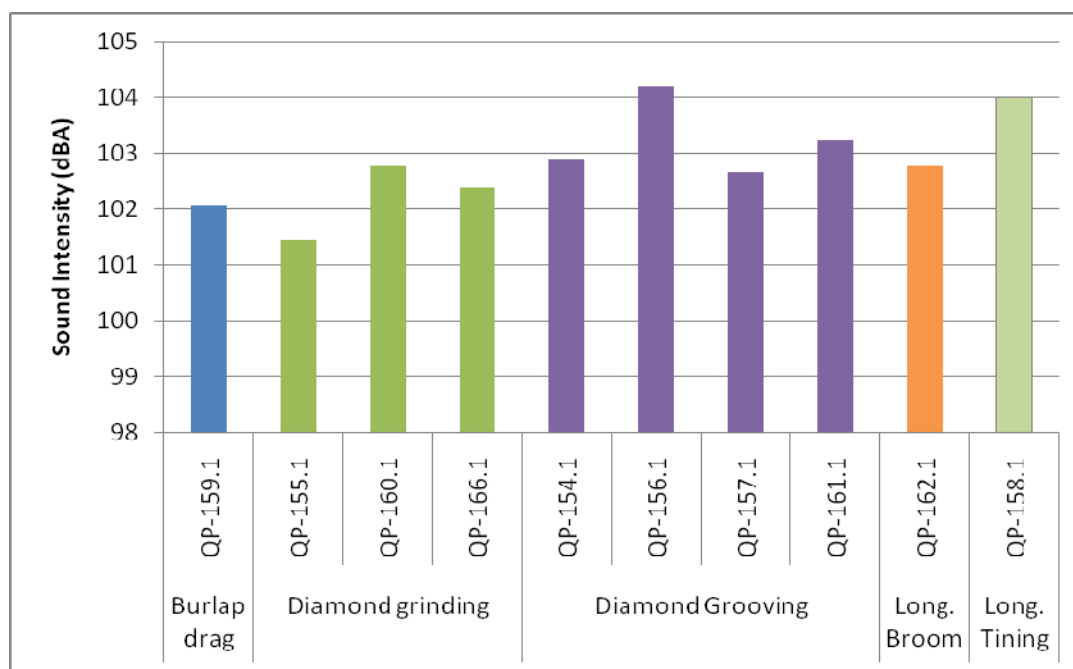
Figure 4.6: Comparison of OBSI noise levels of concrete pavement textures in Mojave sections averaged over the two years of measurement.
