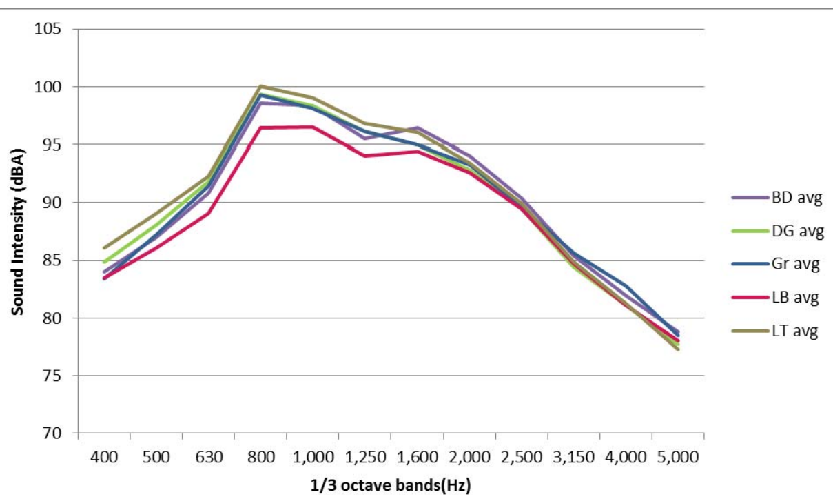
Figure E.1: Figure 3.17: Comparison of OBSI spectral content of sections with different texture types, average of sections with texture aged.
