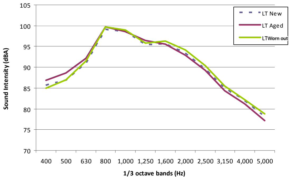
Figure 3.15: Comparison of OBSI spectral content for longitudinally timed sections with texture in different conditions.
