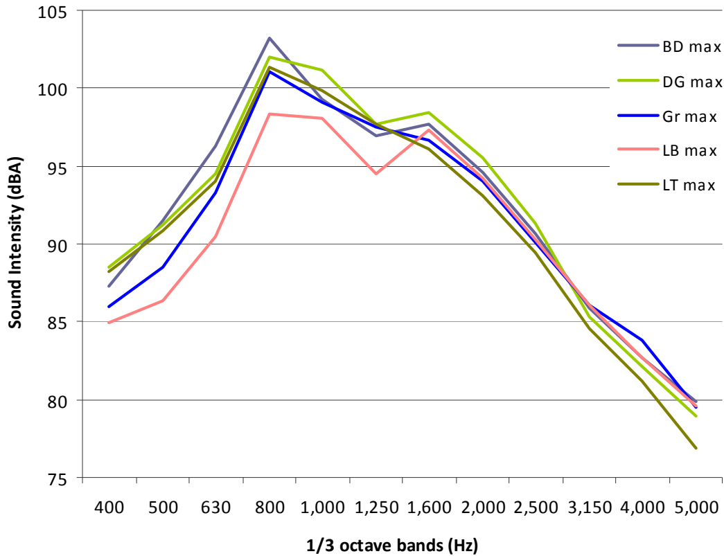
Figure 3.20: Comparison of OBSI spectral content of sections with different texture types, maximum of sections with texture aged . (Note: BD = burlap drag, DG=diamond ground, Gr=diamond grooved, LB=longitudinally broomed, LT=longitudinally tined.)
