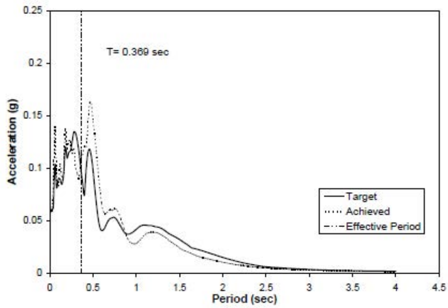
Fig. 3-143. Target vs. Achieved Ground Motion Spectra, Run-1 in SE-2
