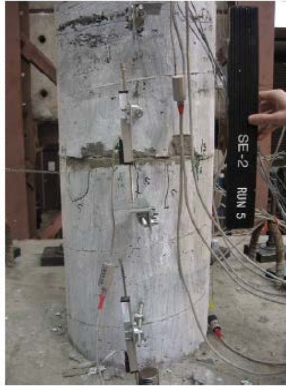
b) SE-2 Column, South, Run-5
