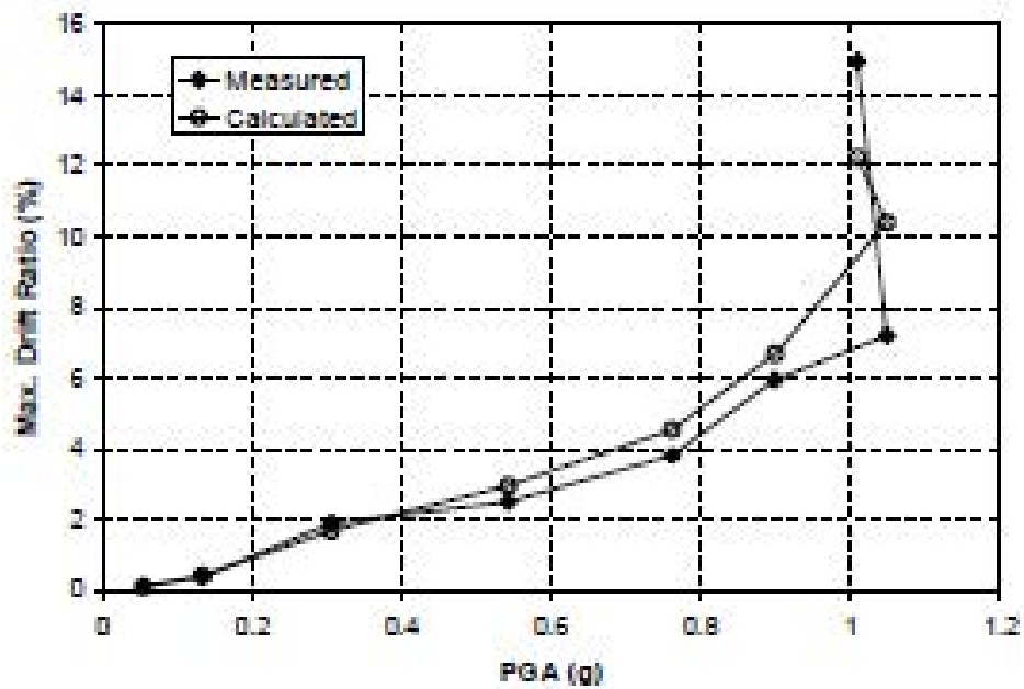
Fig. 6-33. Maximum Drift Ratio vs. PGA in SF-2
