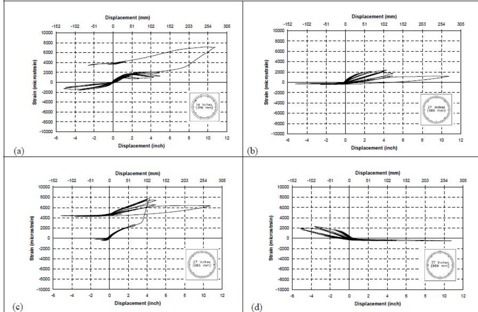
Fig. A-39. a) sg 34, b) sg 35, c) sg 36, d) sg 37 in SF-2
