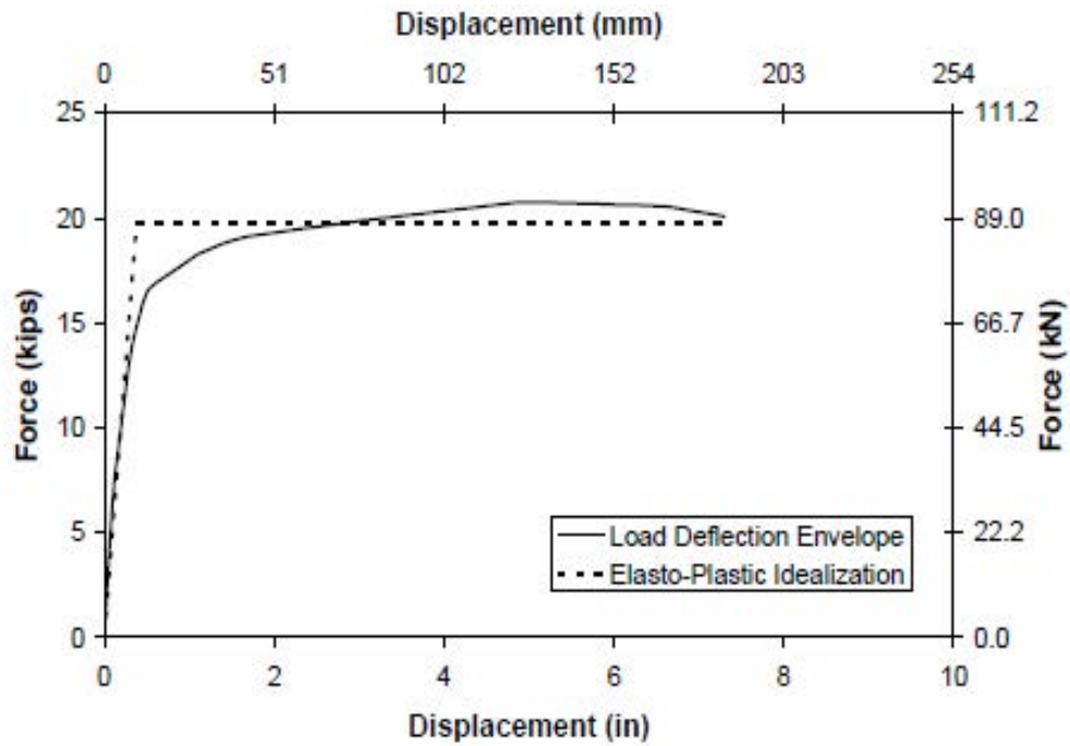
Fig. 3-126. Backbone Curve of SE-2
