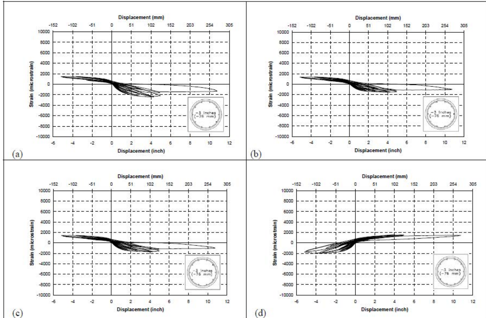
Fig. A-31. a) sg 5, b) sg 6, c) sg 7, d) sg 8 in SF-2
