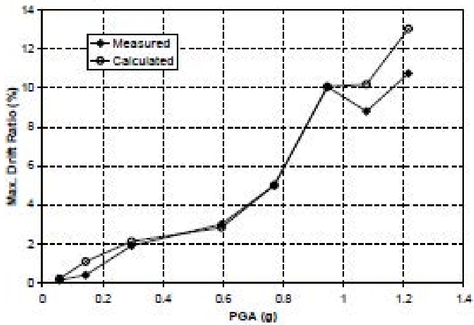
Fig. 6-35. Maximum Drift Ratio vs. PGA in SE-2
