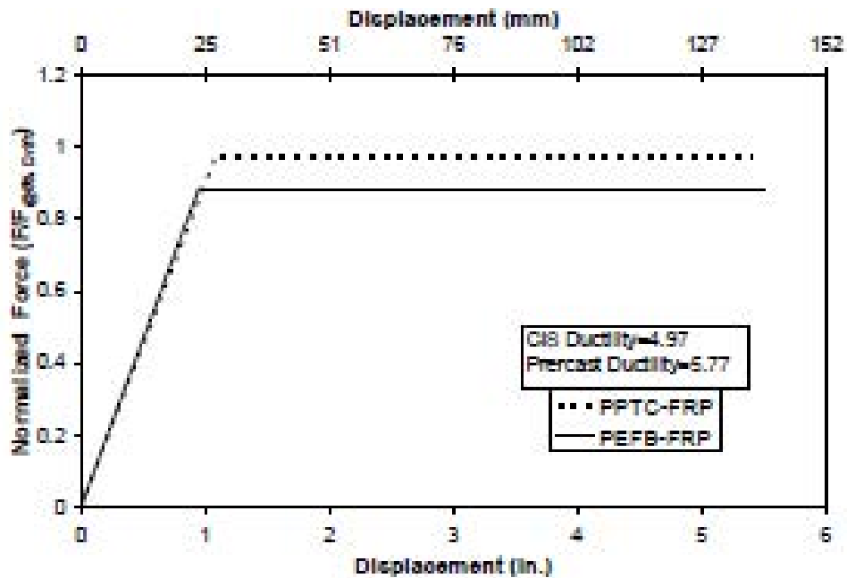
Fig. 4-24. Comparison of Elasto-Plastic Curves for FRP Columns in PEFB and PPTC
