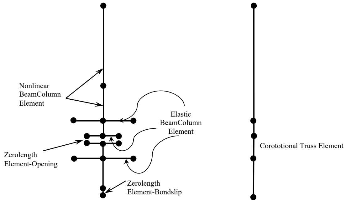
Fig. 6-7. Schematic Analytical Model for Segmental Columns
