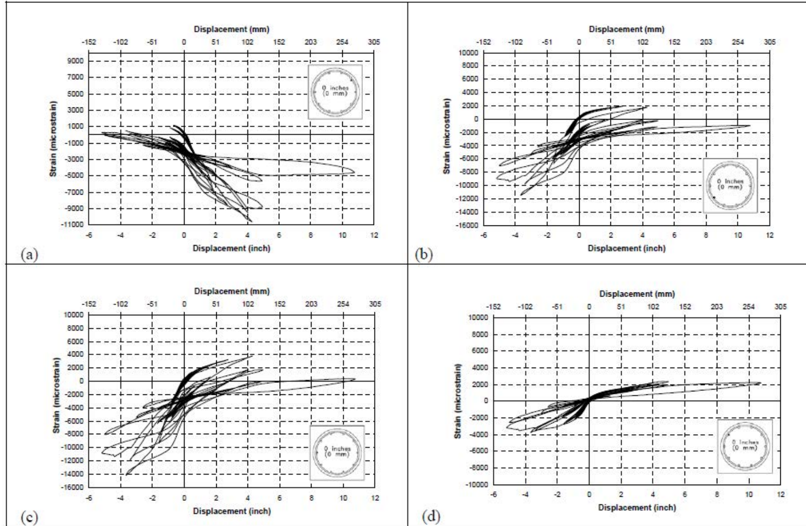
Fig. A-33. a) sg 13, b) sg 14, c) sg 15, d) sg 16 in SF-2
