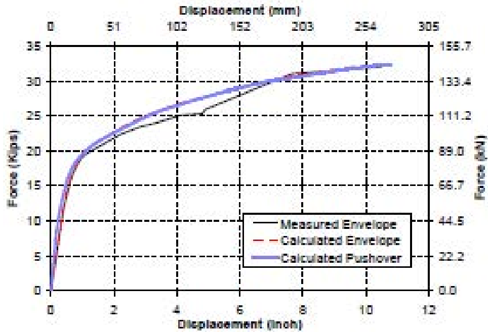
Fig. 6-13. Pushover and Average Backbone Curves of SC-2R
