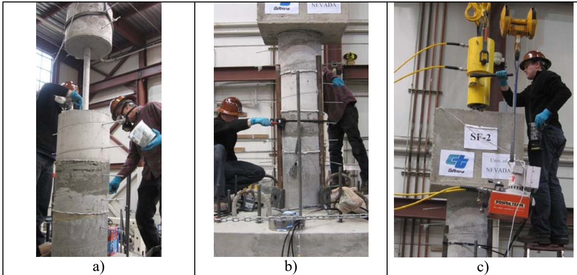
Fig. 2-9. Columns Assembly, a) Setting the Segments, b) Adjusting the Segments, c) Post-Tensioning
