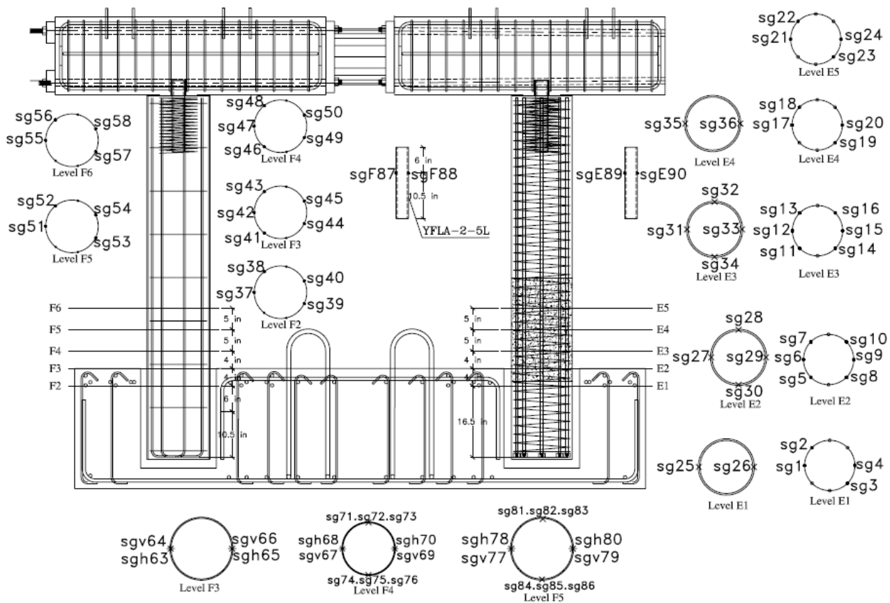
Fig. 2-82. PEFB Strain Gauge Plan
