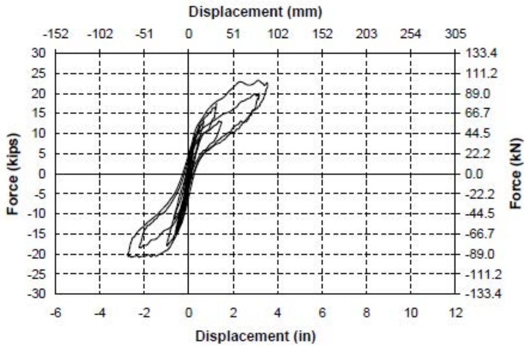
Fig. 3-10. Force-Displacement Hysteresis Curve for Run 5 in SC-2
