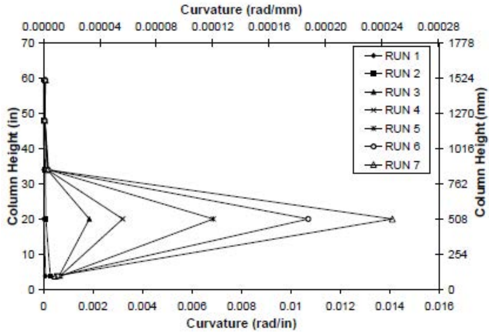
Fig. 3-20. Curvature Profile for SC-2
