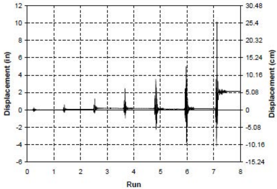
Fig. 3-62. Displacement History in Column SBR-1
