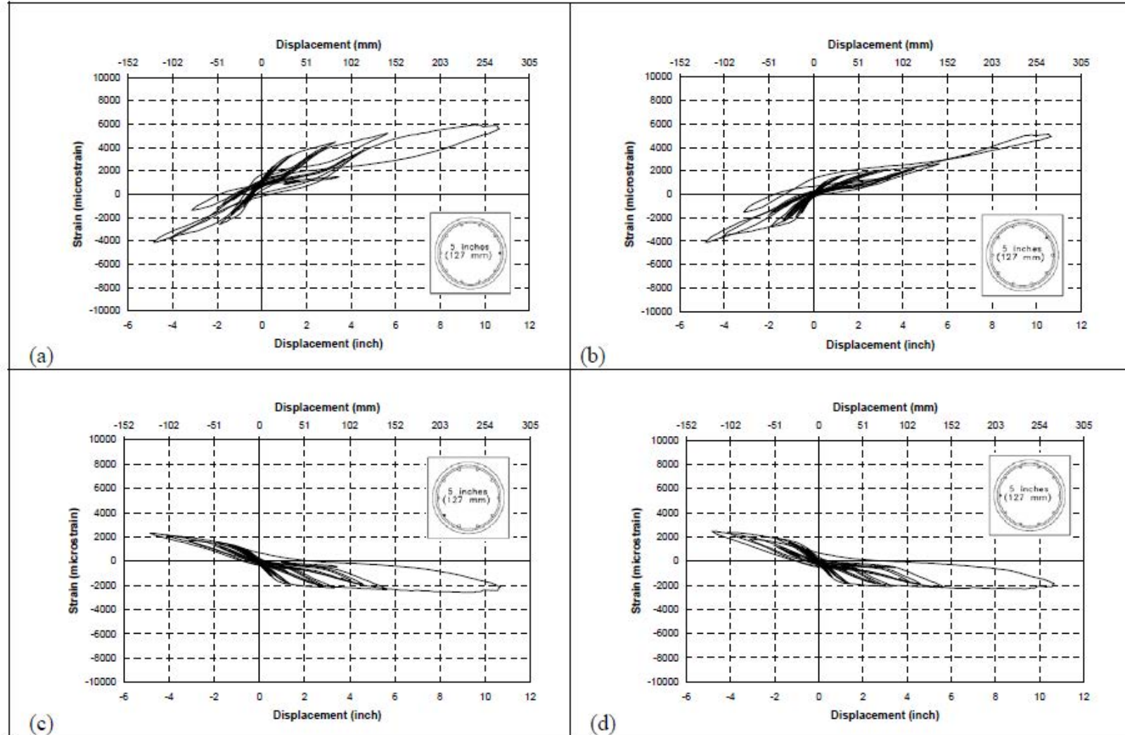
Fig. A-67. a) sg 18, b) sg 19, c) sg 20, d) sg 21 in SC-2R
