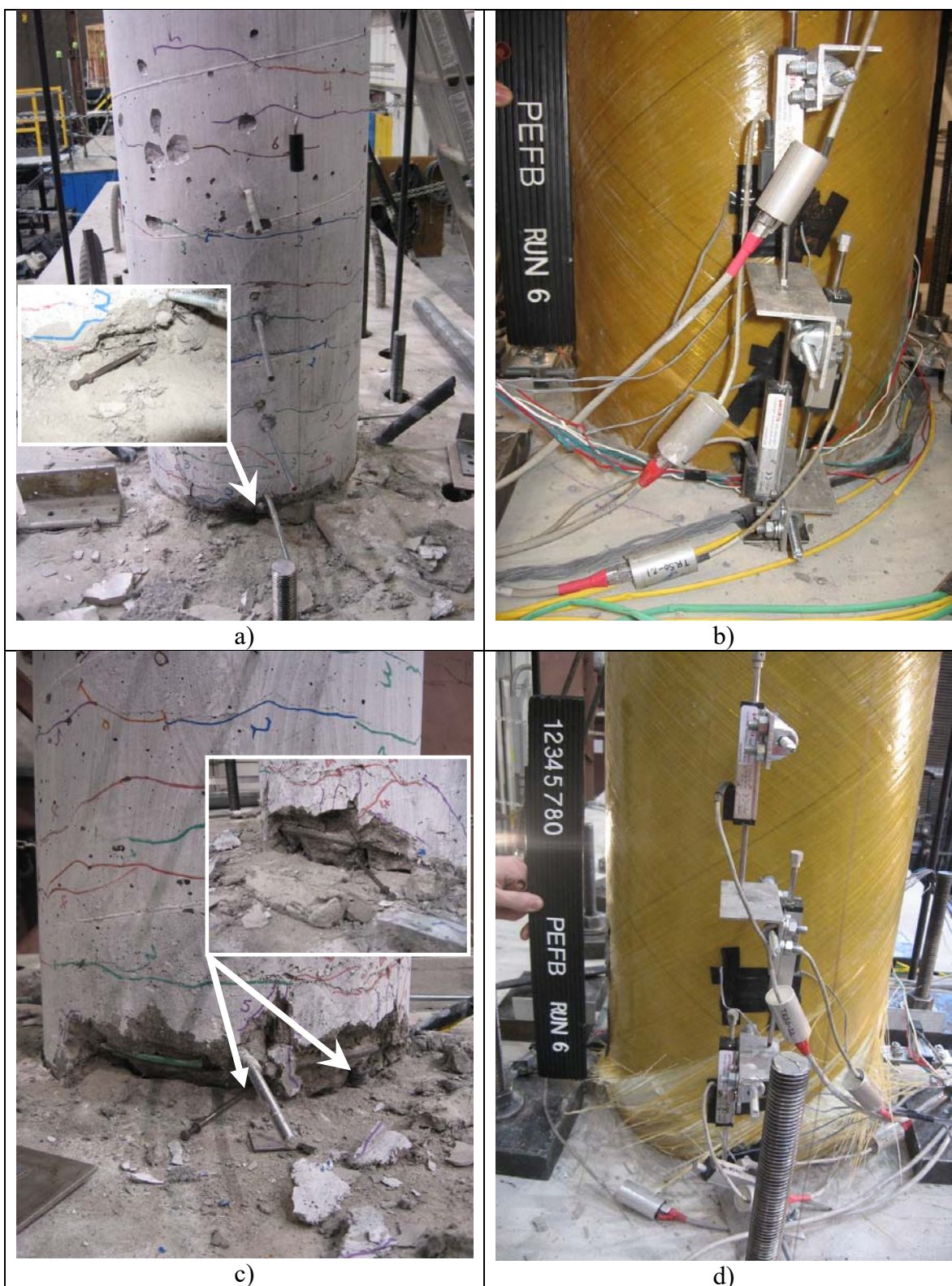
Fig. 4-12. Apparent Damage at 10% Drift for a) RC-ECC, North, b) FRP, North, c) RC-ECC, South, d) FRP, South
