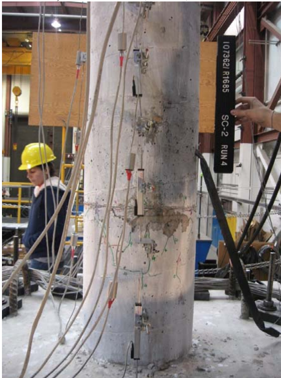
c) SC-2 Column, North, Run-4
