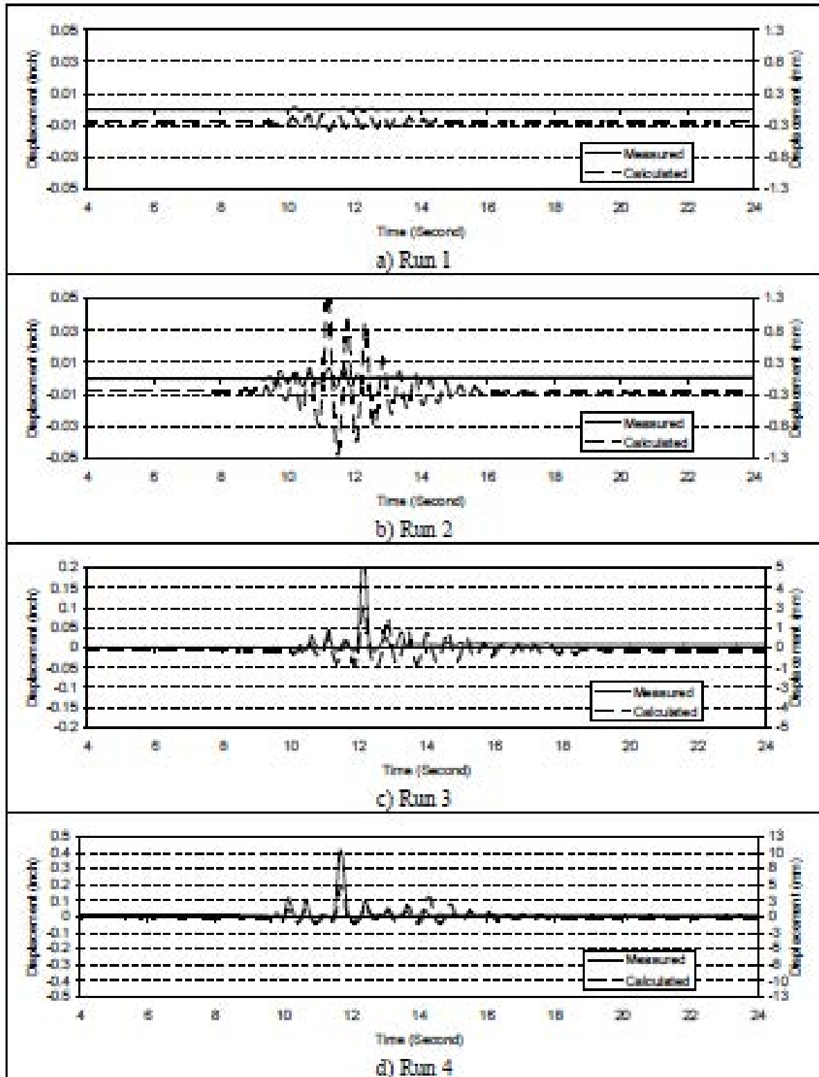
Fig. 6-47. History of Opening at the South Side of the SC-2, Run 1 through Run 4
