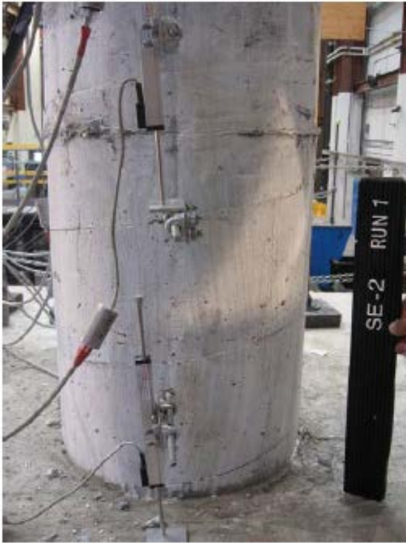
SE-2 Column, North, Run-1
