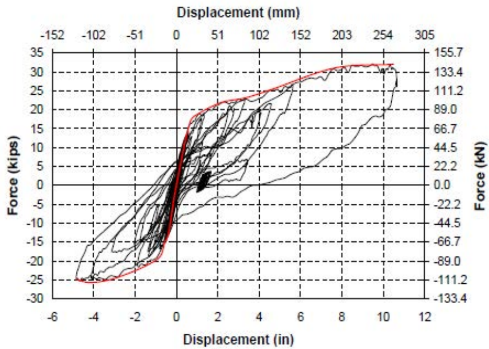
Fig. 3-154. Accumulated Force-Displacement Hysteresis Curve for SC-2R
