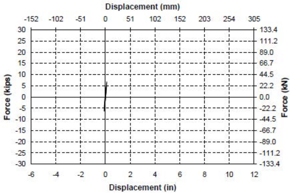
Fig. 3-6. Force-Displacement Hysteresis Curve for Run 1 in SC-2
