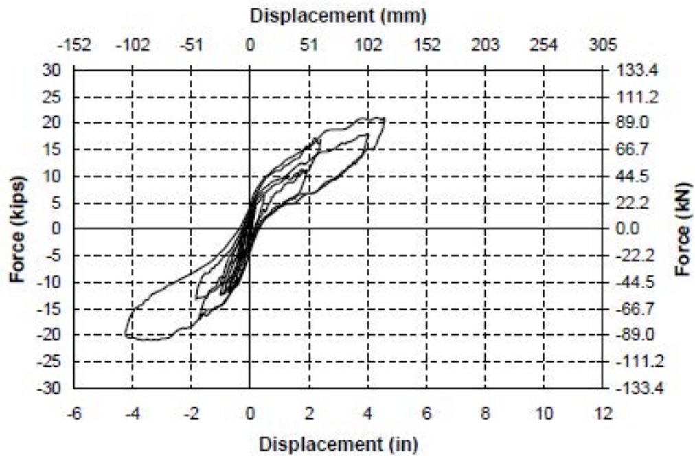
Fig. 3-11. Force-Displacement Hysteresis Curve for Run 6 in SC-2
