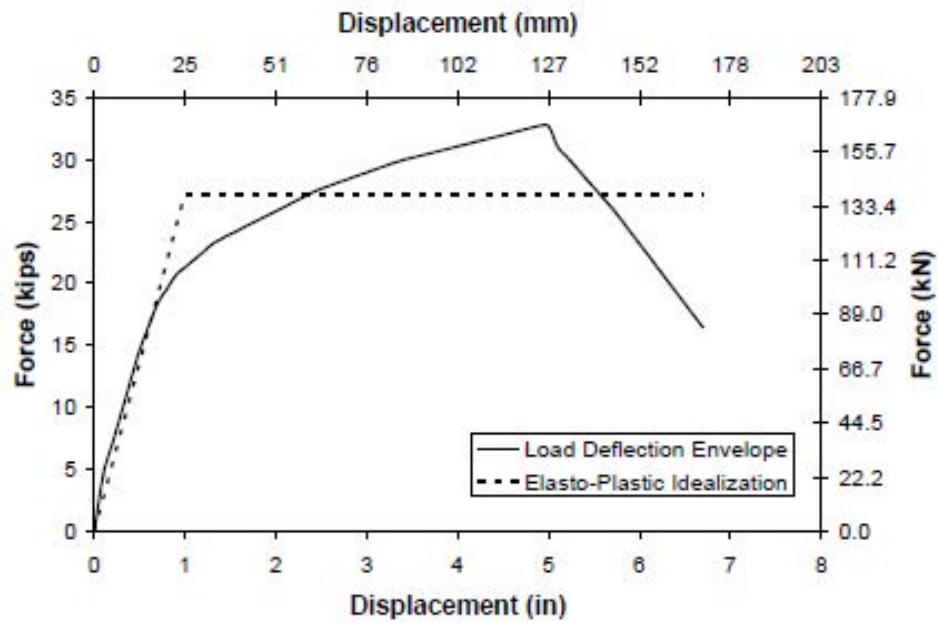
Fig. 3-221. Backbone Curve of FRP Column
