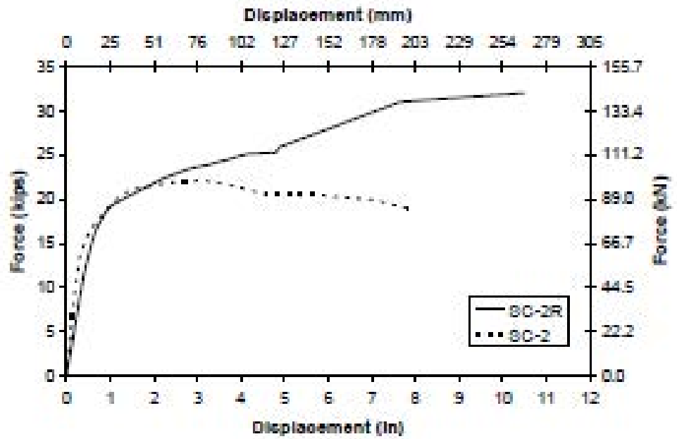
Fig. 4-7. Comparison of Backbone Curves in SC-2R and SC-2
