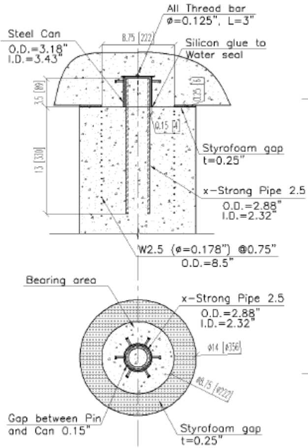
Fig. 2-61. PEFB Pipe-Pin Detail [Zaghi and Saiidi, 2010a]
