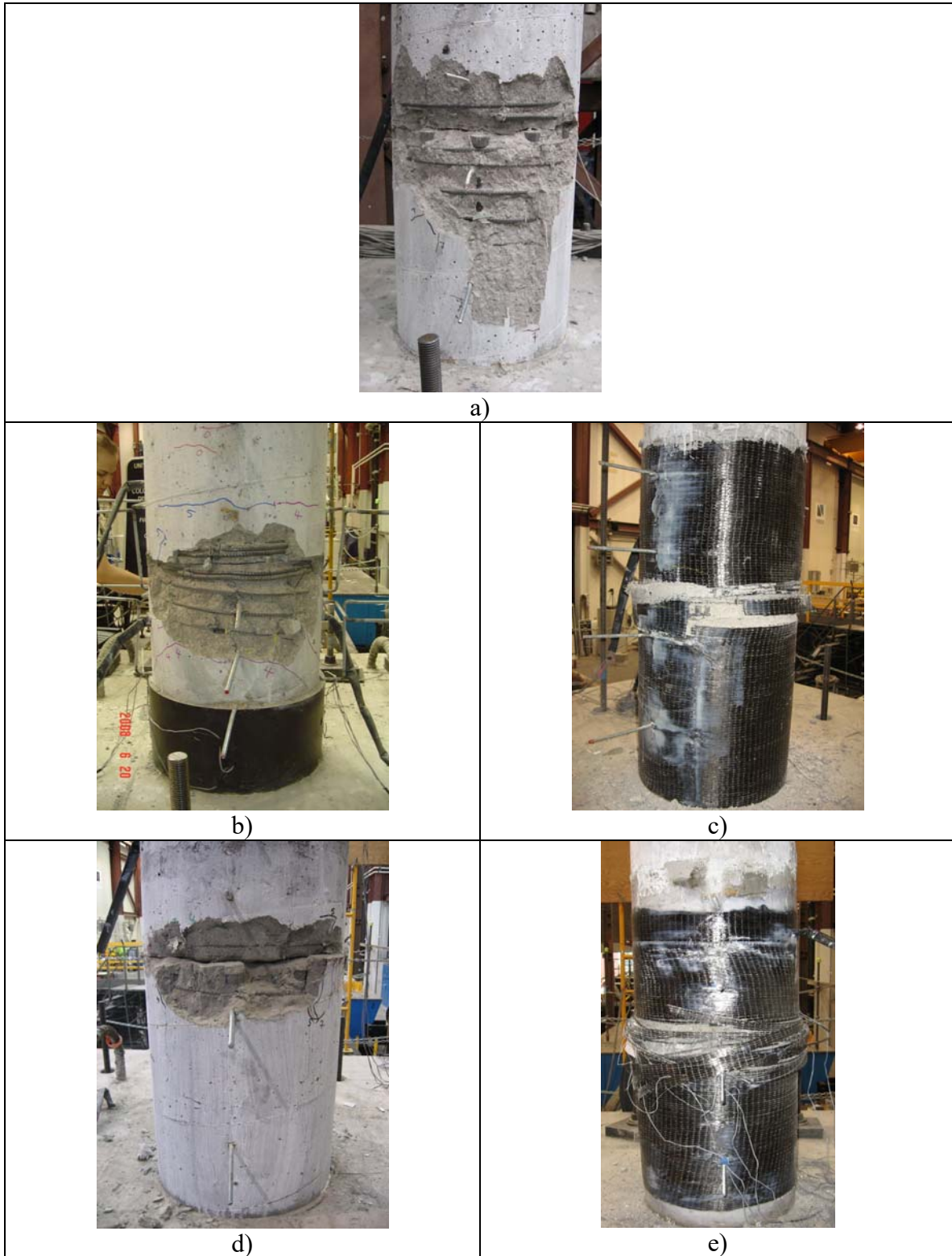
Fig. 4-3. Apparent Damage at 10% Drift for a) SC-2, b) SBR-1, c) SF-2, d) SE-2, e) SC-2R
