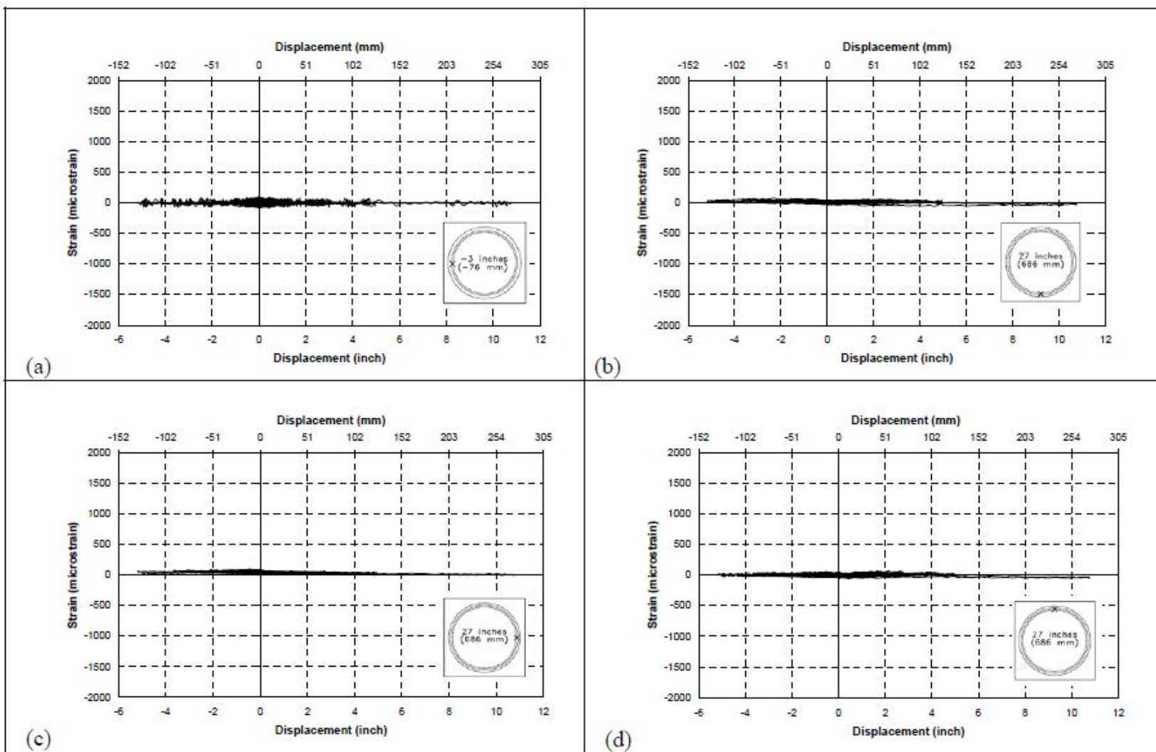
Fig. A-44. a) sg 54, b) sg 55, c) sg 56, d) sg 57 in SF-2
