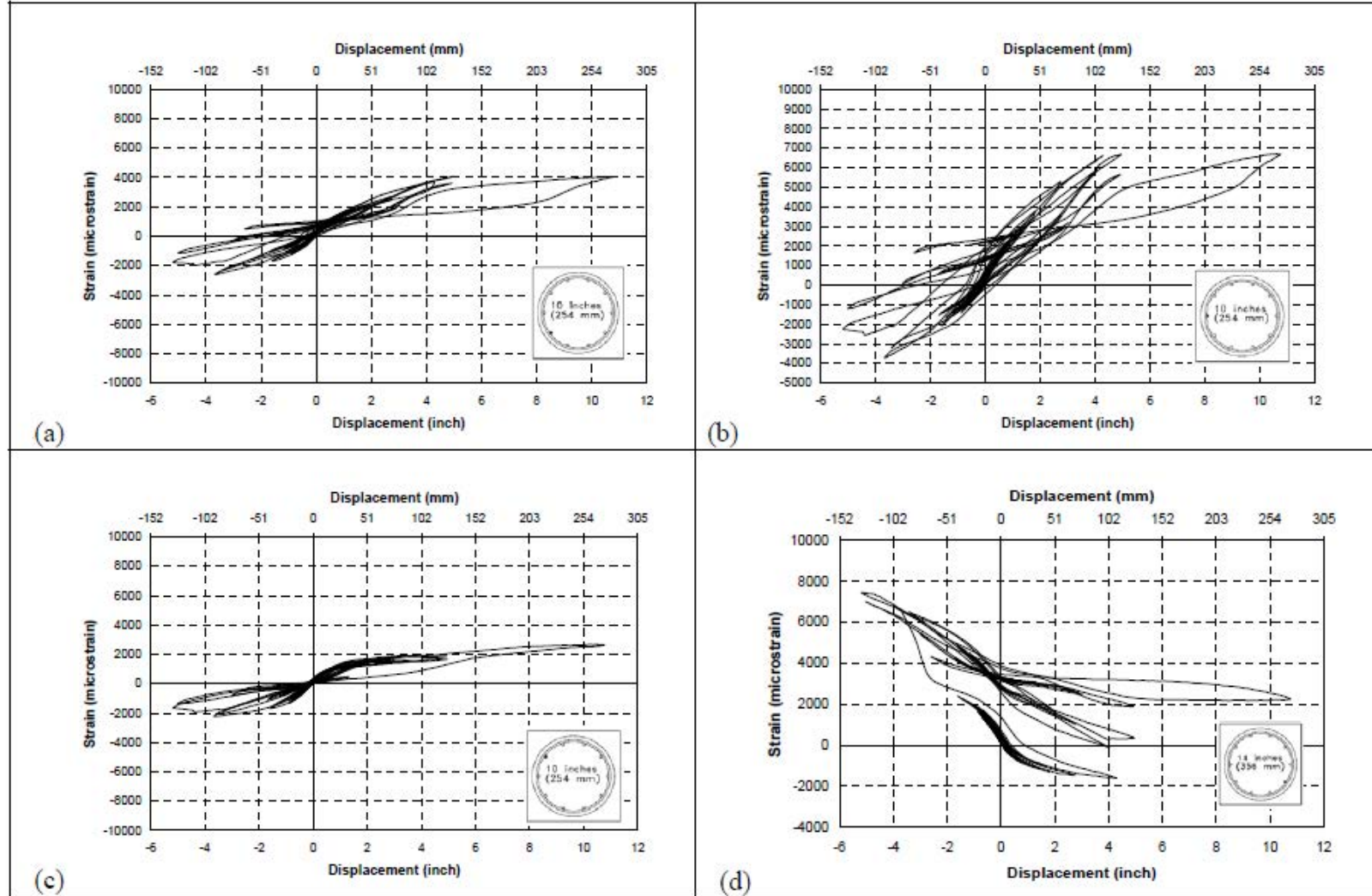
Fig. A-36. a) sg 26, b) sg 27, c) sg 28, d) sg 29 in SF-2
