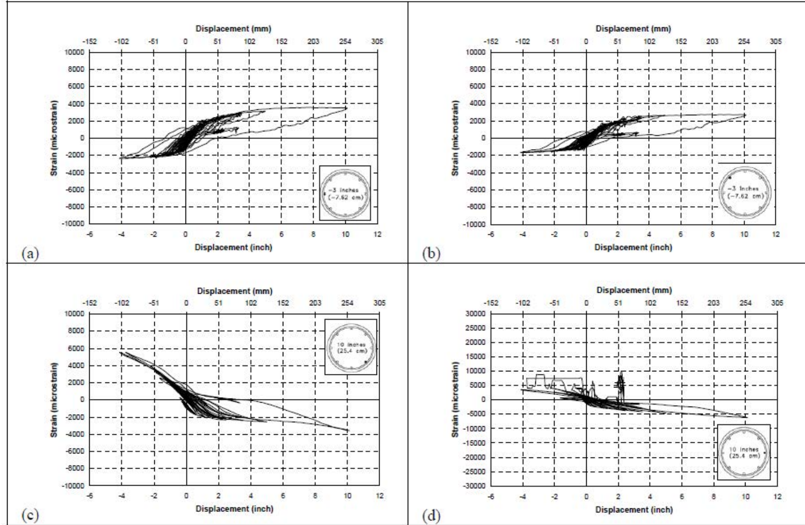
Fig. A-18. a) sg 9, b) sg 10, c) sg 11, d) sg 12 in SBR-1
