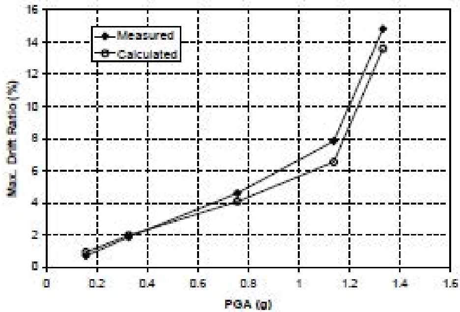
Fig. 6-37. Maximum Drift Ratio vs. PGA in SC-2R
