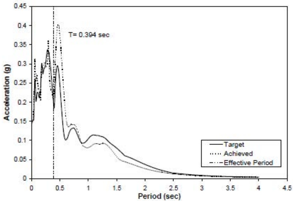
Fig. 3-31. Target vs. Achieved Ground Motion Spectra, Run-2 in SC-2
