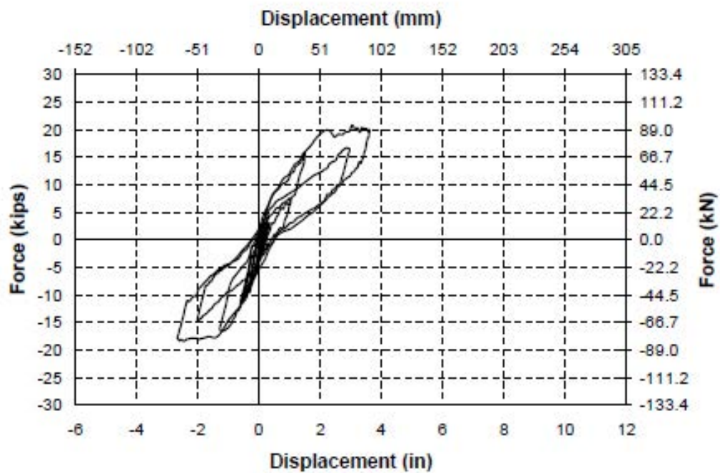
Fig. 3-122. Force-Displacement Hysteresis Curve for Run 5 in SE-2
