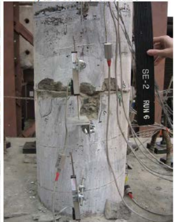
d) SE-2 Column, South, Run-6
