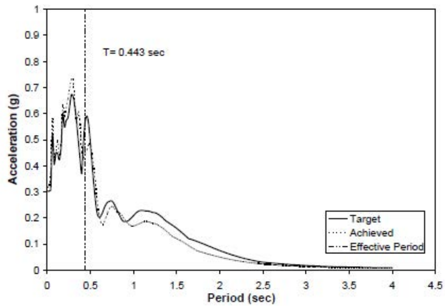
Fig. 3-178. Target vs. Achieved Ground Motion Spectra, Run-2 in SC-2R
