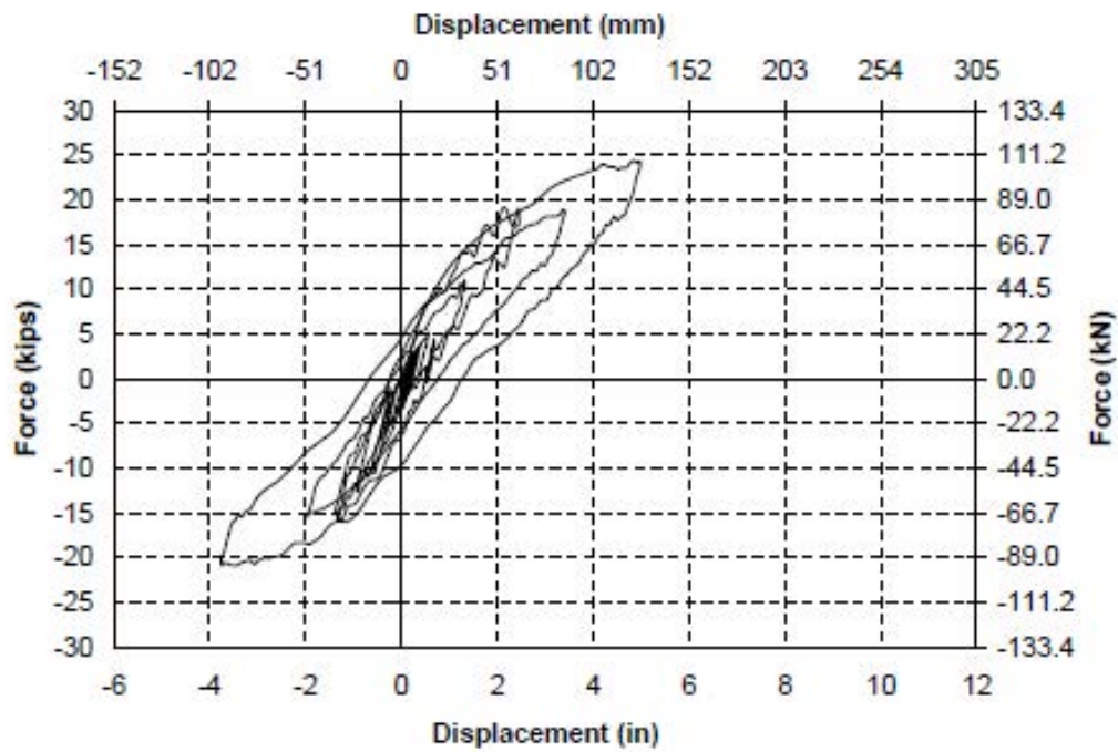
Fig. 3-47. Force-Displacement Hysteresis Curve for Run 6 in SBR-1
