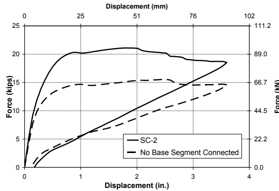
Fig. 17- Comparison between the Force-Displacement Cyclic Curves of SC-2 and Conventional Segmental Column
