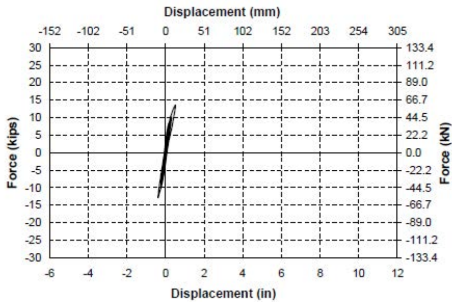
Fig. 3-155. Force-Displacement Hysteresis Curve for Run 1 in SC-2R
