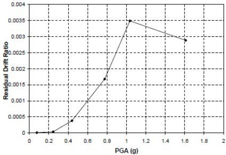
Fig. 3-238. Residual Drift Ratio vs. PGA in RC-ECC Column
