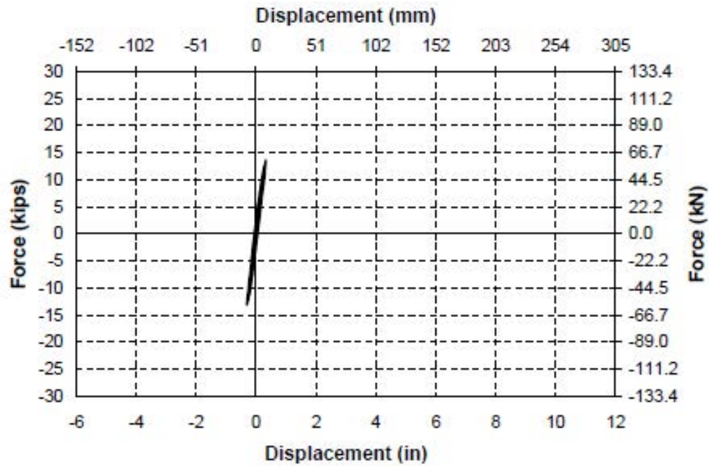
Fig. 3-7. Force-Displacement Hysteresis Curve for Run 2 in SC-2
