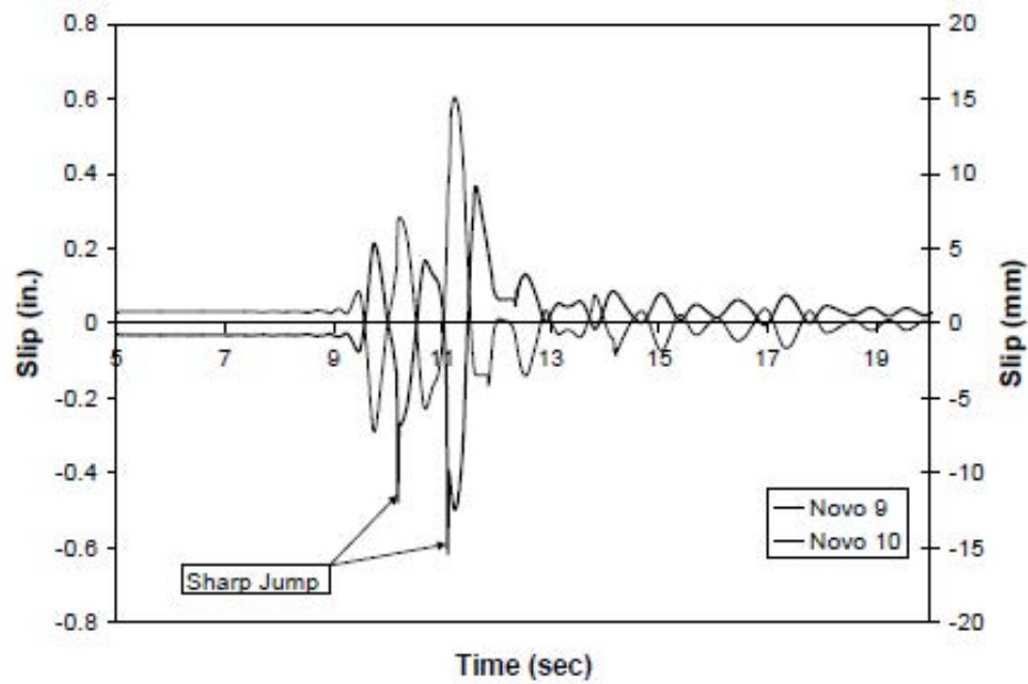
Fig. 3-192. Measured Sliding at Run 6 before Data Correction
