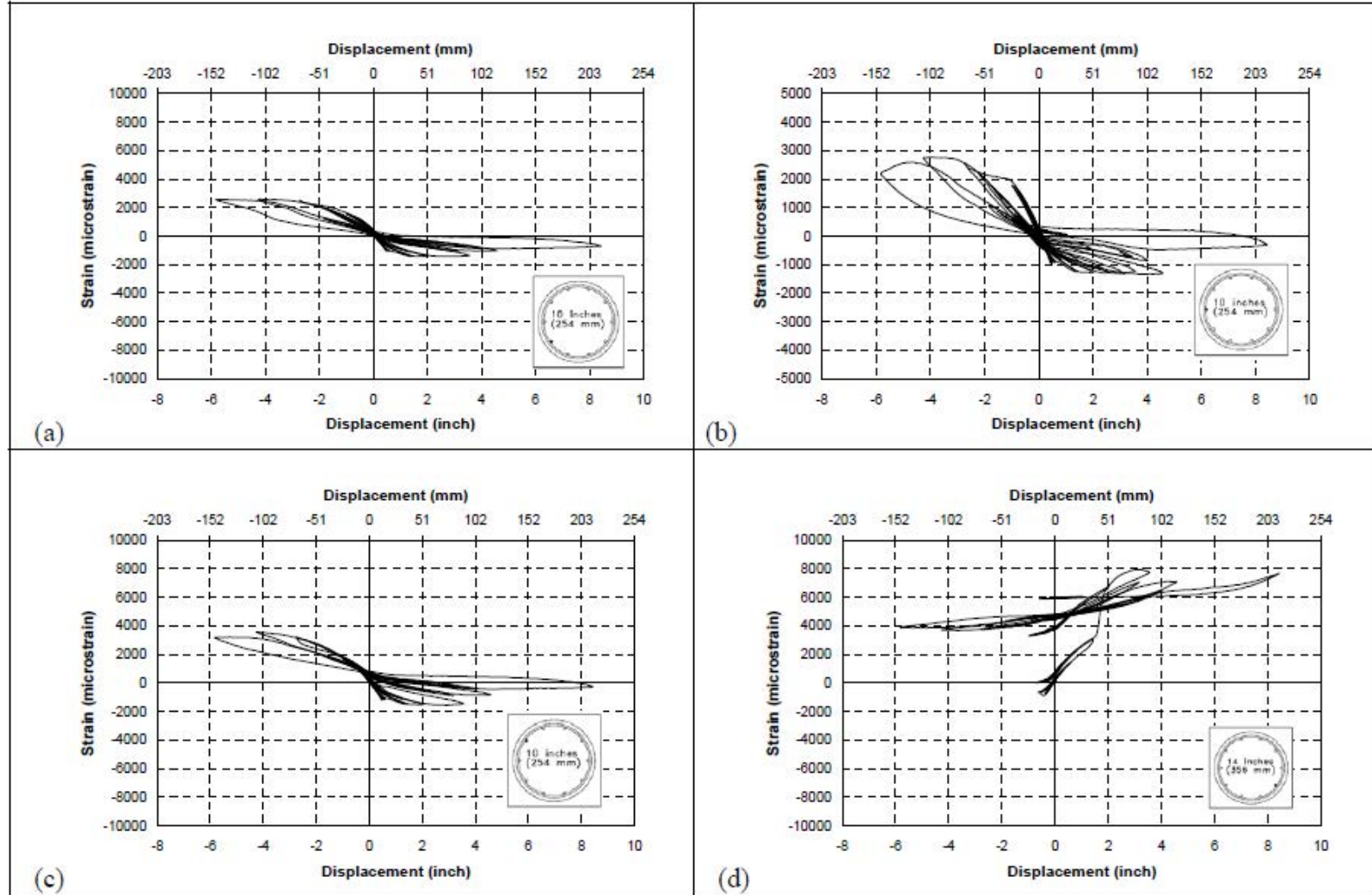
Fig. A-7. a) sg 26, b) sg 27, c) sg 28, d) sg 29 in SC-2
