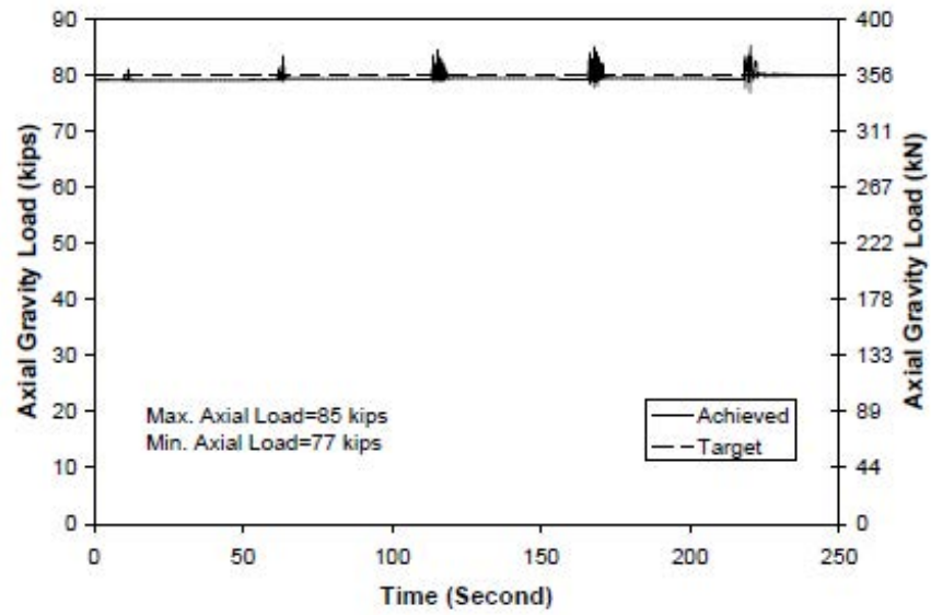
Fig. 3-173. Axial Gravity Load History on SC-2R
