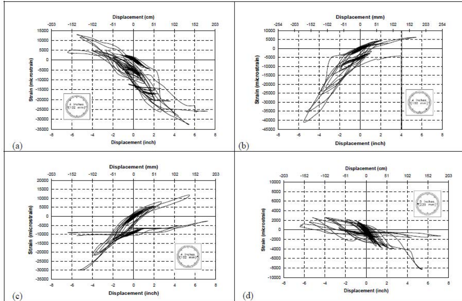
Fig. A-83. a) sg 13, b) sg 14, c) sg 15, d) sg 17 for RC-ECC Column in PEFB
