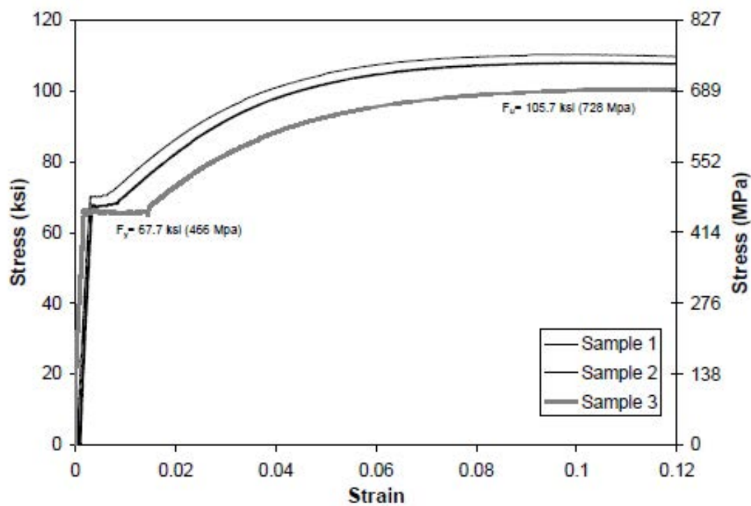
Fig. 2-81. Stress-Strain Behavior of #3 Bars in PEFB
