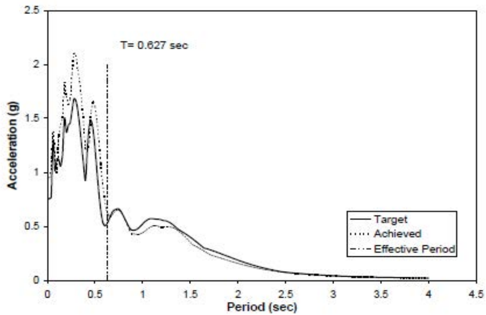
Fig. 3-148. Target vs. Achieved Ground Motion Spectra, Run-6 in SE-2
