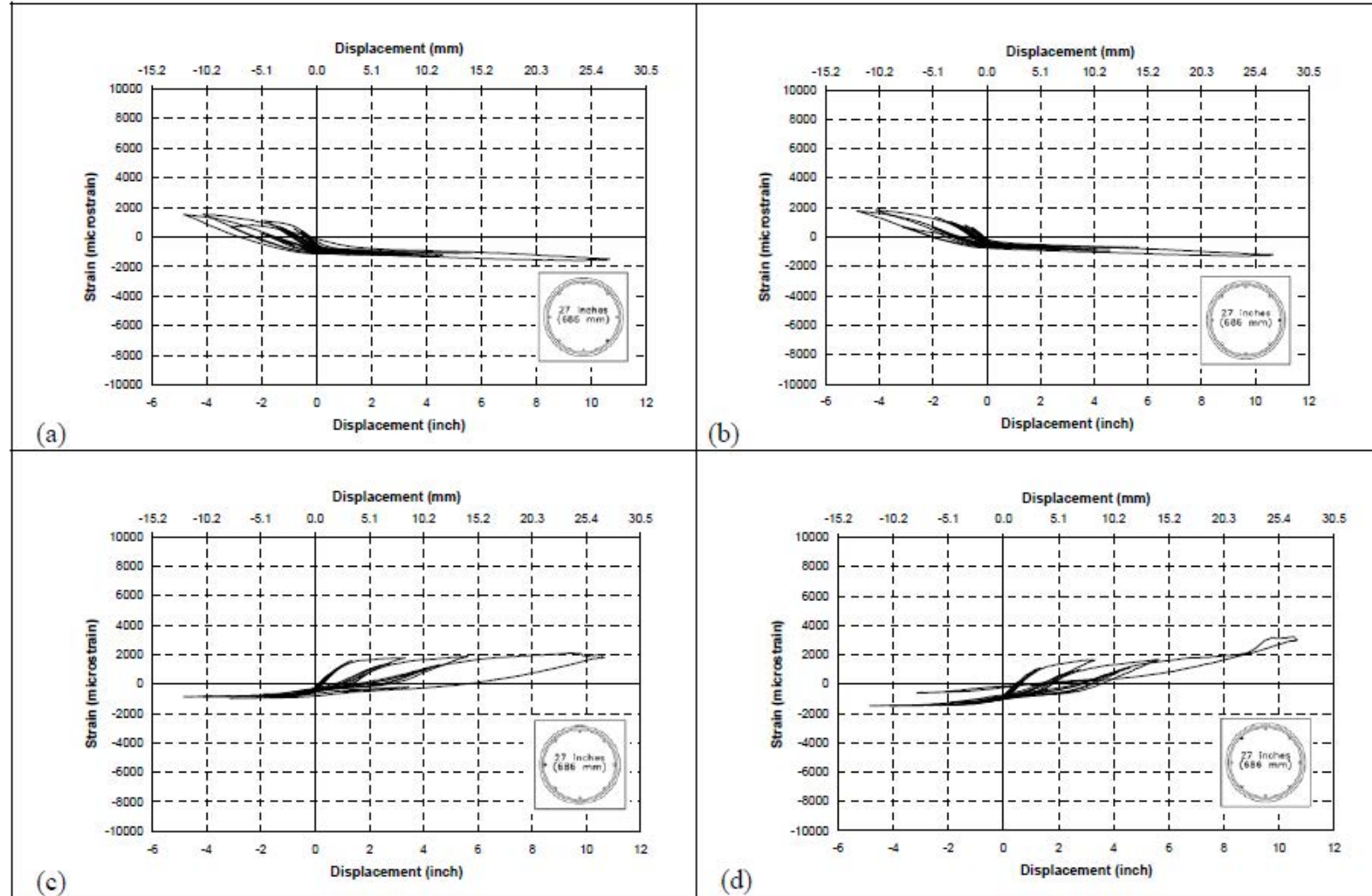
Fig. A-71. a) sg 35, b) sg 36, c) sg 37, d) sg 38 in SC-2R
