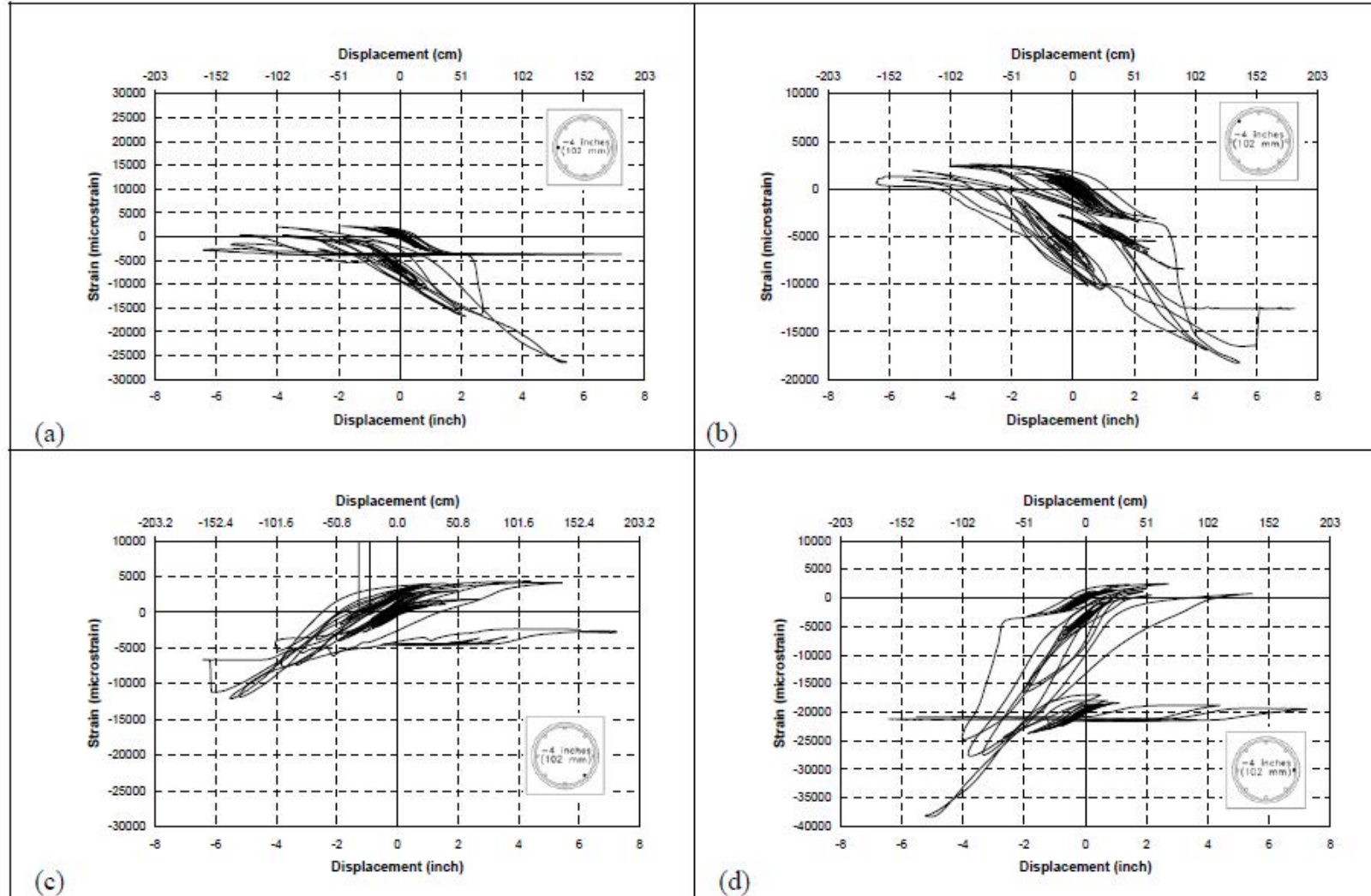
Fig. A-80. a) sg 1, b) sg 2, c) sg 3, d) sg 4 for RC-ECC Column in PEFB
