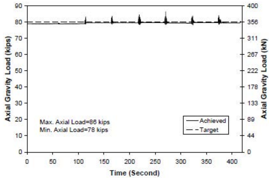
Fig. 3-139. Axial Gravity Load History on SE-2
