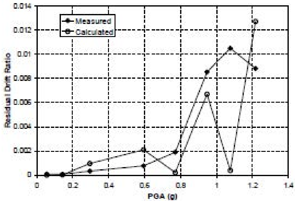
Fig. 6-36. Residual Drift Ratio vs. PGA in SE-2
