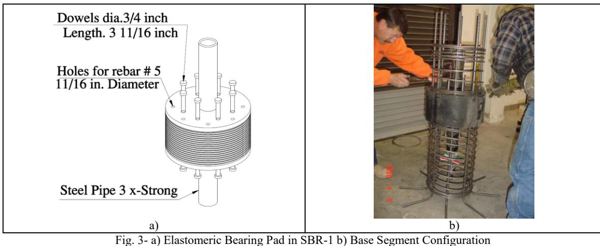
Fig. 3- a) Elastomeric Bearing Pad in SBR-1 b) Base Segment Configuration
