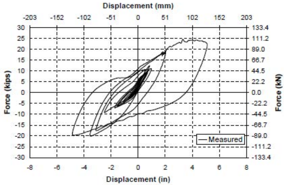
Fig. 3-211. Force-Displacement Hysteresis Curve for Run 5 in RC-ECC Column
