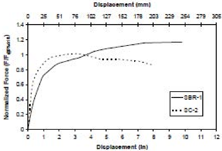
Fig. 4-4. Comparison of Normalized Backbone Curves in SBR-1 and SC-2
