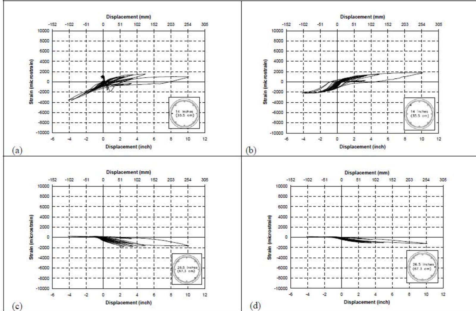
Fig. A-21. a) sg 21, b) sg 22, c) sg 23, d) sg 24 in SBR-1
