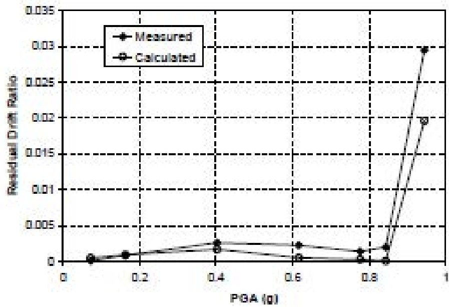
Fig. 6-32. Residual Drift Ratio vs. PGA in SBR-1
