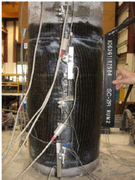
SC-2R Column, North, Run-2
