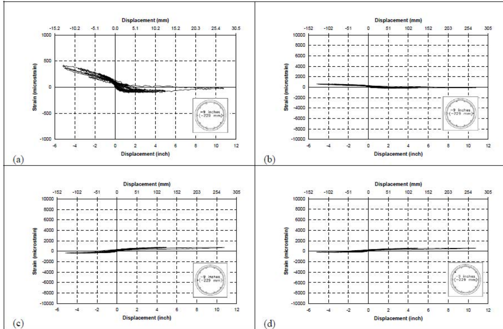
Fig. A-30. a) sg 1, b) sg 2, c) sg 3, d) sg 4 in SF-2
