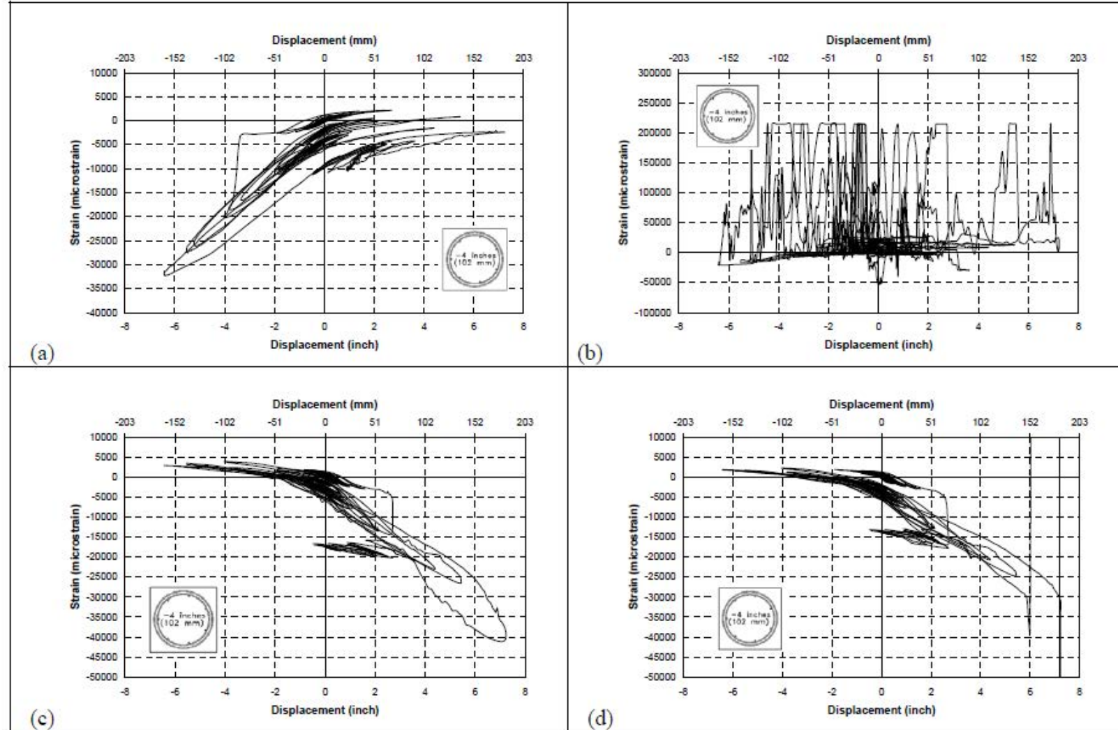
Fig. A-88. a) sg 37, b) 38, c) sg 39, d) sg 40 for FRP Column in PEFB
