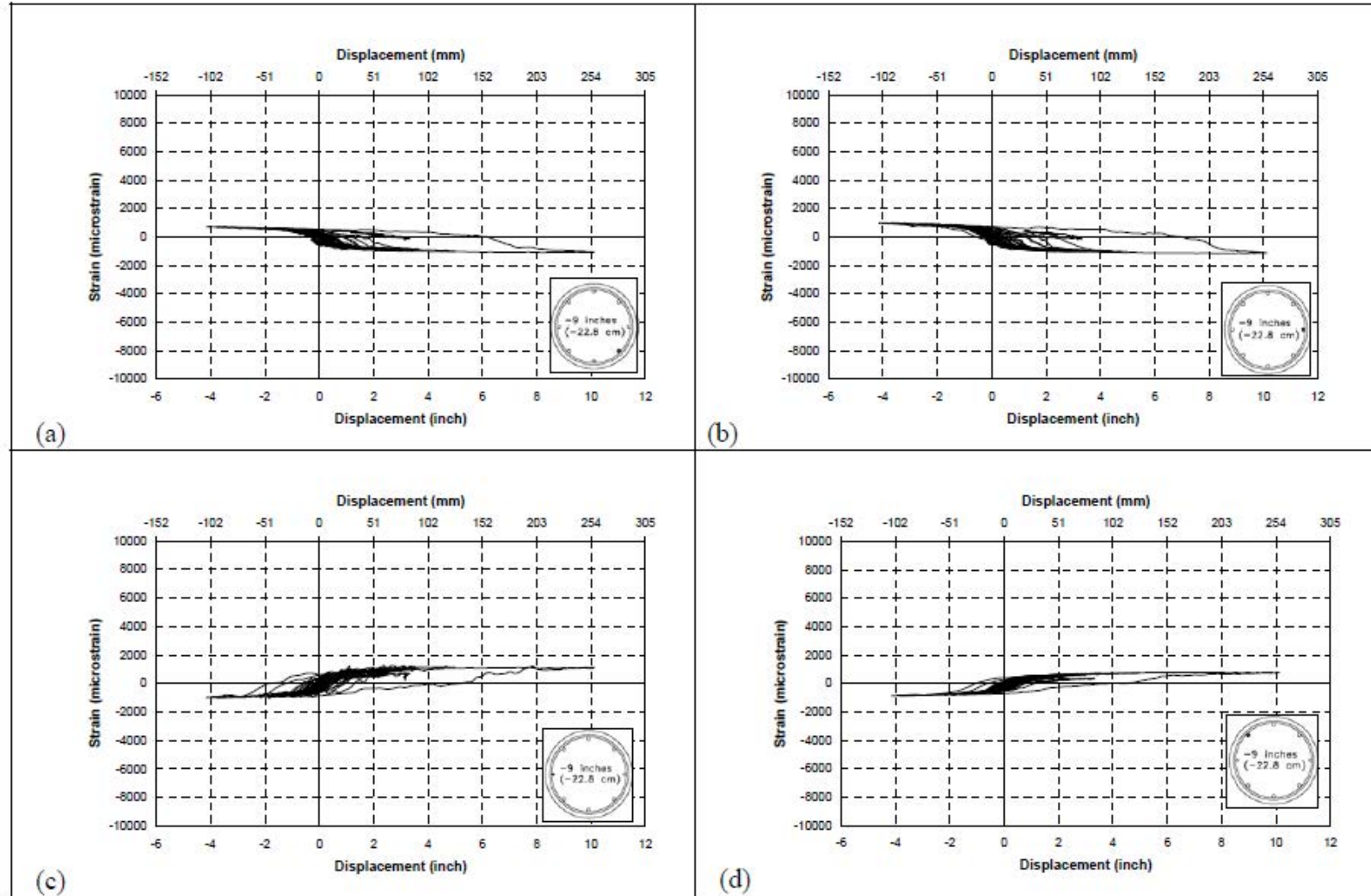
Fig. A-16. a) sg 1, b) sg 2, c) sg 3, d) sg 4 in SBR-1
