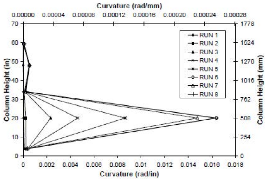
Fig. 3-133. Curvature Profile for SE-2
