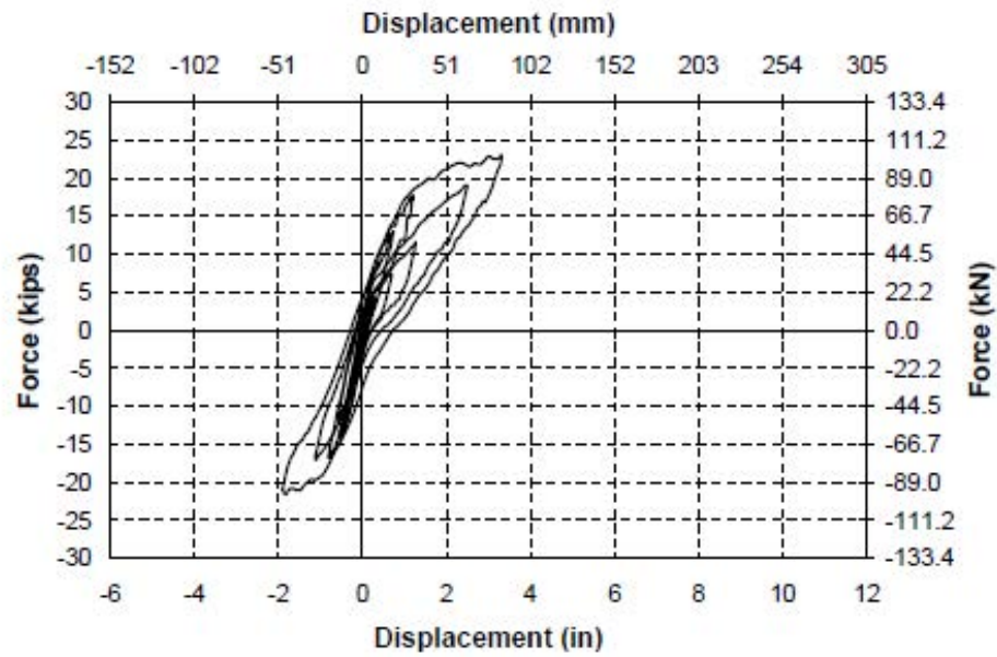
Fig. 3-157. Force-Displacement Hysteresis Curve for Run 3 in SC-2R
