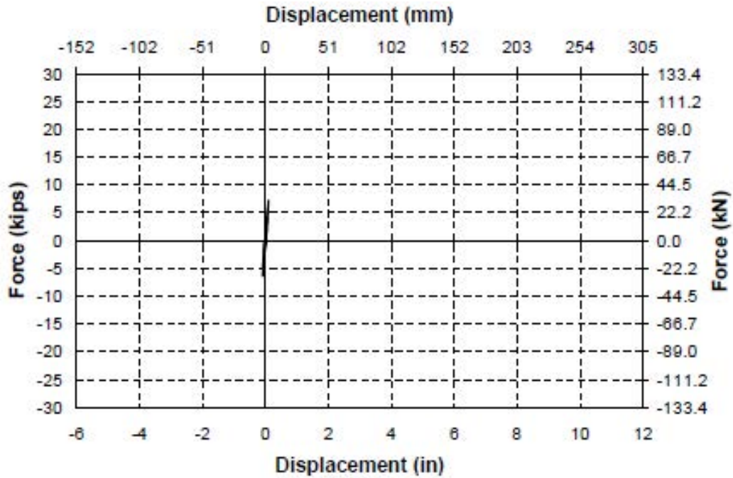
Fig. 3-79. Accumulated Force-Displacement Hysteresis Curve for SF-2
