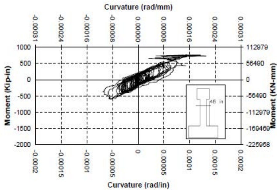
Fig. 3-165. Accumulated Moment Curvature at the Fourth Level in SC-2R
