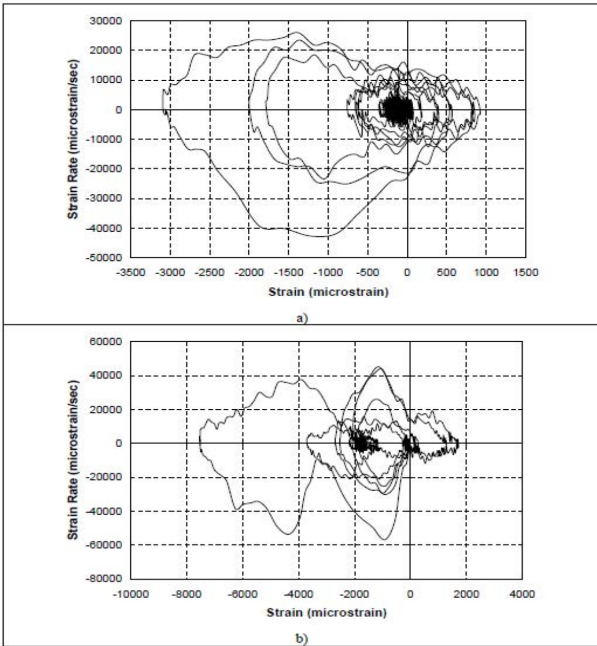
Fig. 3-176. Strain Rate vs. Strain in SC-2R a) Gauge 15, Run 2 b) Gauge 12, Run 4
