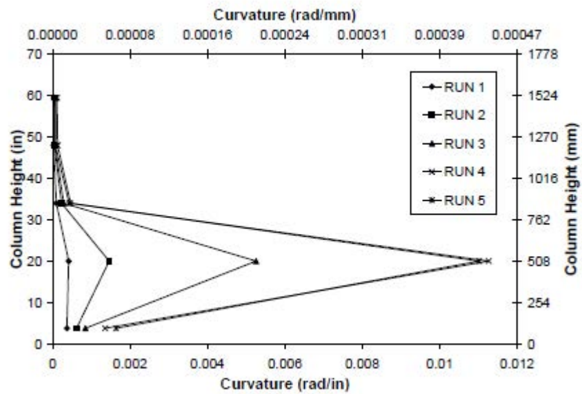
Fig. 3-167. Curvature Profile for SC-2R
