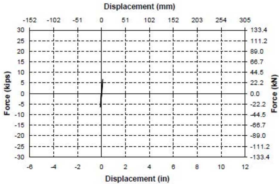
Fig. 3-118. Force-Displacement Hysteresis Curve for Run 1 in SE-2
