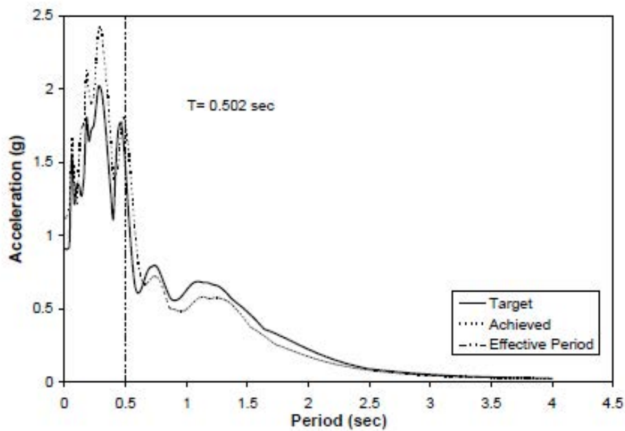
Fig. 3-180. Target vs. Achieved Ground Motion Spectra, Run-4 in SC-2R
