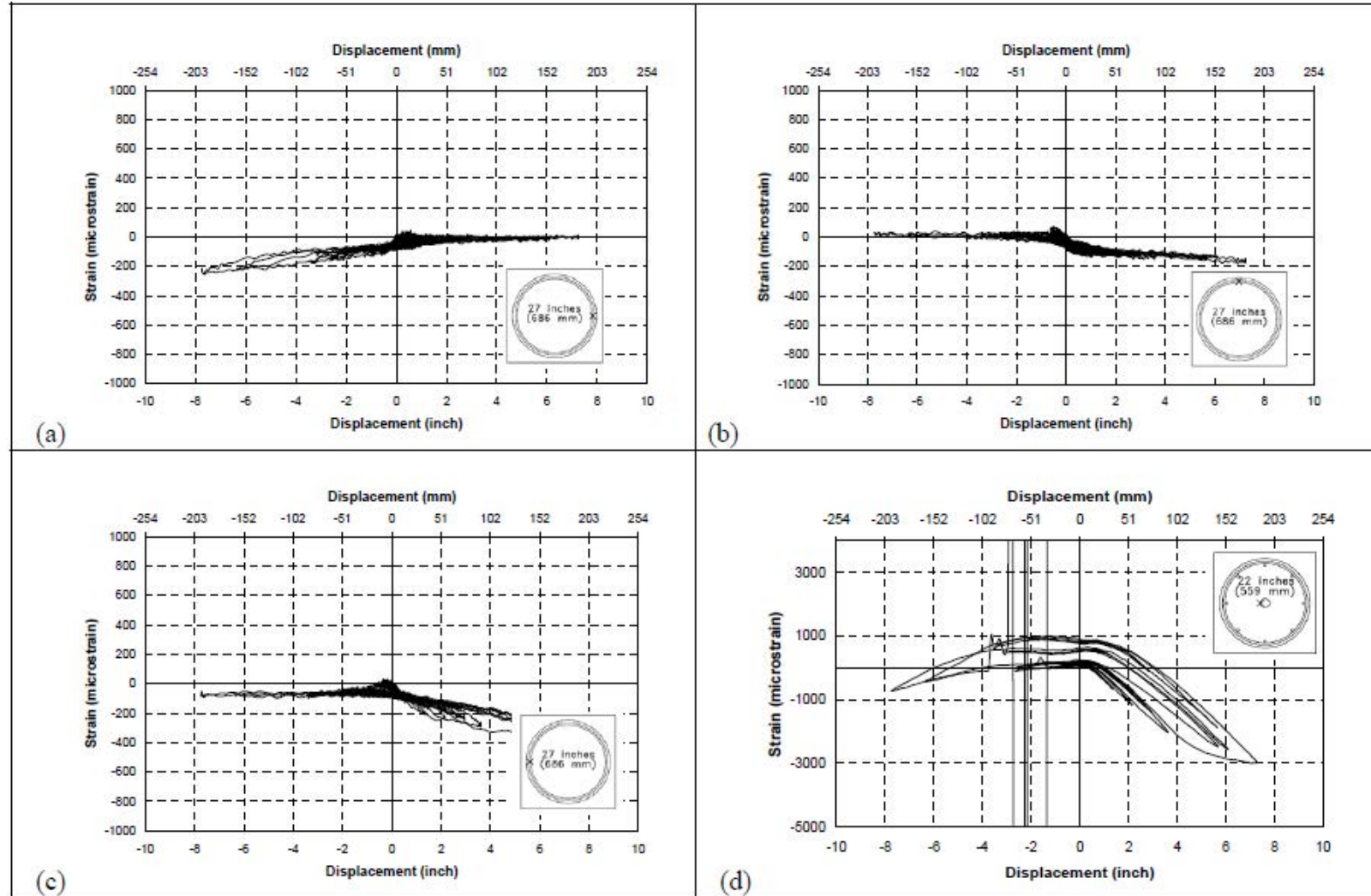
Fig. A-61. a) sg 6 b) sg 57, c) sg 58, d) sg 59 in SE-2
