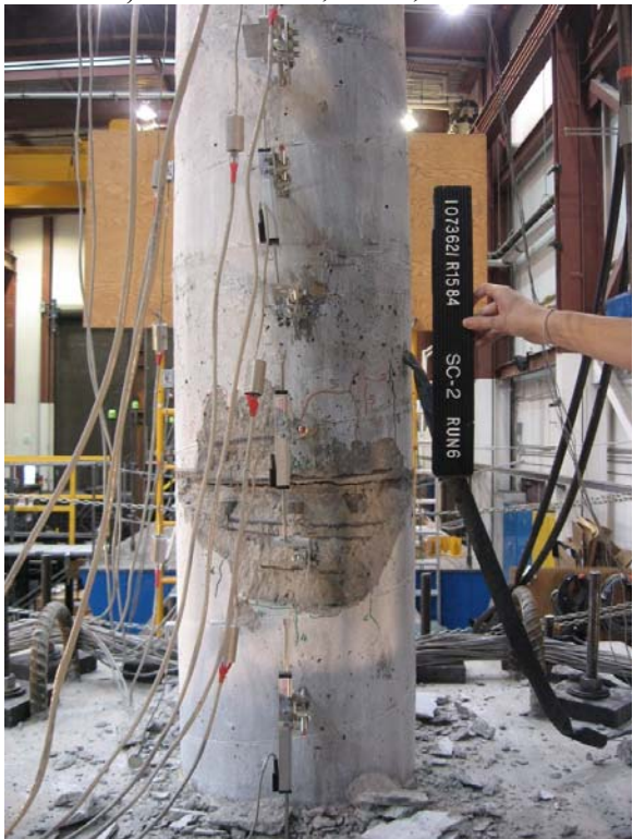
c) SC-2 Column, North, Run-6
