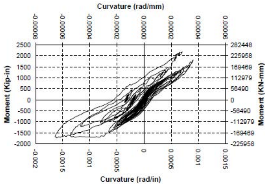
Fig. 3-162. Accumulated Moment Curvature at the First Level in SC-2R
