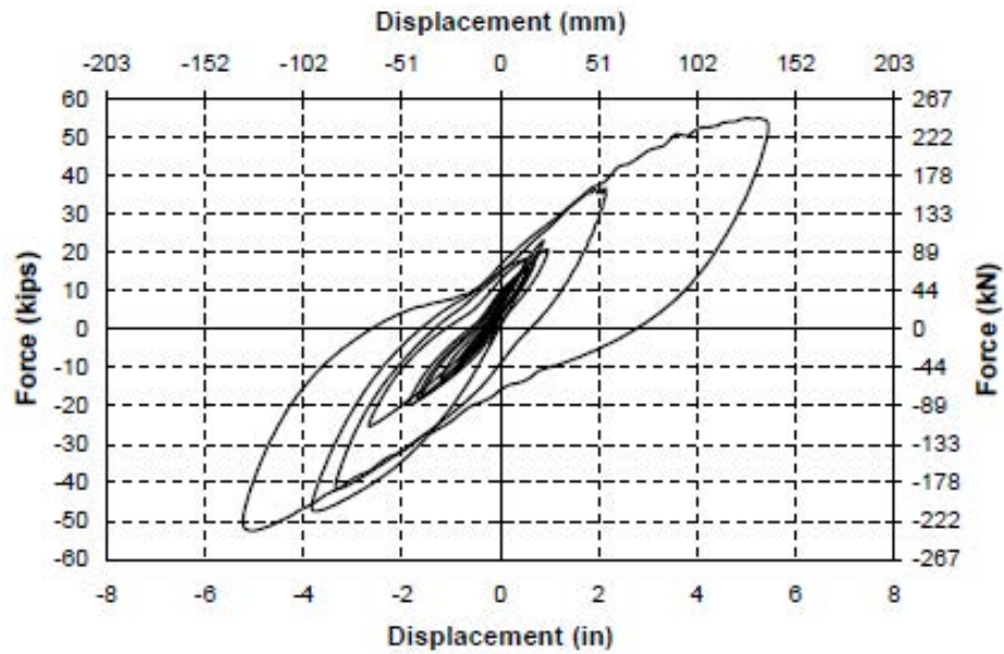
Fig. 3-203. Force-Displacement Hysteresis Curve for Run 5 in PEFB Bent
