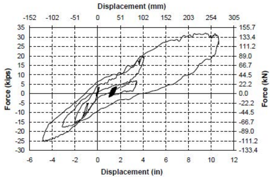
Fig. 3-159. Force-Displacement Hysteresis Curve for Run 5 in SC-2R
