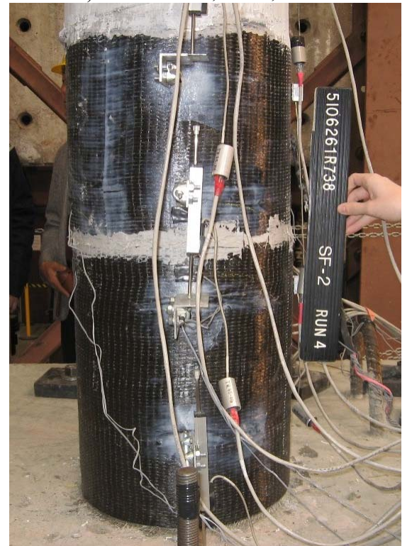
d) SF-2 Column, South, Run-4
