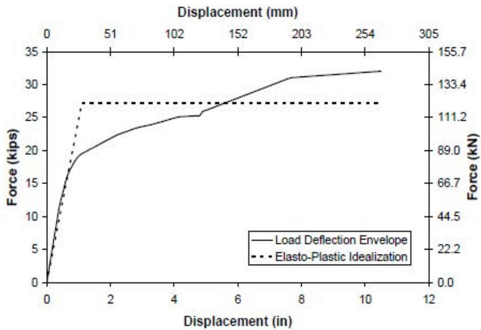
Fig. 3-160. Backbone Curve of SC-2R
