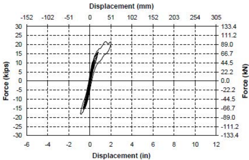
Fig. 3-9. Force-Displacement Hysteresis Curve for Run 4 in SC-2
