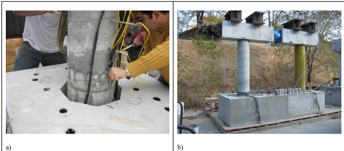
Fig. 8- a) Inserting the Columns in to the Footing, b) PEFB after Assembly
