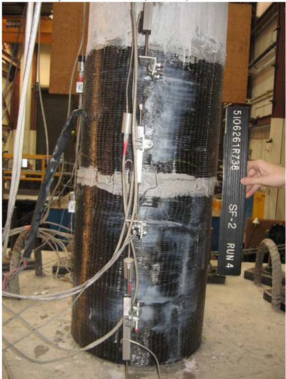
c) SF-2 Column, North, Run-4
