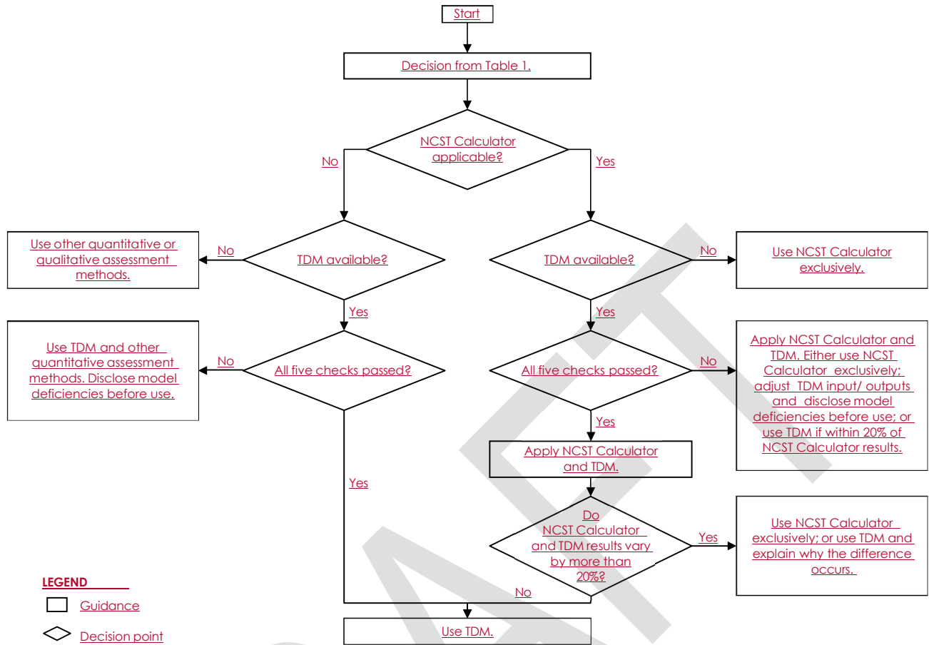
Figure 5-5. A detailed assessment method selection flow chart.
