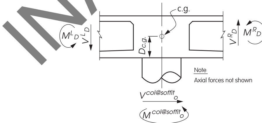
Figure 4 - Longitudinal Free Body Diagram of Joint Forces
