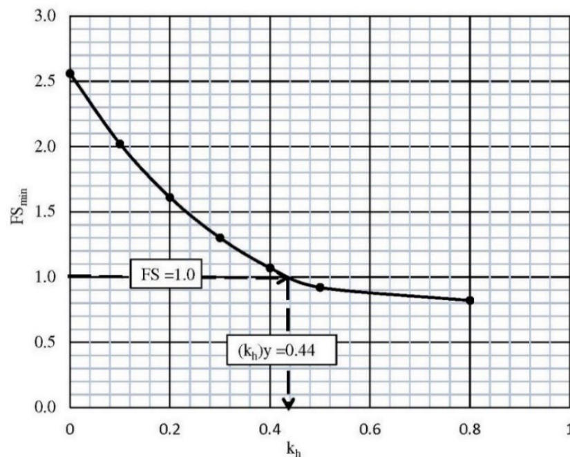
Figure 5. Determination of the Coefficient of Yield Acceleration
