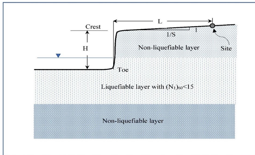
Figure 10. Model Parameters (Modified after Bartlett and Youd, 1992)
