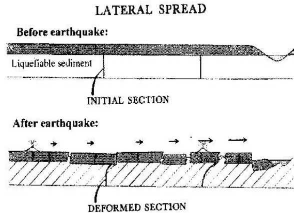
Figure 9. Liquefaction-Induced Lateral Spread (Youd, 2018)
