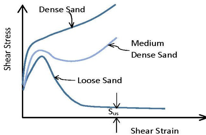
Figure 1: Undrained Shear Stress-Strain Behavior of Saturated Cohesionless Soils Under Monotonic Loading (Schematic)
