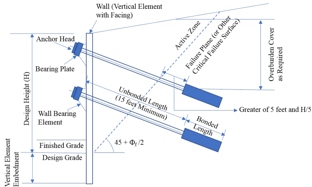
Figure 1: Ground Anchor ERS Components and Dimensions (Modified after AASHTO LRFD BDS)
