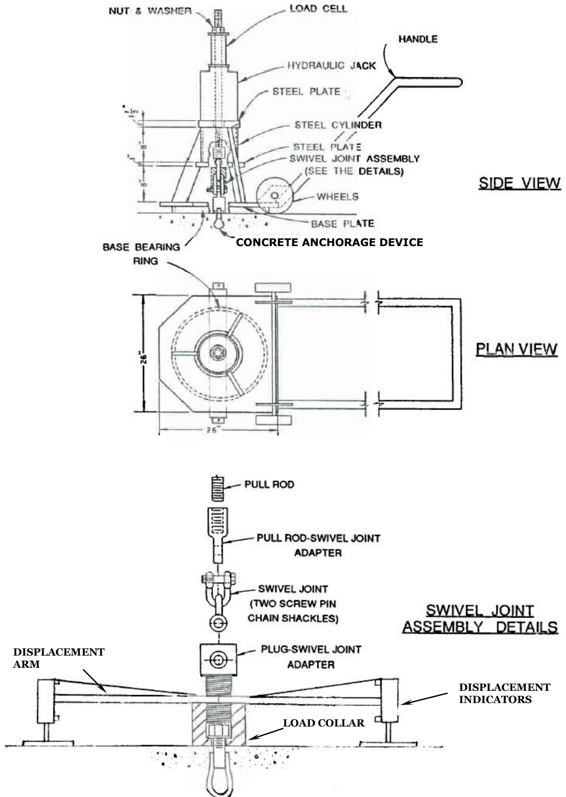
Figure 1. SCHEMATIC OF A TENSION TESTING APPARATUS
