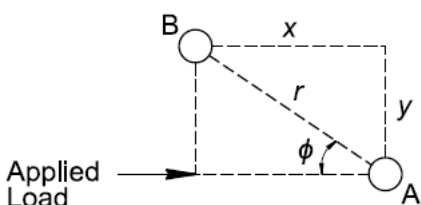
Figure 10.7.2.4-4 Skew Effect (After Reese, et al.(2006))
