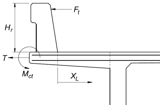
Figure A13.4.2-1 – Force Effects on Deck Overhang Due to Railing Collision Force
