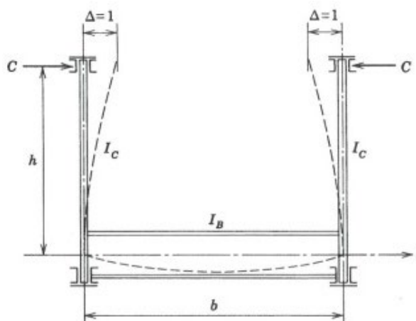
Figure C4.6.2.5-1A—U-Frame
