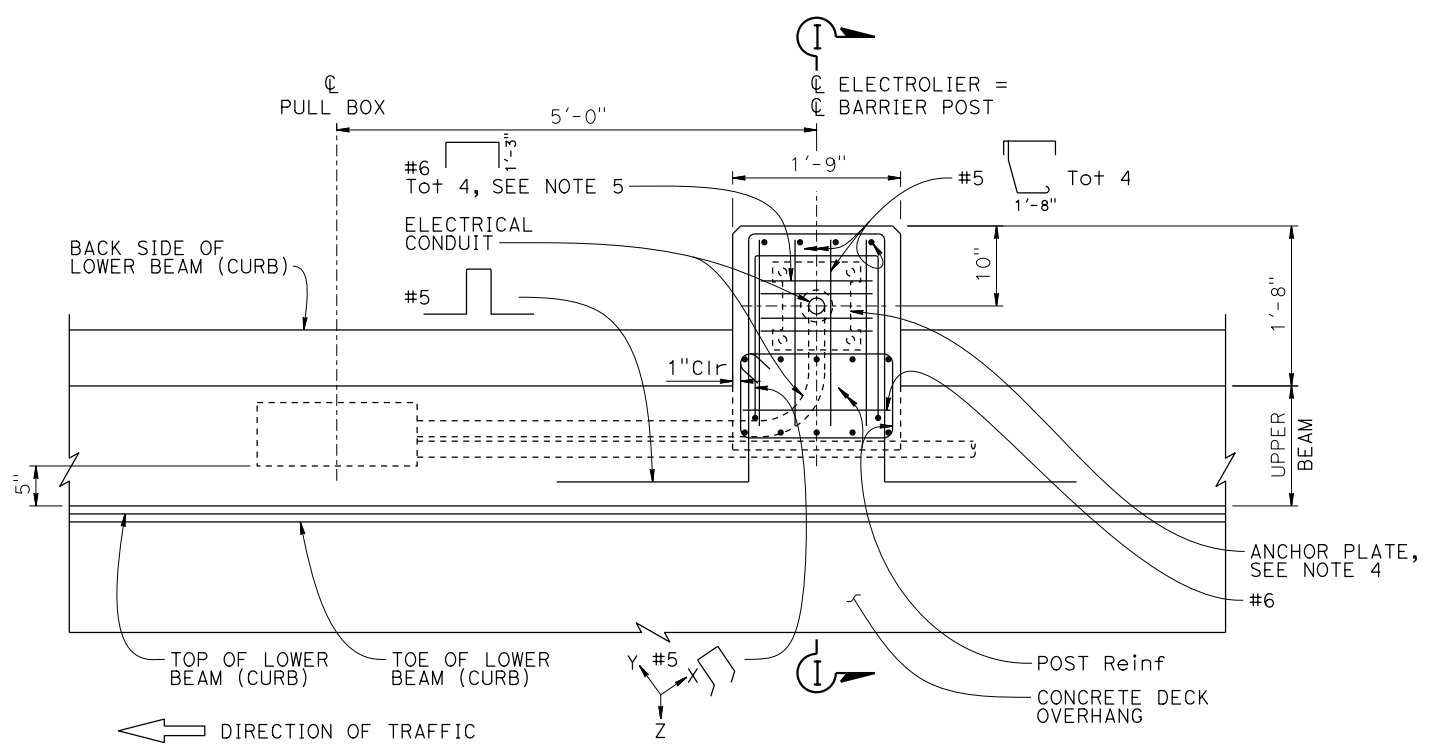
PLAN See Note 1.
