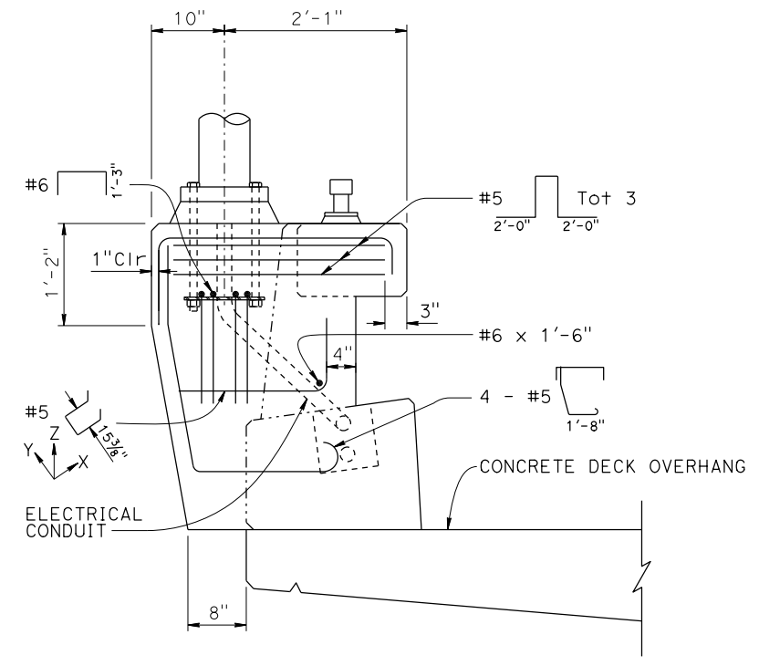
SECTION I-I See Note 4.
