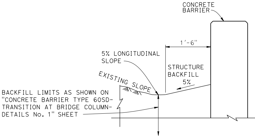
BACKFILL DETAIL
