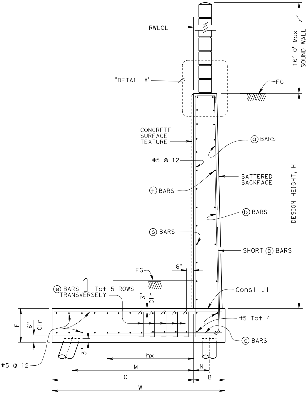
TYPICAL SECTION
