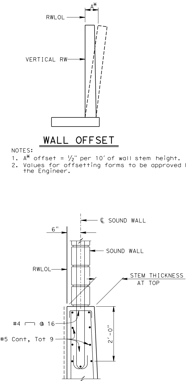
DETAIL A
