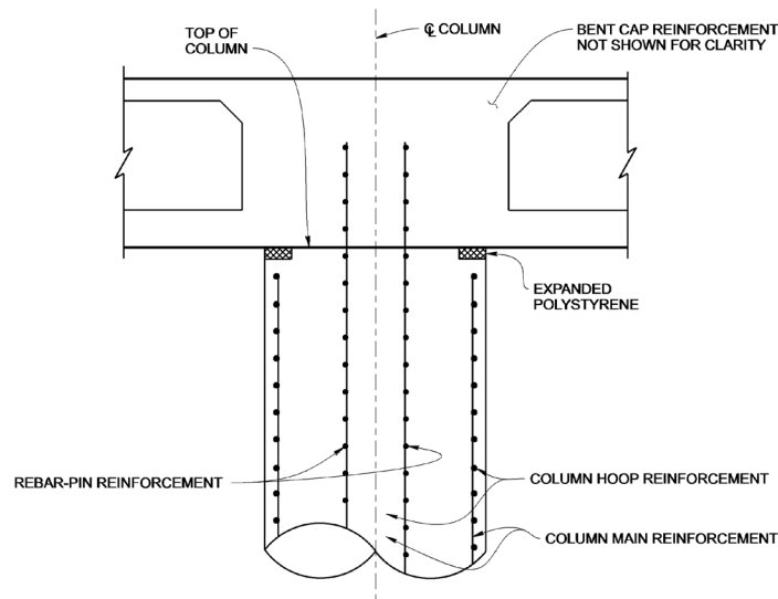
Figure 5.5.4.1-2 Rebar-Pin Details
