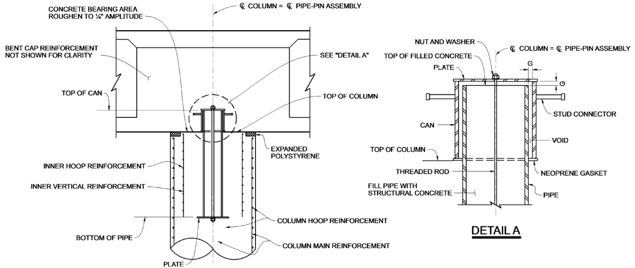
Figure 5.5.4.1-1 Pipe-Pin Details
