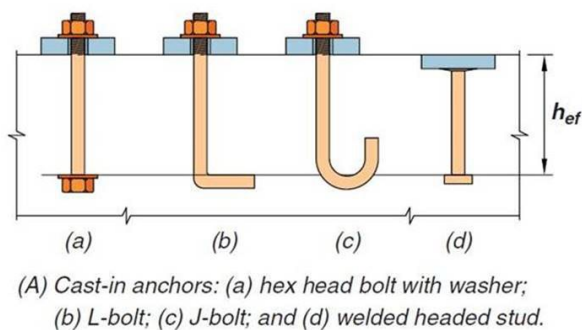
Figure 5.51.4-1 Cast-in Anchor Types (ACI 318-14, Figure R2.1)
