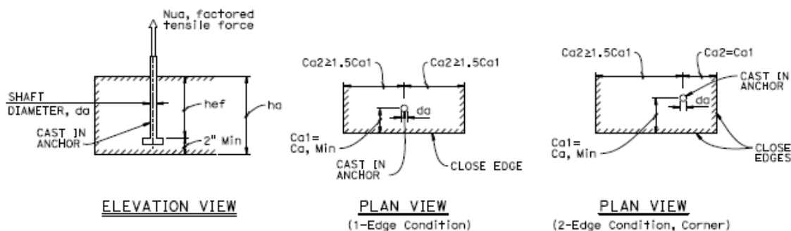
Figure 5.51.5.2-1 Tension
