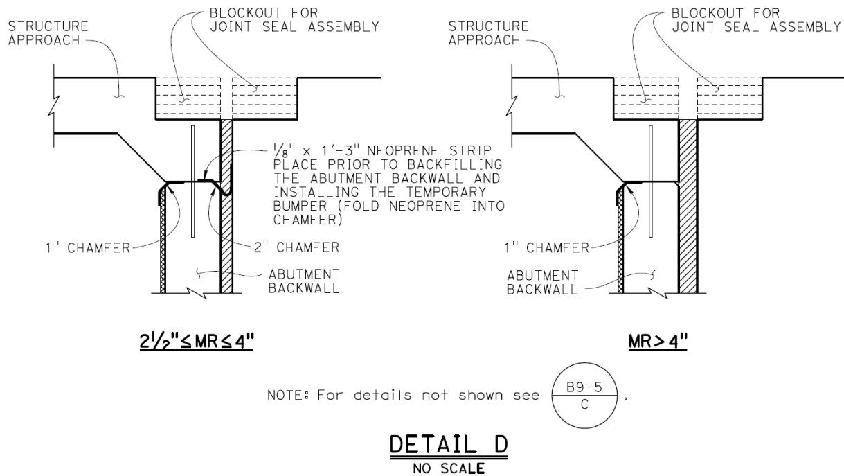
Figure 6.7.3 Joint Seal Protection Detail (MR > 2 1/2")
