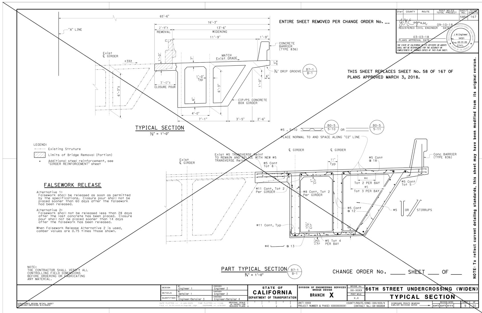
Figure 1A.G.7 Deleted Sheet Detailing Example
