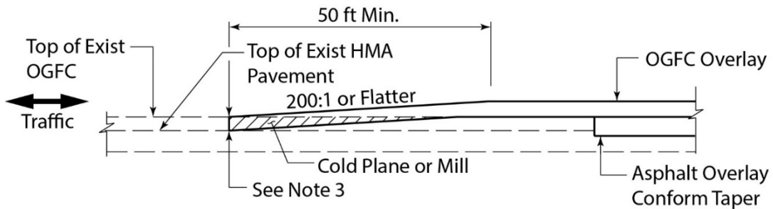
Transverse OGFC Taper to Existing OGFC Pavement
