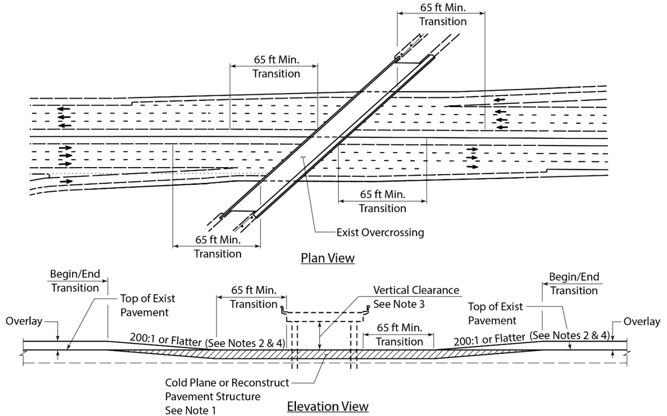
Figure 671.3C Transition Taper Underneath Overcrossing/Bridge
