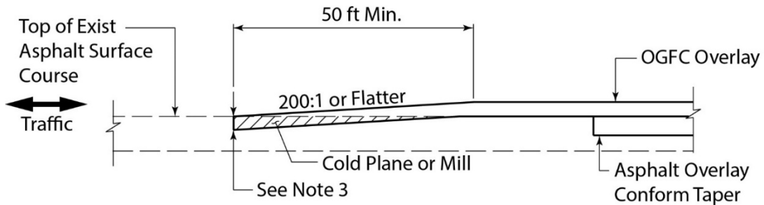
Transverse OGFC Taper to Existing Asphalt Pavement
