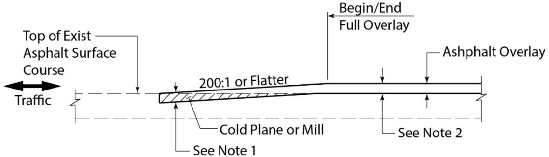
Transverse Asphalt Taper to Existing Asphalt Pavement
