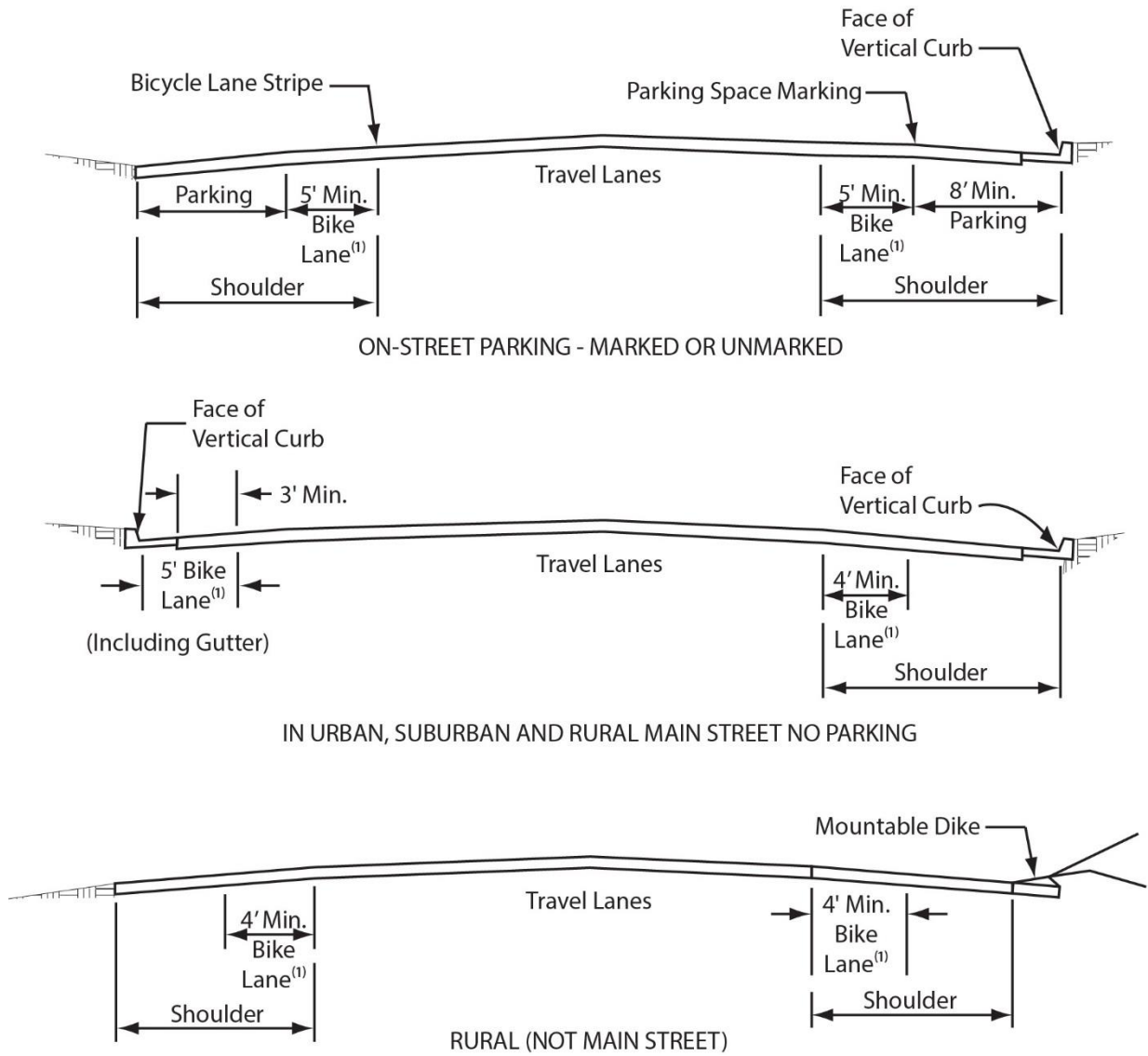
Figure 301.2A Typical Class II Bikeway (Bike Lane) Cross Sections
