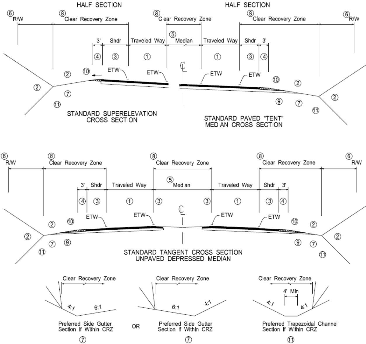
Figure 307.4A Geometric Cross Sections for Freeways and Expressways
