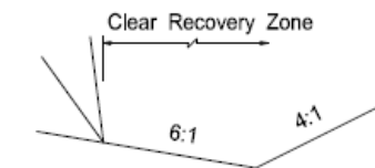
Preferred Side Gutter Section If Within CRZ
