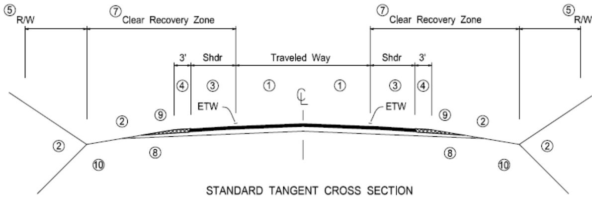
STANDARD TANGENT CROSS SECTION
