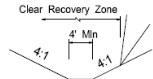
Preferred Trapezoidal Channel Section if Within CRZ
