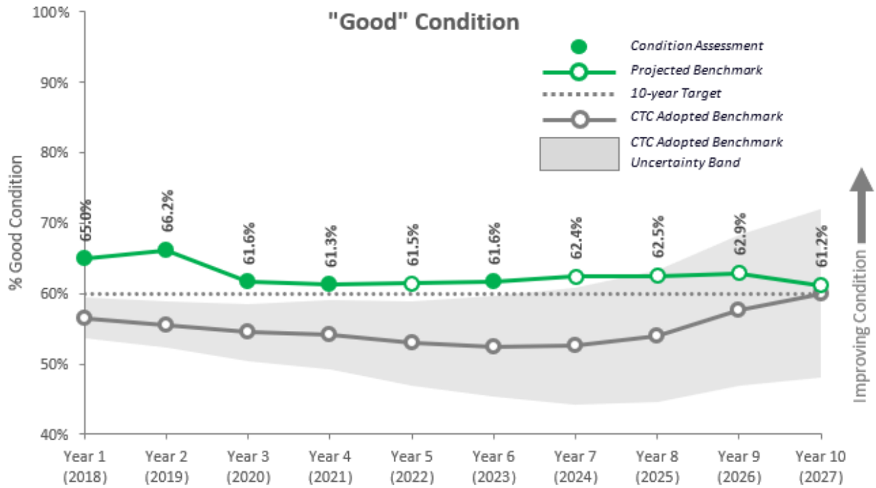
Figure 1 - Pavement Class I, Good
