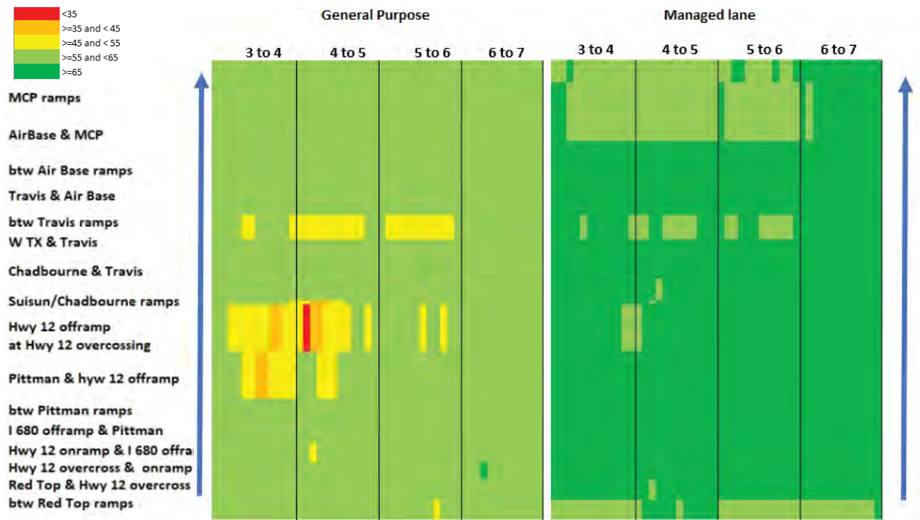
Figure 1-16: Future Build Scenario 1 Weekday Eastbound Speed – Fairfield PM Peak Period
