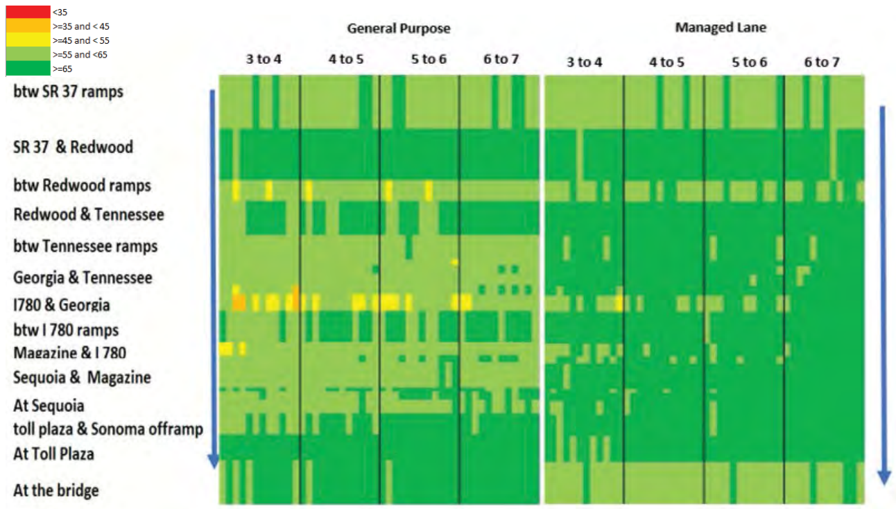
Figure 1-21: Future Build Scenario 1 Weekday Westbound Speed – Vallejo PM Peak Period
