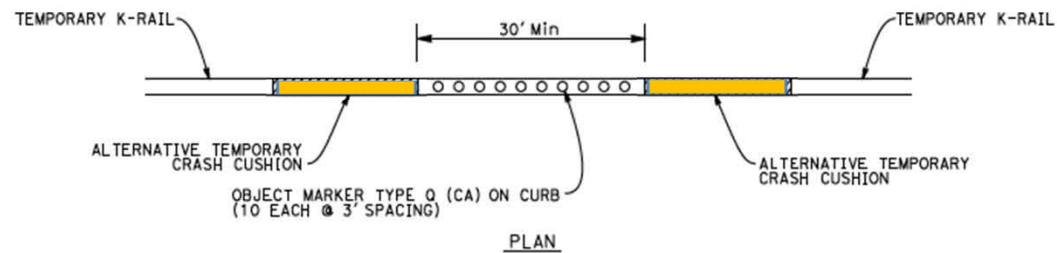
TEMPORARY EMERGENCY MEDIAN OPENING
