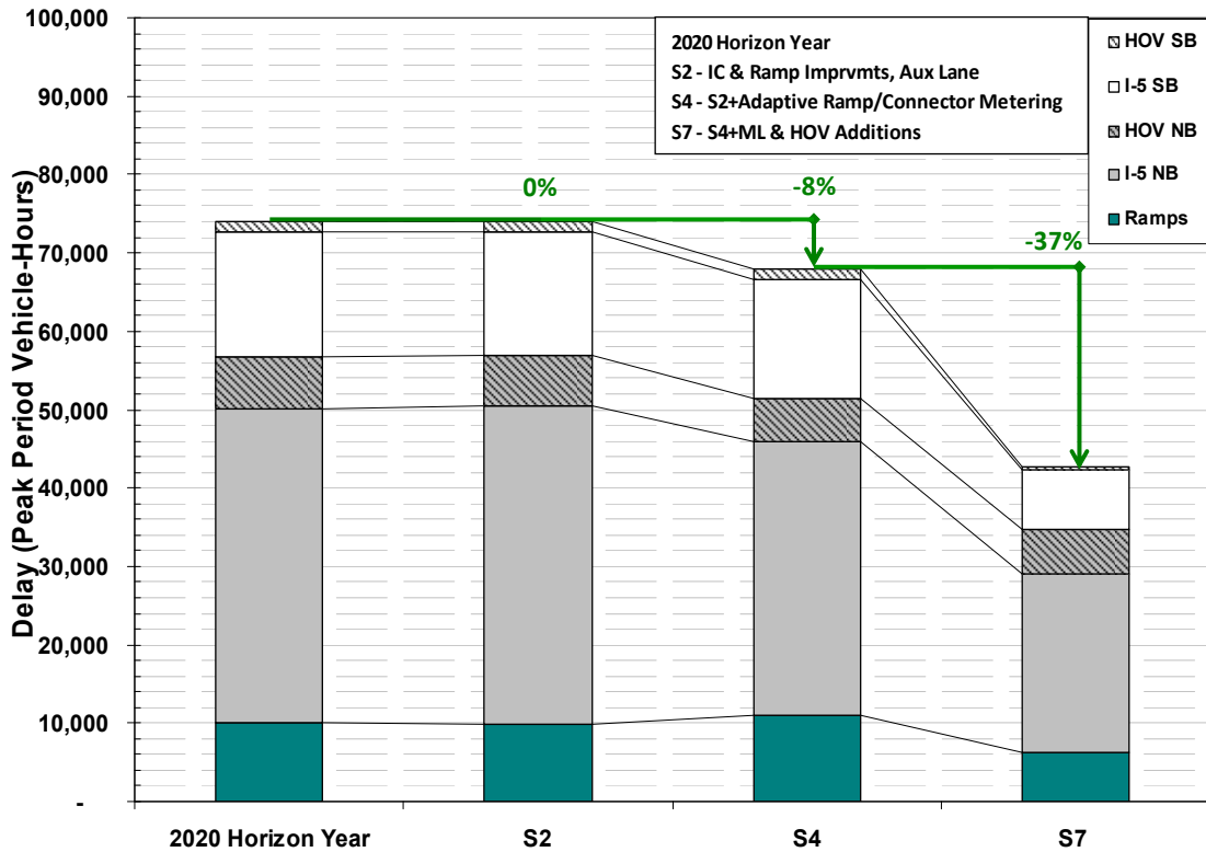
Exhibit ES-30: 2020 PM Peak Micro-Simulation Delay by Scenario
