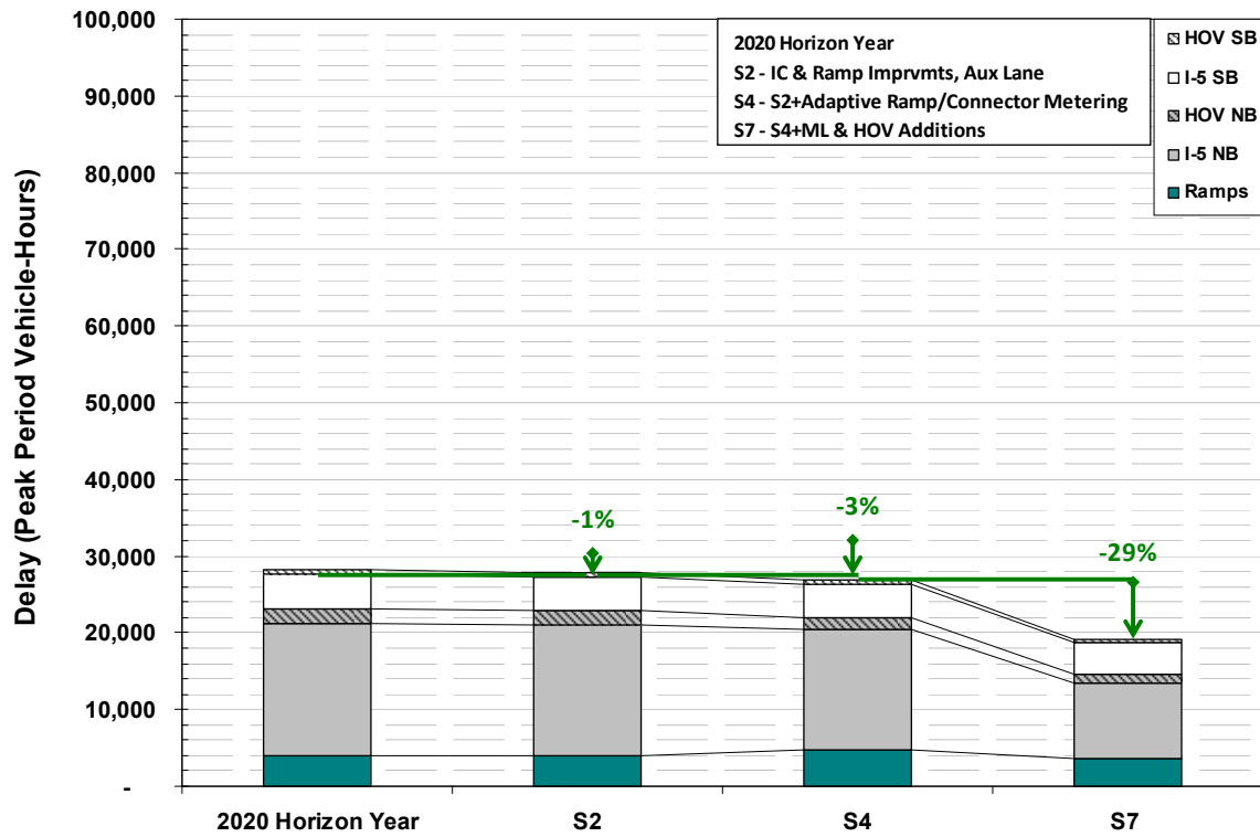
Exhibit ES-30: 2020 PM Peak Micro-Simulation Delay by Scenario
