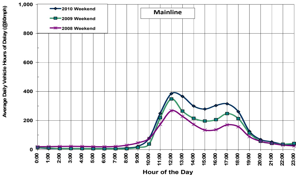
Exhibit ES-21: Weekend Northbound Mainline Lanes Hourly Delay (2008-2010)
