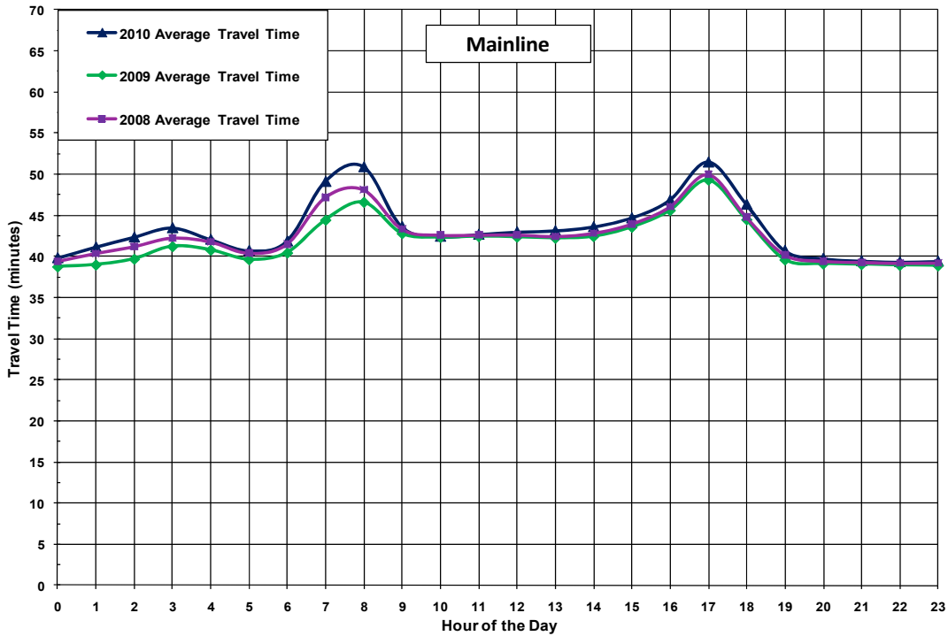
Exhibit ES-11: Southbound Mainline Lanes Travel Time by Hour (2008-2010)
