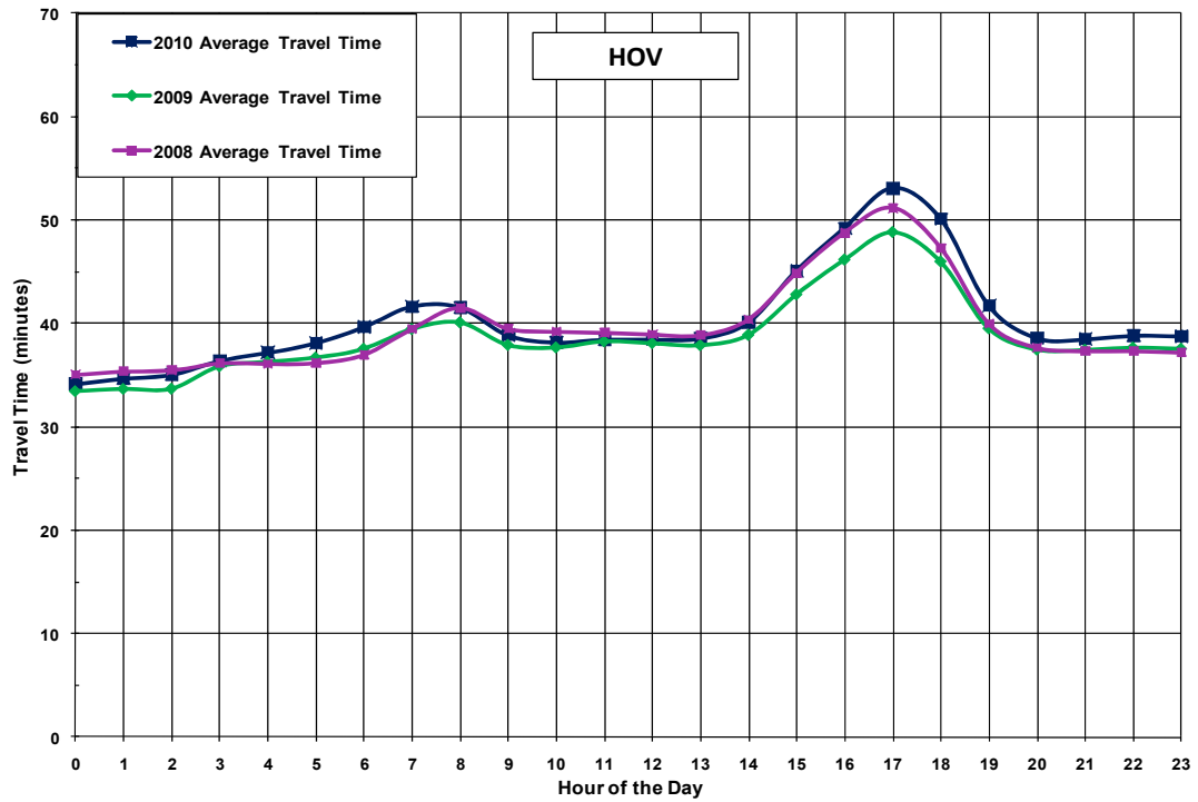
Exhibit ES-12: Northbound HOV Lanes Travel Time by Hour (2008-2010)
