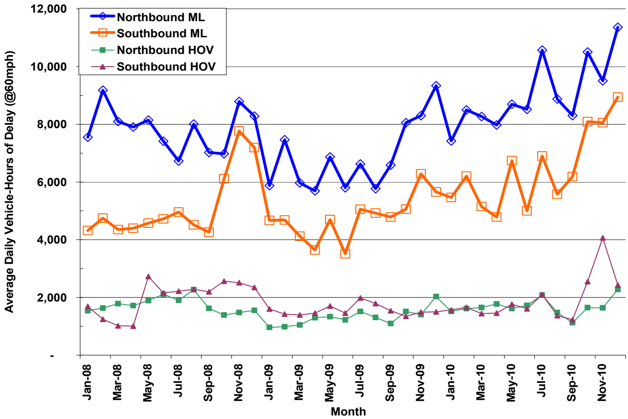
Exhibit ES-3: Average Weekday Delay by Month (2008-2010)
