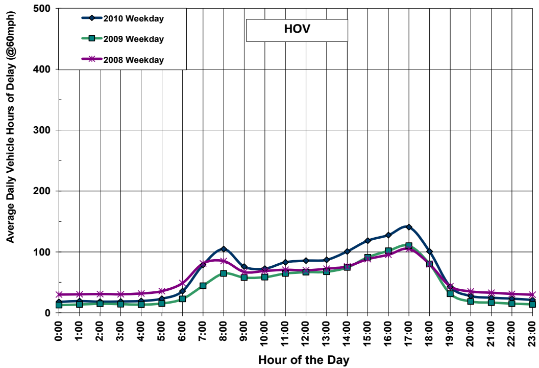
Exhibit ES-9: Southbound HOV Lanes Hourly Delay (2008-2010)
