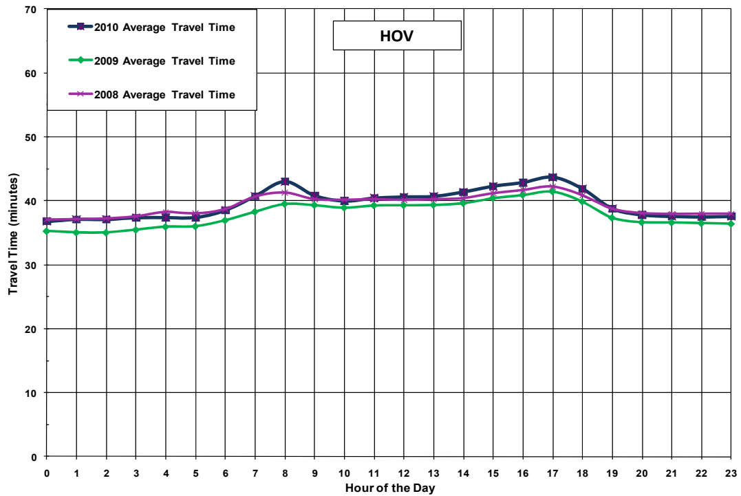
Exhibit ES-13: Southbound HOV Lanes Travel Time by Hour (2008-2010)
