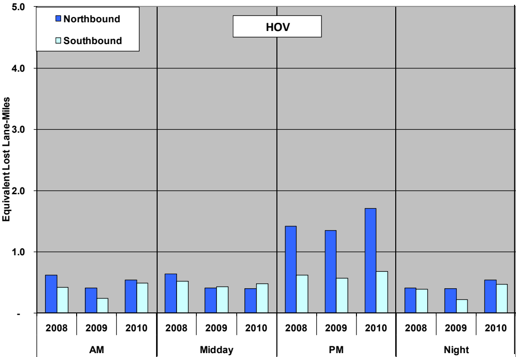
Exhibit ES-20: HOV Lost Lane-Miles by Direction and Period (2008-2010)
