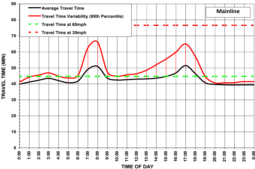
Exhibit ES-15: Southbound Mainline Lanes Travel Time Variability (2010)
