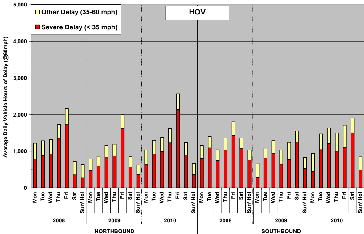
Exhibit ES-5: HOV Lanes Delay by Day of Week (2008-2010)
