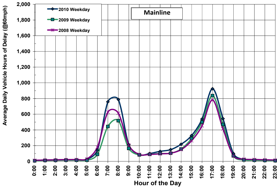
Exhibit ES-7: Southbound Mainline Lanes Hourly Delay (2008-2010)
