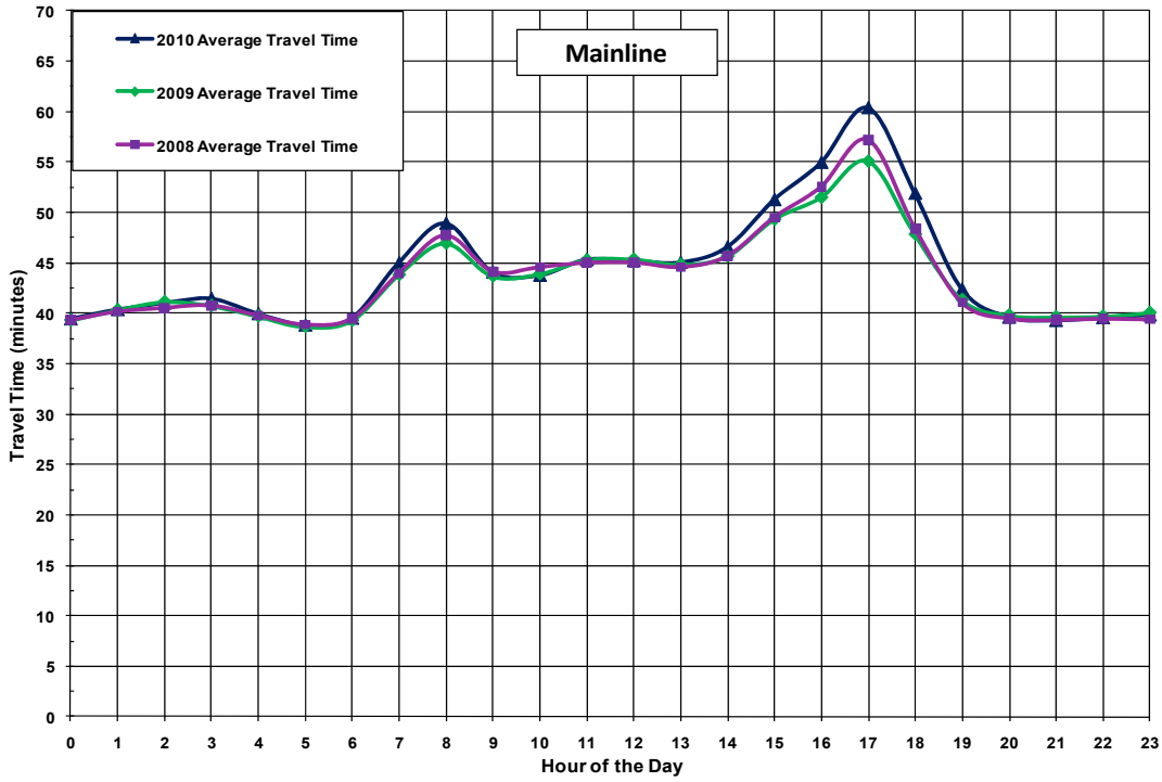
Exhibit ES-10: Northbound Mainline Lanes Travel Time by Hour (2008-2010)
