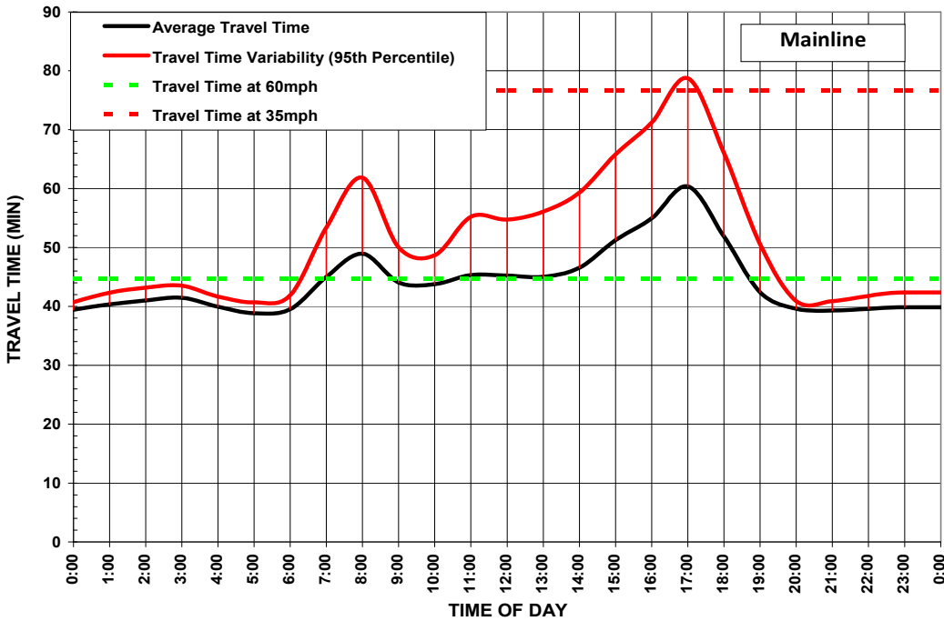
Exhibit ES-14: Northbound Mainline Lanes Travel Time Variability (2010)
