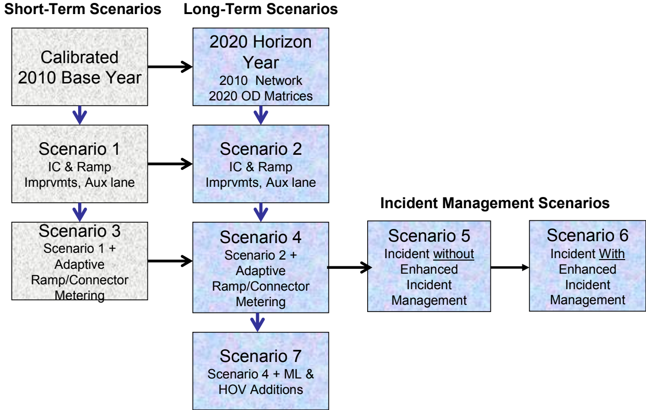
Exhibit ES-26: Paramics Micro-Simulation Modeling Approach
