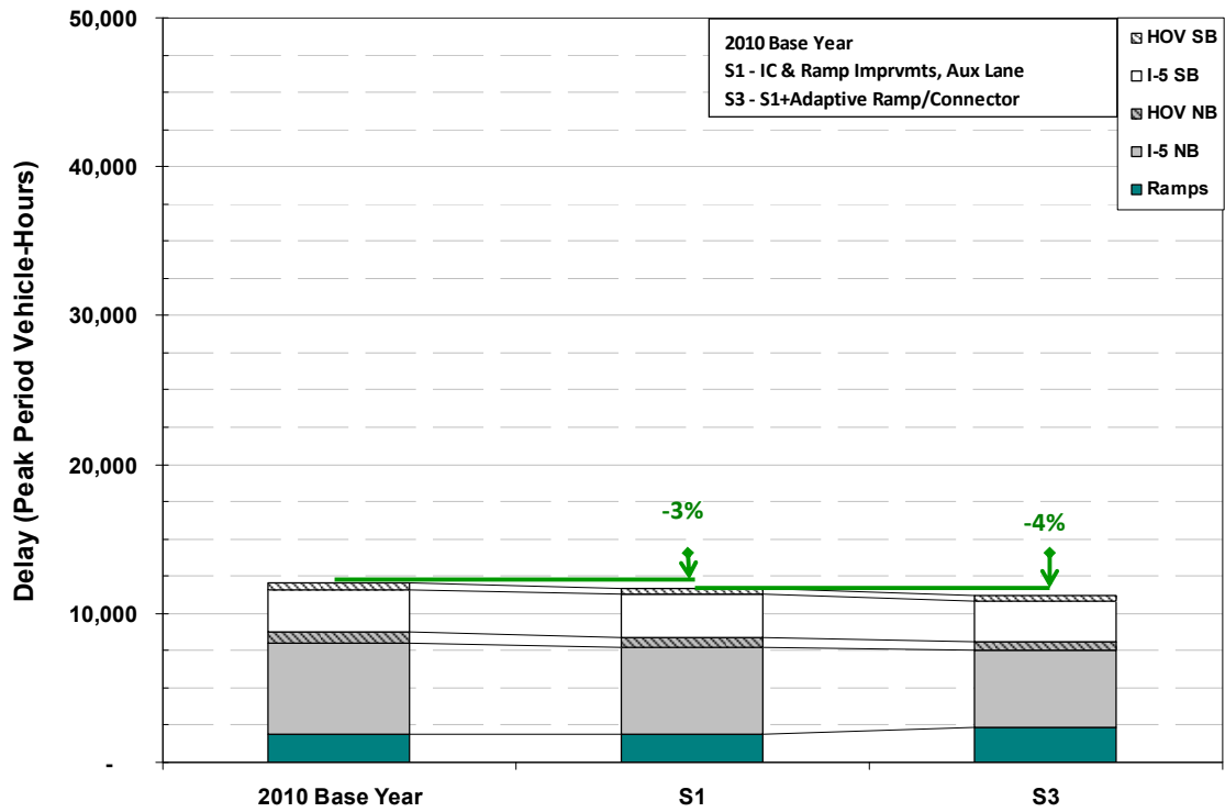
Exhibit ES-28: 2010 PM Peak Micro-Simulation Delay by Scenario
