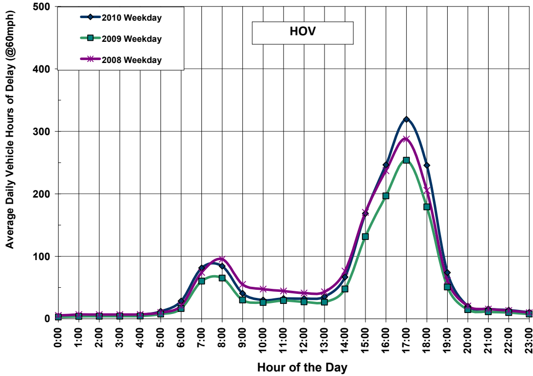
Exhibit ES-9: Southbound HOV Lanes Hourly Delay (2008-2010)
