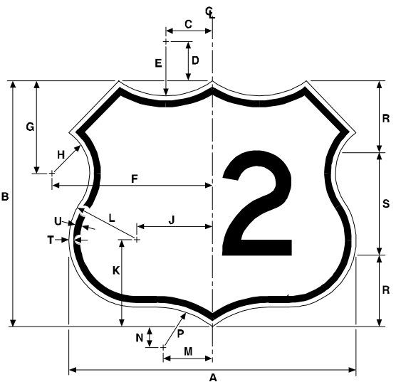
DIMENSIONS (MILLIMETERS)
