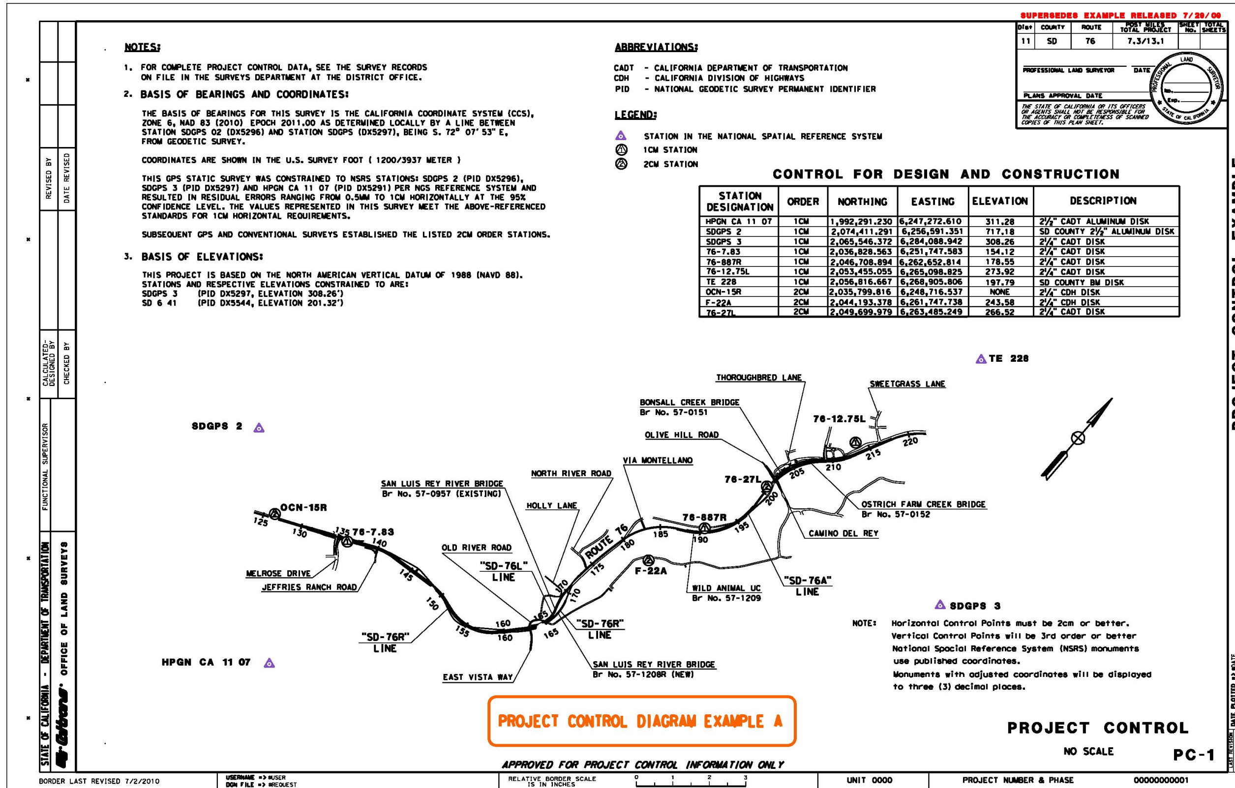
Figure 9.6-2 Project Control Diagram Example
