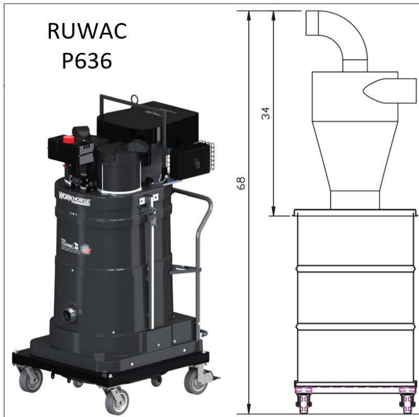
Figure 2.9: RUWAC vacuum
