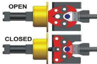
REAR HYDRAULIC CLAW DOOR. Rear hydraulic claw door has an over-center locking mechanism for a no-fuss positive lock and unlock.
