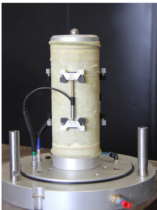
Image 3: Triaxial testing to simulate stiffness changes on FDR projects.
