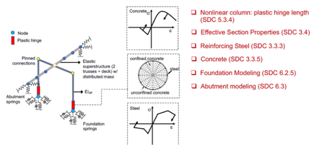
Image 2: Modeling approach in OpenSees
