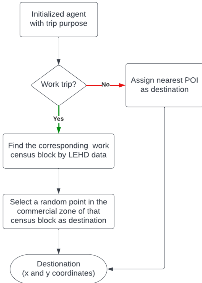
Figure 8. Destination assignment logic
