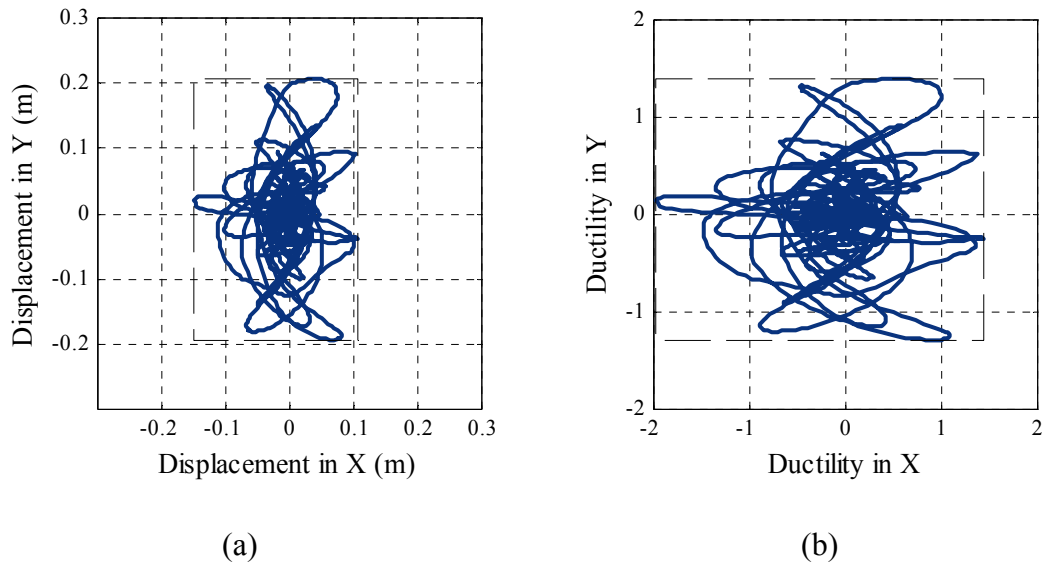
Fig. 2.5 Displacement orbits at top of bridge column: (a) absolute displacements, (b) normalized displacements.
