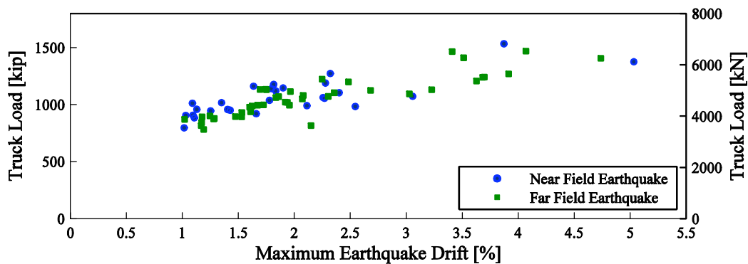
Fig. 5.6 Relation between maximum earthquake drift and post-earthquake bridge truck load capacity (Rx0 abutment, residual drift of 1.0%, truck is in curb lane).
