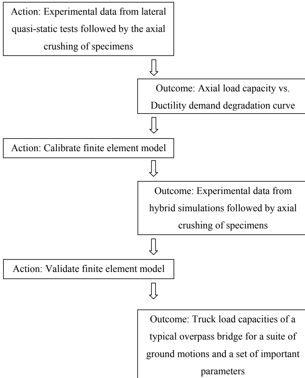
Fig. 1.1 Methodology for evaluation of remaining capacity of a bridge to carry traffic load after earthquake.
