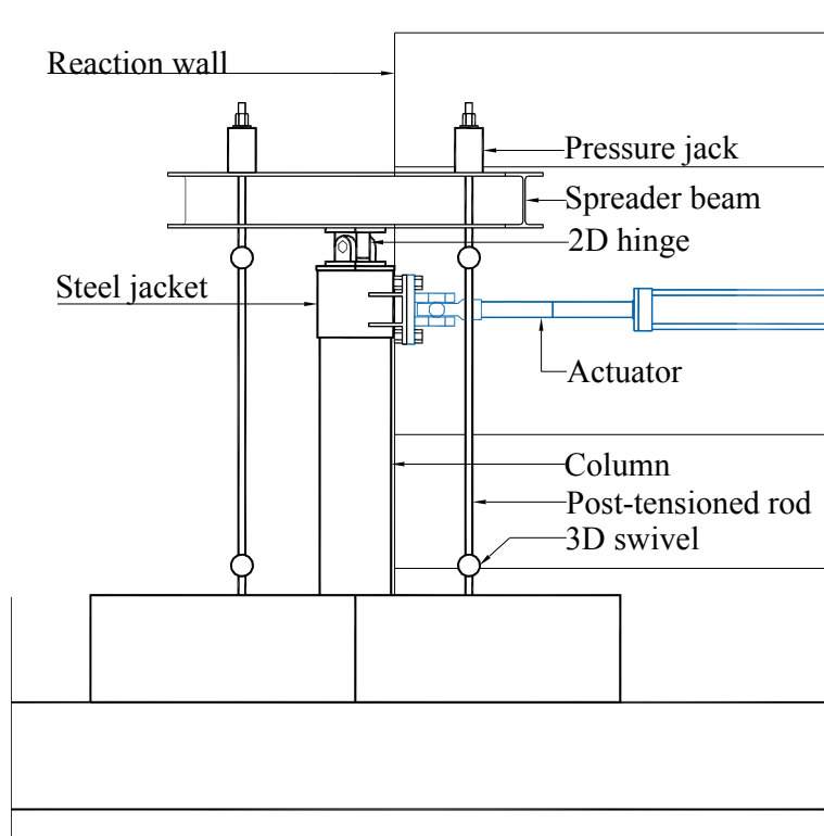
Fig. C.3 Elevation (A-A) of experimental setup.
