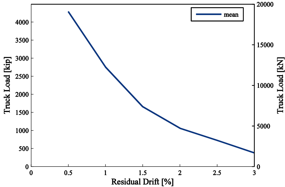
Fig. 5.7 Relation between residual drift and post-earthquake bridge truck load capacity (Rx0 abutment, truck is in fast lane).
