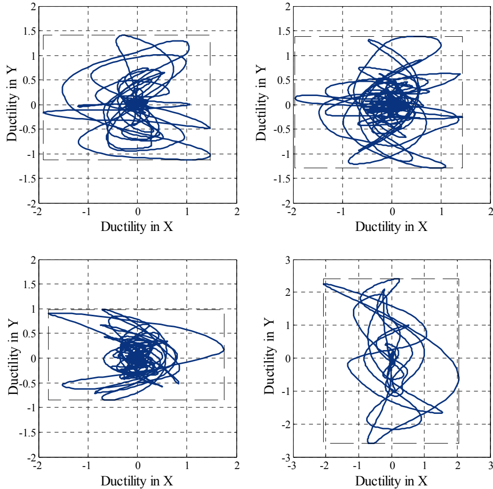
Fig. B.3 Displacement orbits at top of column for thrust-fault earthquake.
