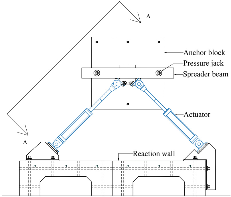
Fig. 3.14 Plan view of hybrid simulation experimental setup.
