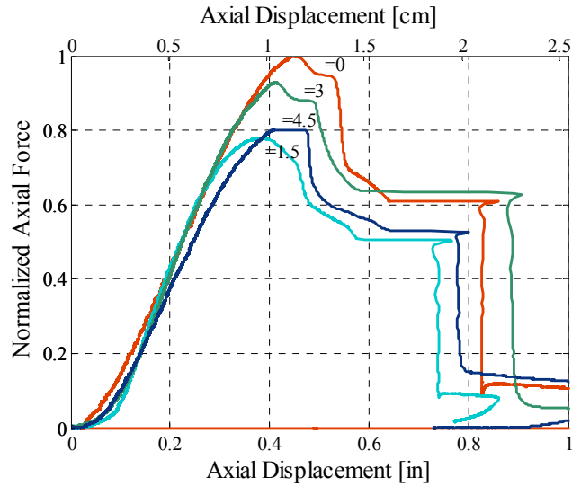
Fig. 2.29 Comparison of axial force-displacement relationships for tests Base0, Base15, Base30, and Base45.
