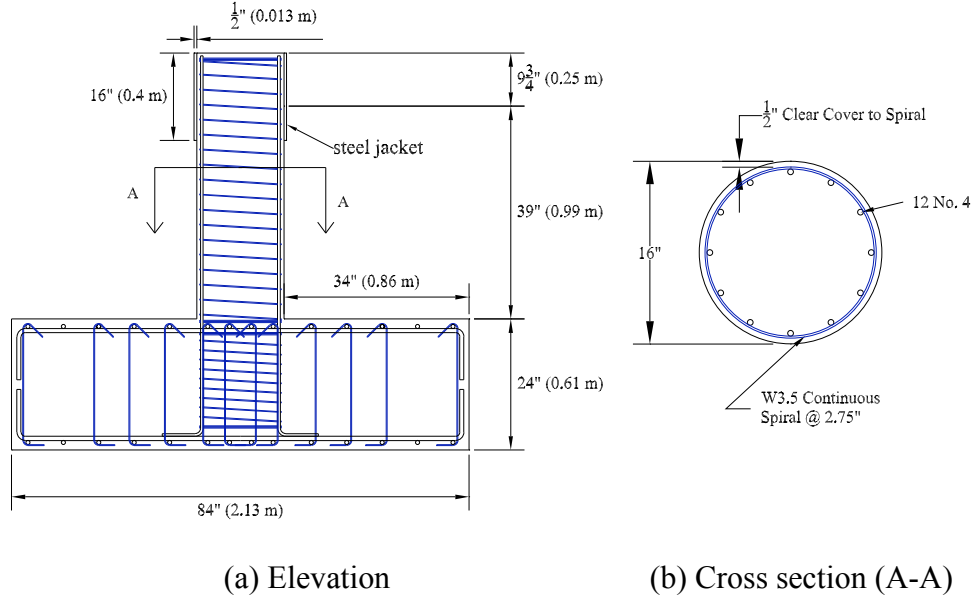
Fig. 2.3 Geometry and reinforcement of Shear-Short Column specimen.
