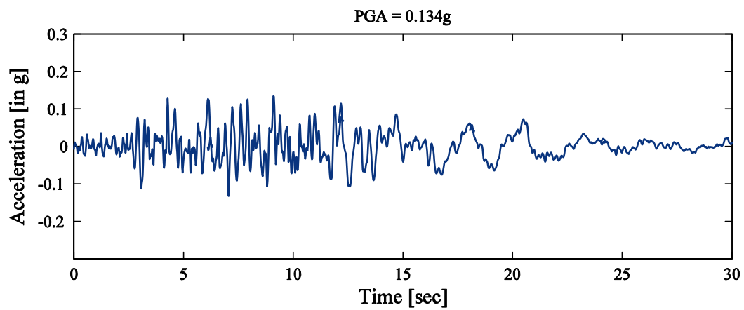
(b) Horizontal component of ground motion: longitudinal bridge direction
