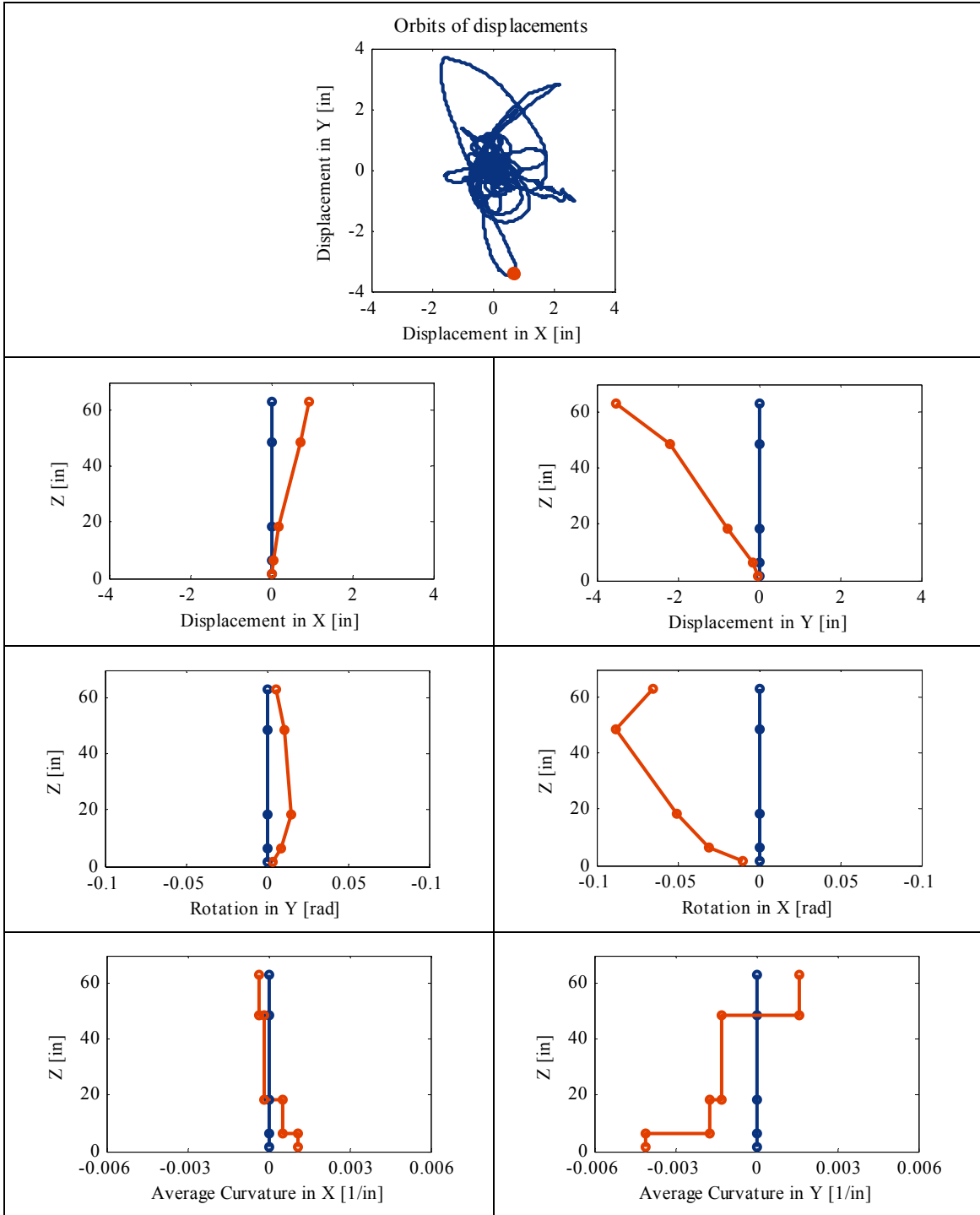
Fig. 3.35 State of displacements, rotations, and average curvatures along height of specimen at a certain time during earthquake (marked point on control point displacement orbit graph).
