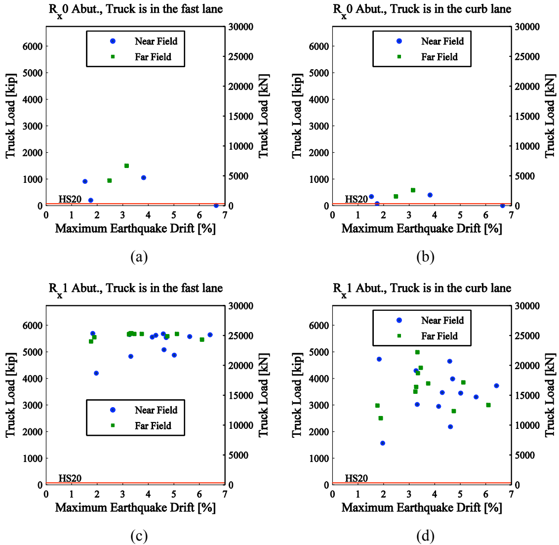
Fig. 5.17 Post-earthquake bridge truck load capacity vs. maximum earthquake drift for residual drift of 1.5% and the following cases: (a) R_x abutment, truck is in fast lane; (b) R_x abutment, truck is in curb lane; (c) R_x abutment, truck is in fast lane; (d) R_x abutment, truck is in curb lane.
