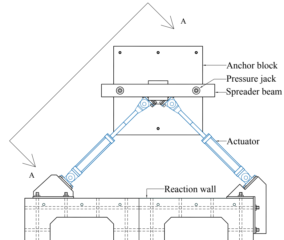
Fig. C.2 Plan view of experimental setup.
