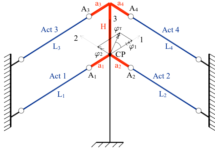
Fig. 3.17 Schematic presentation of rigid column extension (red) and actuators (dark blue) at beginning of hybrid simulation.
