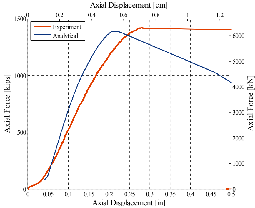
Fig. 4.18 Axial force-displacement relationships: experimental vs. analytical relationship for bridge column exposed to medium seismic intensity (HSM test).
