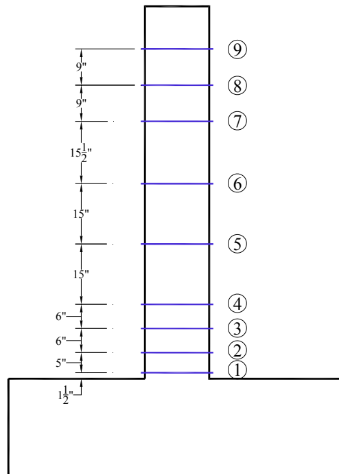
Fig. 3.20 Externally instrumented levels along height of hybrid simulation specimens.
