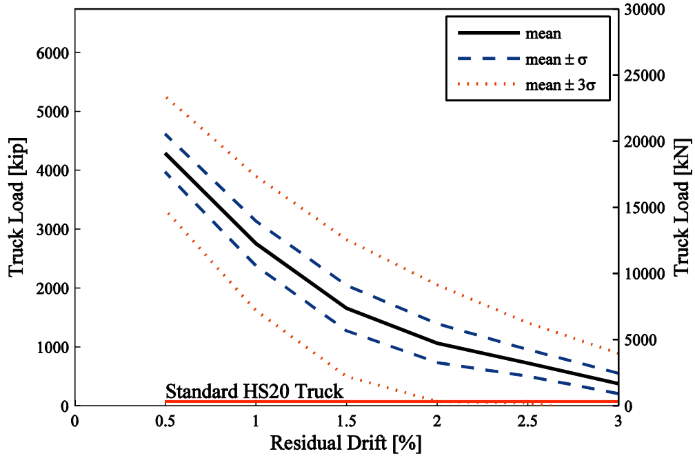
Fig. 5.13 Degradation of post-earthquake bridge truck load capacity with increase in residual drift for case of Rx0 abutments when truck load is in fast lane.
