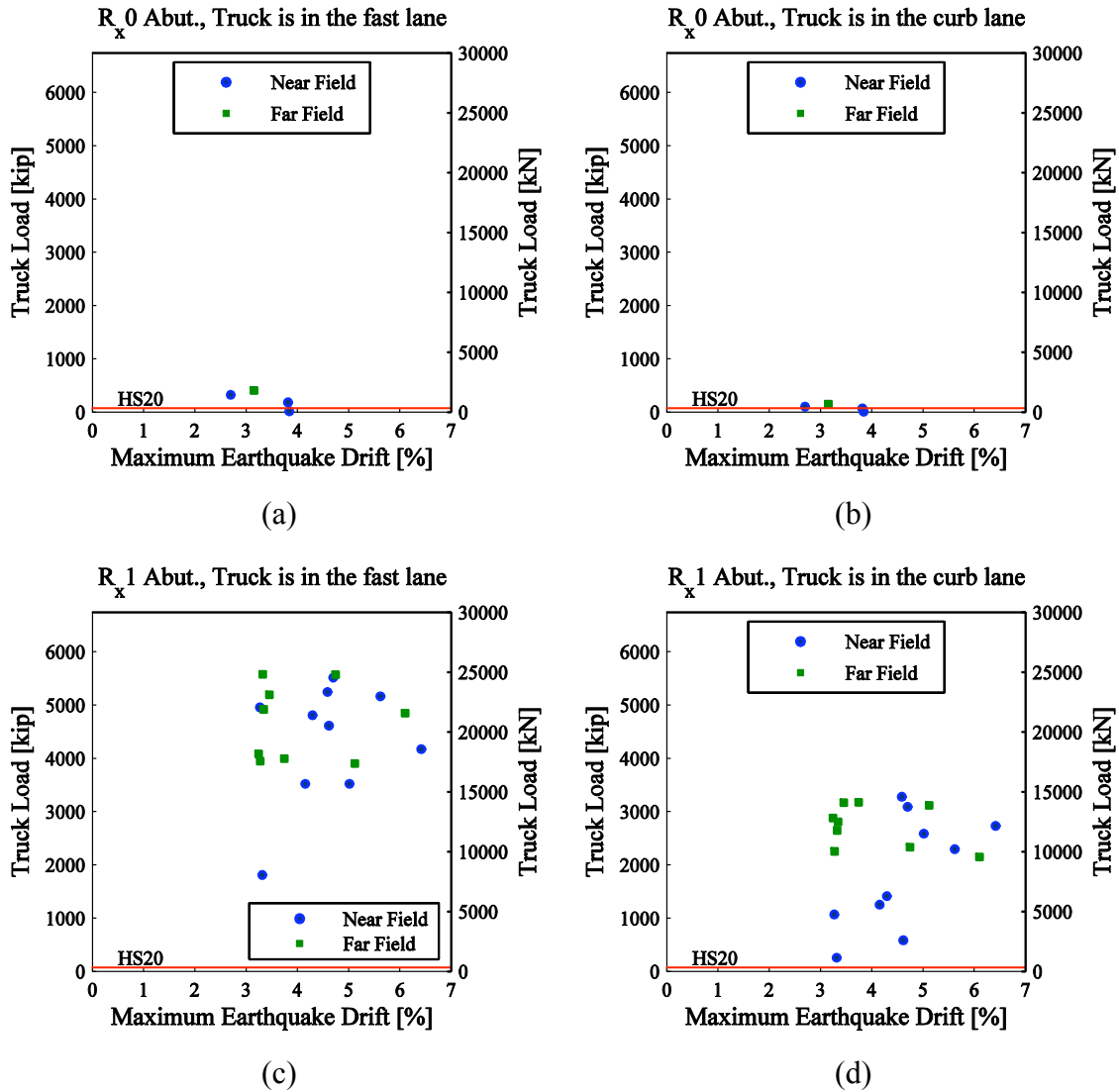
Fig. 5.19 Post-earthquake bridge truck load capacity vs. maximum earthquake drift for residual drift of 2.5% and the following cases: (a) Rx0 abutment, truck is in fast lane; (b) Rx0 abutment, truck is in curb lane; (c) Rx1 abutment, truck is in fast lane; (d) Rx1 abutment, truck is in curb lane.
