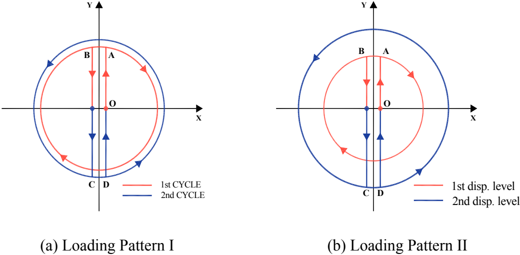
Fig. B.4 Two loading patterns considered for quasi-static tests.
