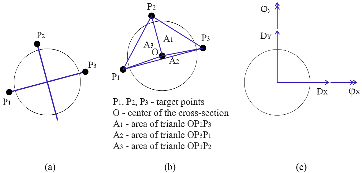
Fig. C.12 Transformation of displacements at target points to displacements and rotations at centroid of column's cross section that plane defined by points P1, P2, and P3 intersects.
