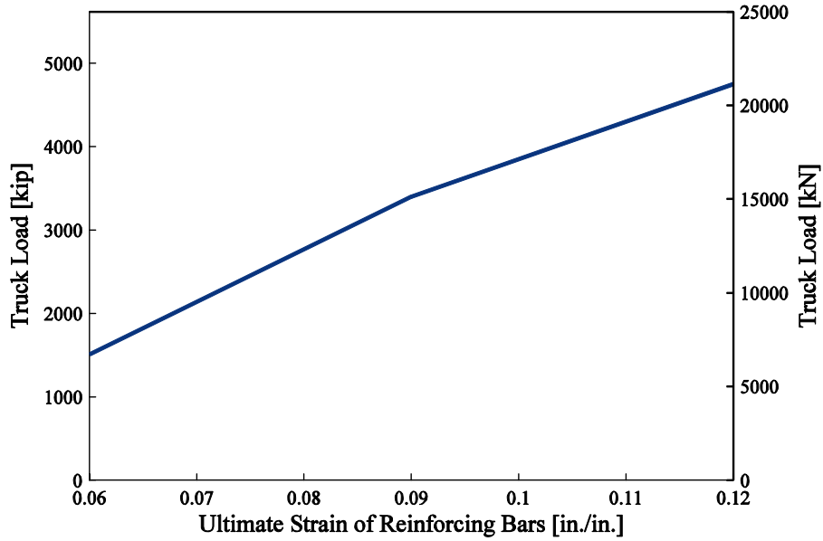
Fig. 5.9 Relation between ultimate strain of reinforcing bars and post-earthquake bridge truck load capacity (Rx1 abutment, residual drift of 2.5%, truck is in curb lane, earthquake vvnuy from Van Nuys earthquake bin).
