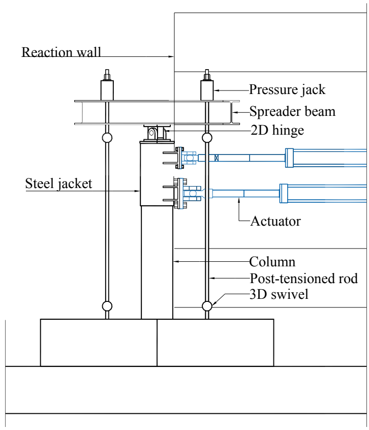
Fig. 3.15 Elevation (A-A) of hybrid simulation experimental setup.
