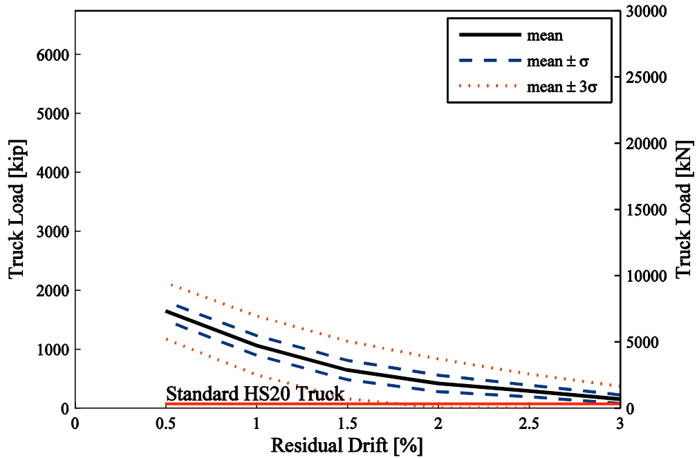
Fig. 5.14 Degradation of post-earthquake bridge truck load capacity with increase in residual drift for case of Rx0 abutments when truck load is in curb lane.
