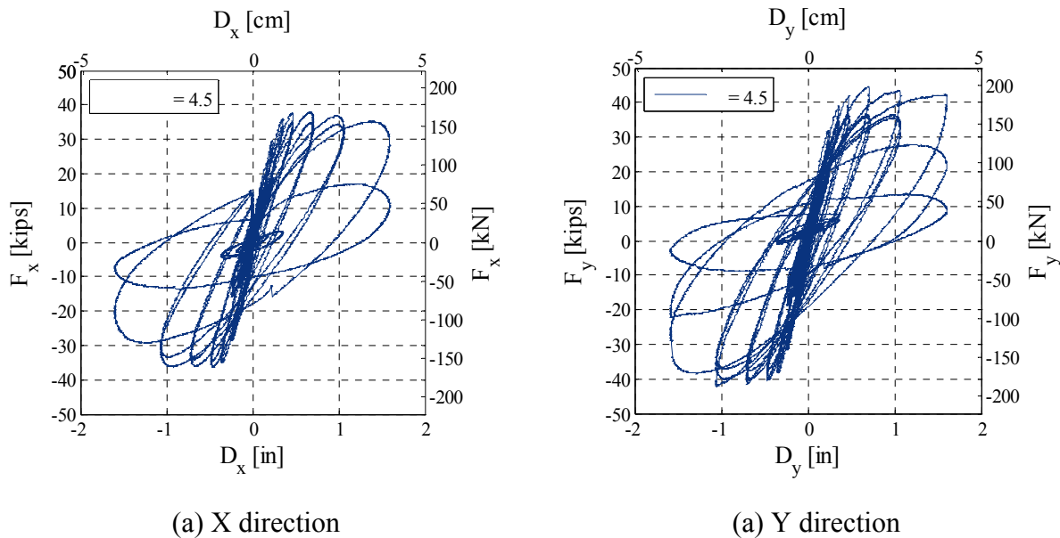
Fig. 2.31 Lateral force-displacement response curves in two major directions (X and Y) for ShearShort45 test.
