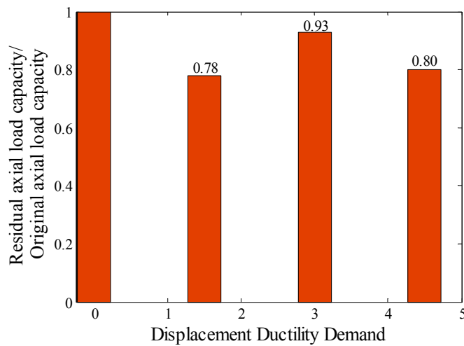
Fig. 2.30 Degradation of axial strength of laterally damaged specimens.
