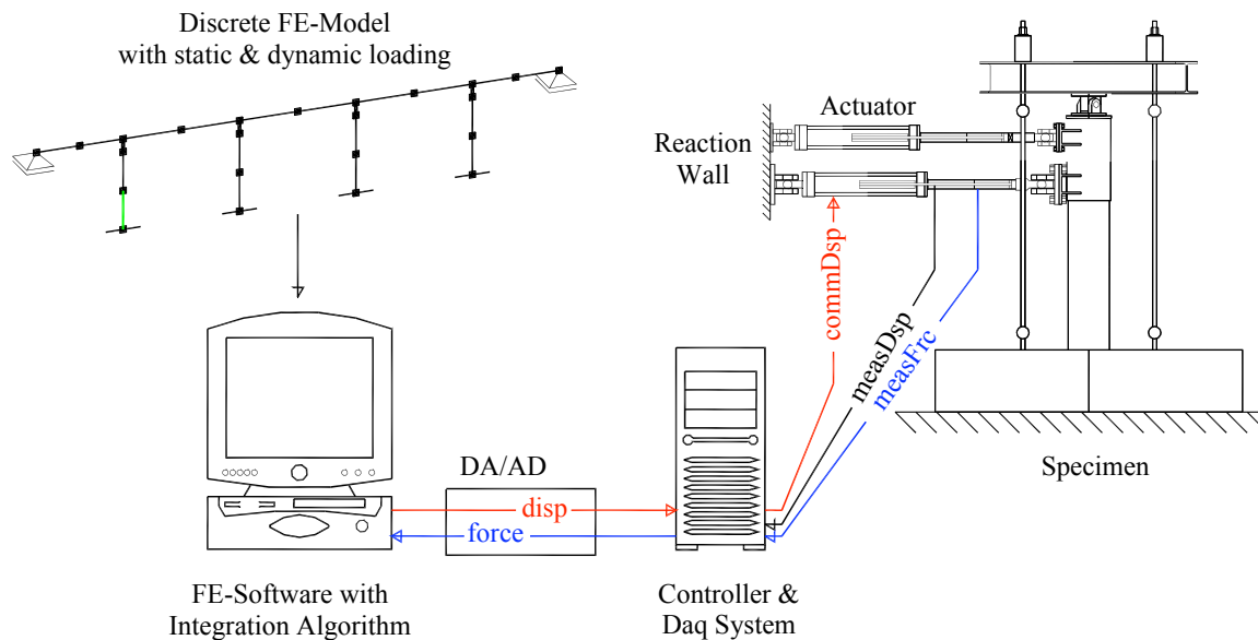
Fig. 3.1 Key components of hybrid simulation.
