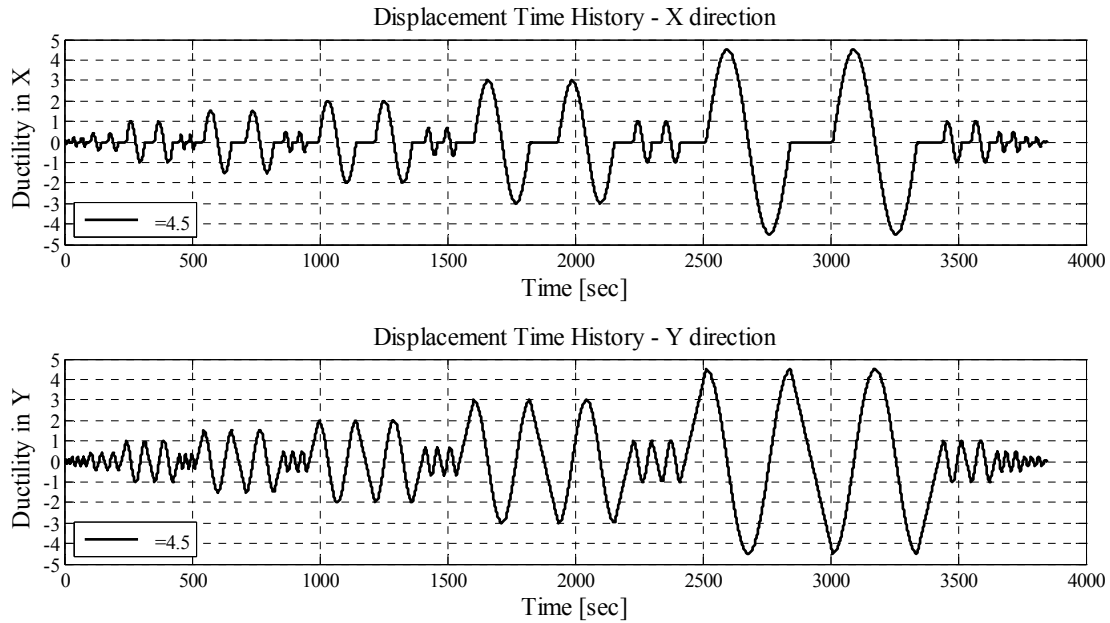
Fig. 2.7 Displacement history for test Base45.
