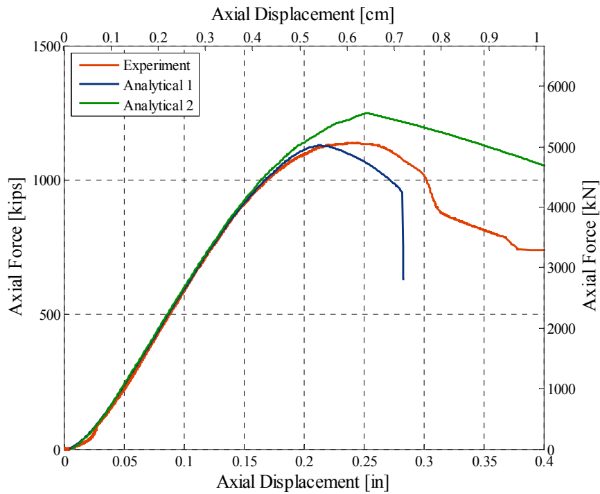
Fig. 4.15 Axial force-displacement relationships: experimental vs. analytical relationships for the axial sequence of Base15 test.
