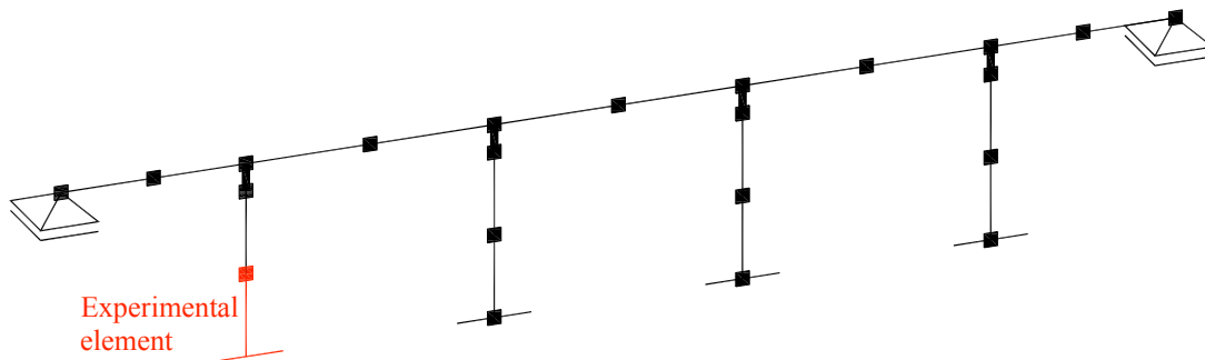
Fig. 3.5 Analytical model of numerical portion of hybrid bridge model.
