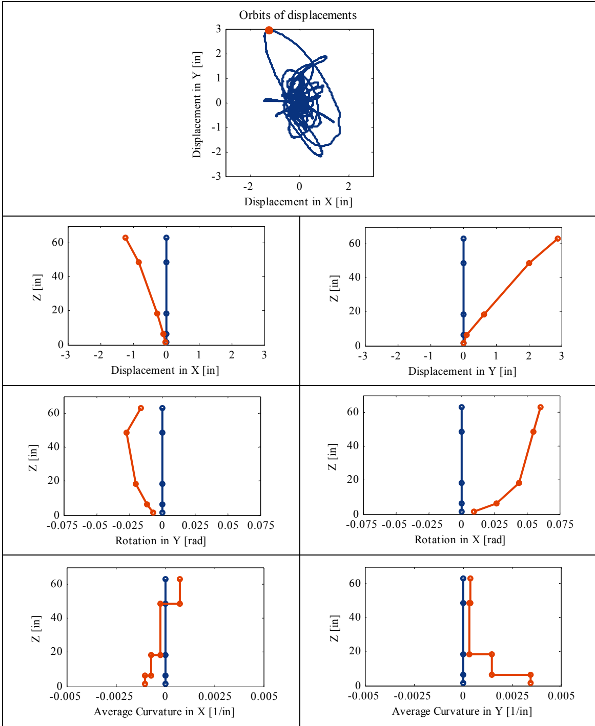
Fig. 3.27 State of displacements, rotations, and average curvatures along height of specimen at a certain time during earthquake (marked by point on control point displacement orbit).
