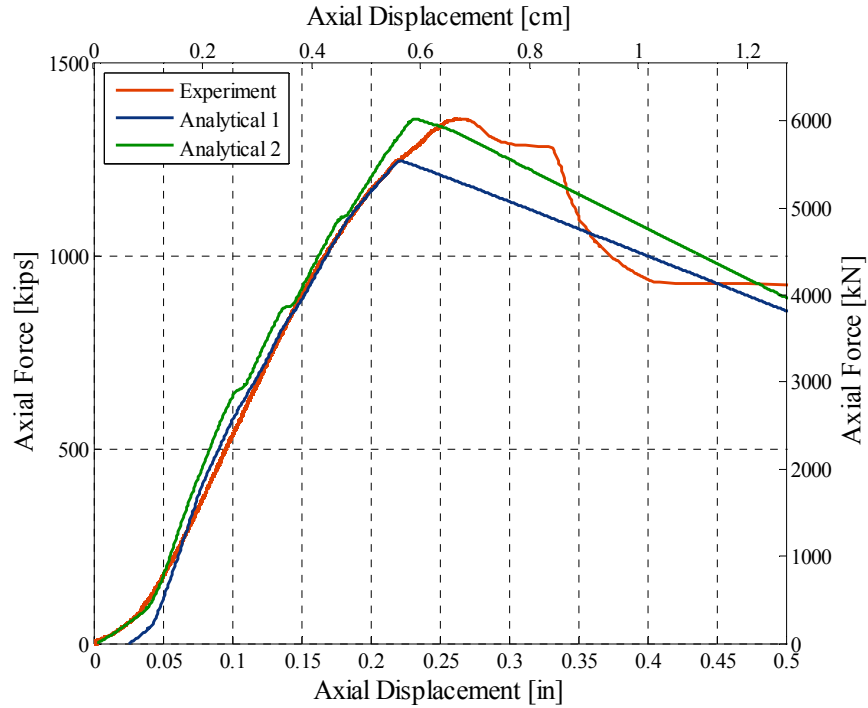
Fig. 4.16 Axial force-displacement relationships: experimental vs. analytical relationships for the axial sequence of Base30 test.
