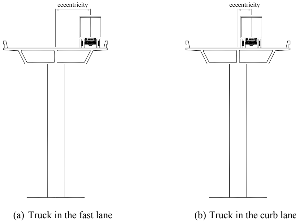
Fig. 5.3 Two considered cases of truck position relative to superstructure centerline.
