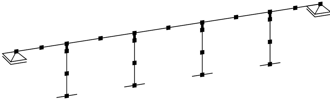
Fig. 5.1 Analytical model of bridge structure.
