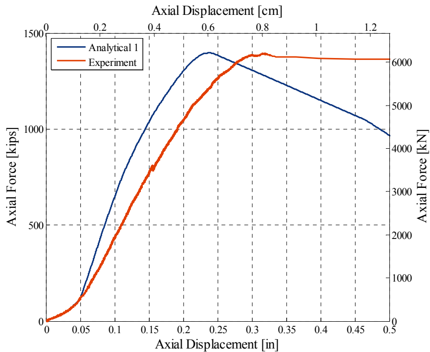
Fig. 4.19 Axial force-displacement relationships: experimental vs. analytical relationship for bridge column exposed to high seismic intensity (HSH test).
