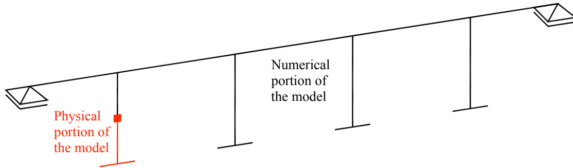
Fig. 3.2 Physical and numerical portions of hybrid bridge model.
