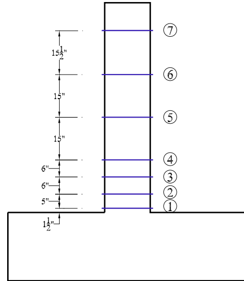
(b) Base-Column specimen
