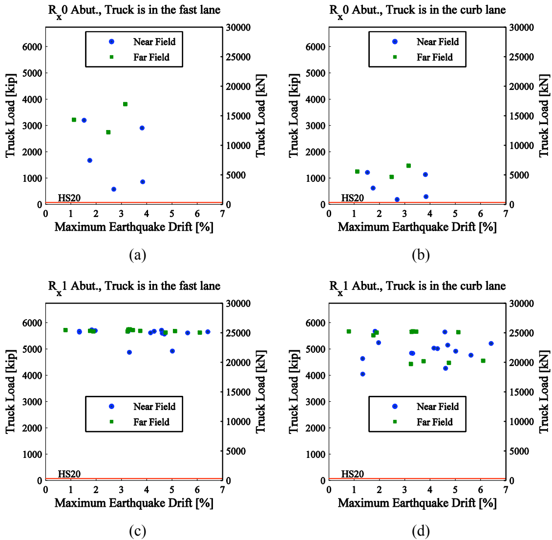
Fig. 5.15 Post-earthquake bridge truck load capacity vs. maximum earthquake drift for residual drift of 0.5% and following cases: (a) R_{x0} abutment, truck is in fast lane; (b) R_{x0} abutment, truck is in curb lane; (c) R_{x1} abutment, truck is in fast lane; (d) R_{x1} abutment, truck is in curb lane.
