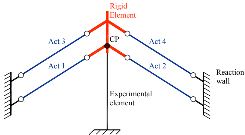
Fig. 3.12 Schematic representation of hybrid simulation setup for lateral load application.
