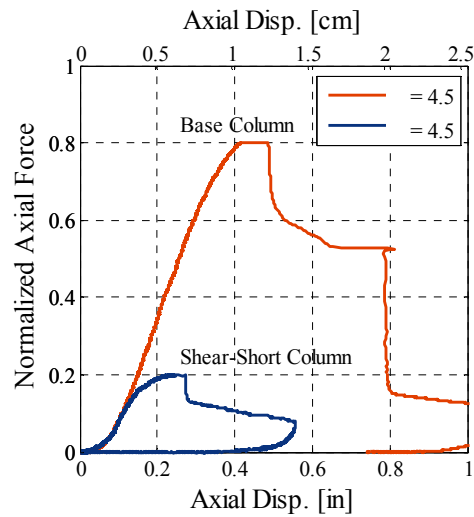
Fig. 2.36 Axial force-displacement relationships for ShearShort45 and Base45 tests.
