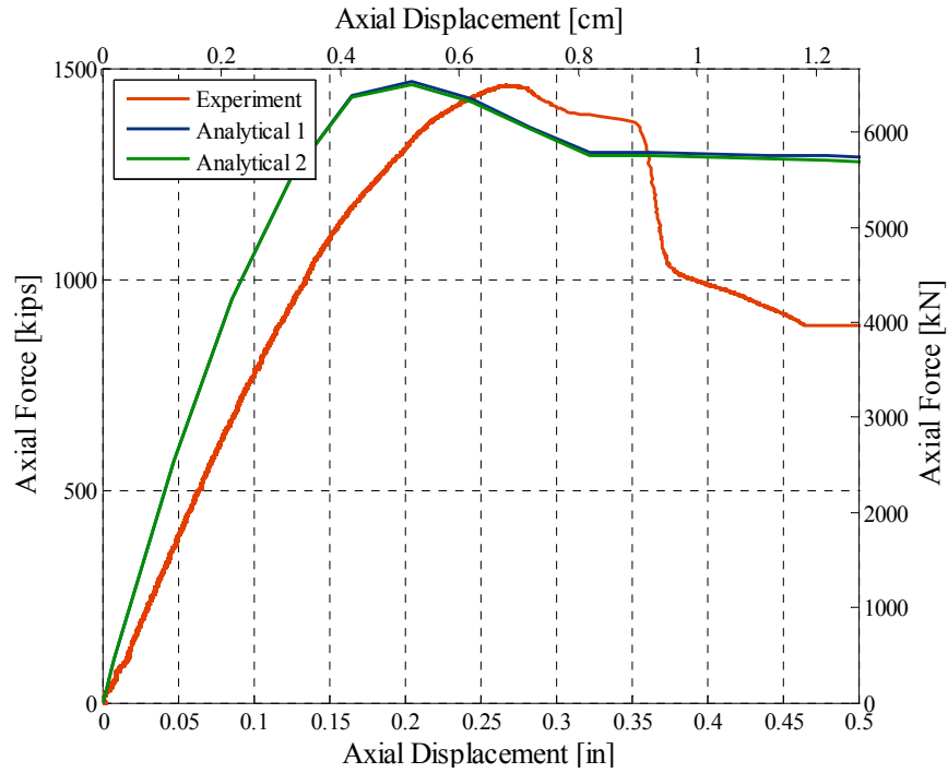
Fig. 4.14 Axial force-displacement relationships: experimental vs. analytical relationships for Base0 test.
