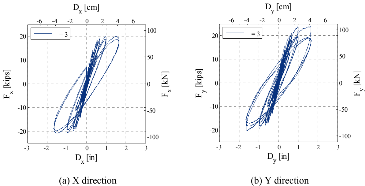
Fig. 2.19 Lateral force-displacement response curves in two major directions (X and Y) for Base30 test.
