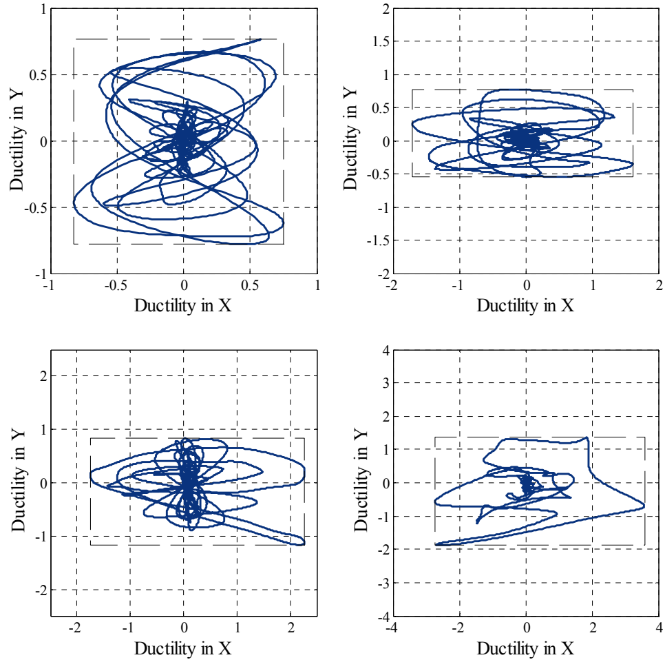
Fig. B.2 Displacement orbits at top of column for strike-slip earthquake; component of motion parallel to fault is aligned with transverse direction of bridge.
