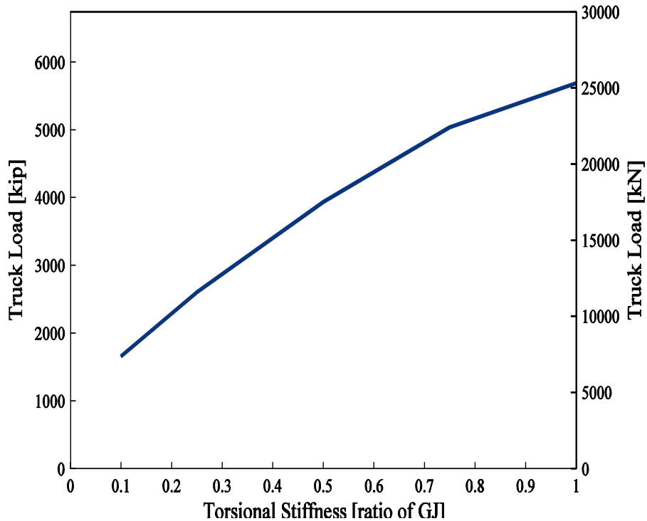
Fig. 5.8 Relation between torsional stiffness of superstructure and post-earthquake bridge truck load capacity (Rx1 abutment, residual drift of 1.0%, truck is in curb lane, earthquake vvvny from Van Nuys earthquake bin).
