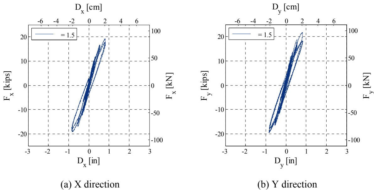
Fig. 2.15 Lateral force-displacement response curves in two major directions (X and Y) for Base15 test.
