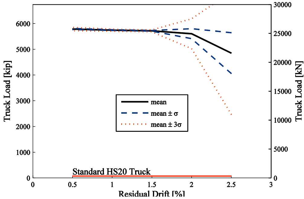
Fig. 5.11 Degradation of post-earthquake bridge truck load capacity with increase in residual drift for case of Rx1 abutments when truck load is in fast lane.
