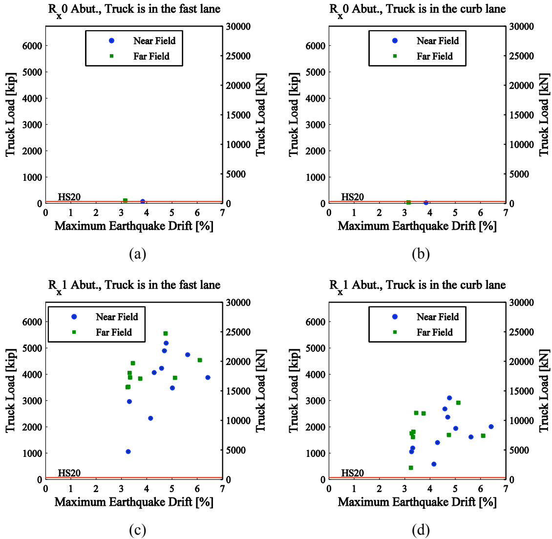
Fig. 5.20 Post-earthquake bridge truck load capacity vs. maximum earthquake drift for residual drift of 3.0% and the following cases: (a) R_{x0} abutment, truck is in fast lane; (b) R_{x0} abutment, truck is in curb lane; (c) R_{x1} abutment, truck is in fast lane; (d) R_{x1} abutment, truck is in curb lane.
