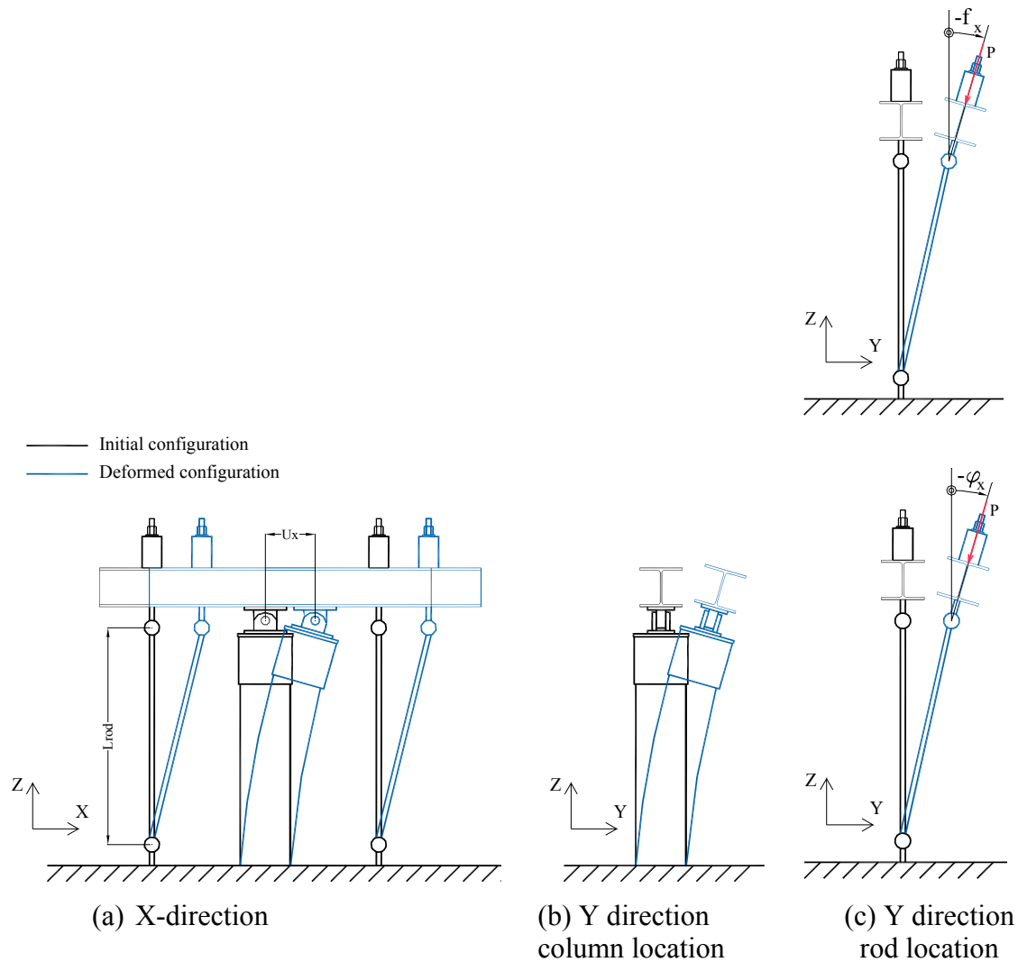
Fig. C.10 Initial vs. deformed configuration of axial test setup in X and Y directions.
