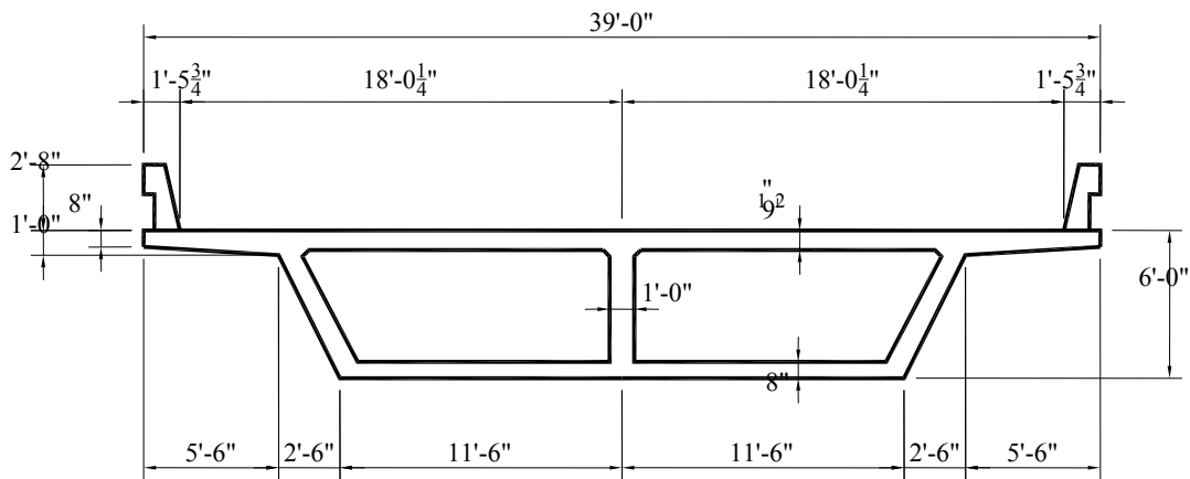
Fig. 3.4 Deck cross section (Ketchum et al. 2004).
