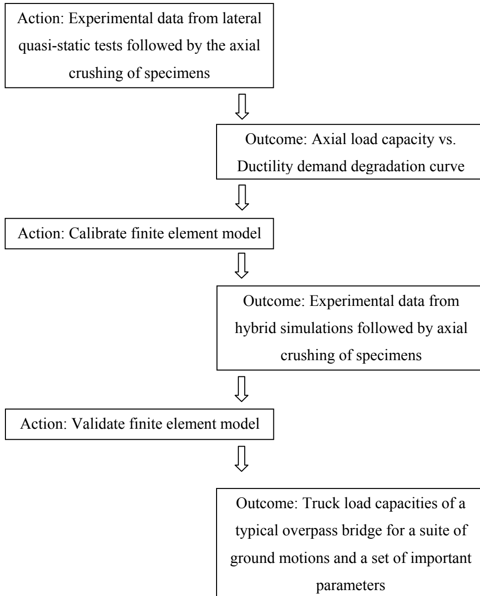
Fig. 6.1 Methodology for evaluation of remaining capacity of bridge to carry traffic load after earthquake.
