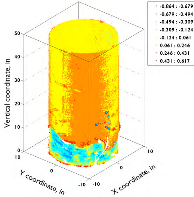
Fig. 2.26 Deviation of column surface from a perfect cylinder with diameter of 16 in.; after lateral sequence of Base45 test.
