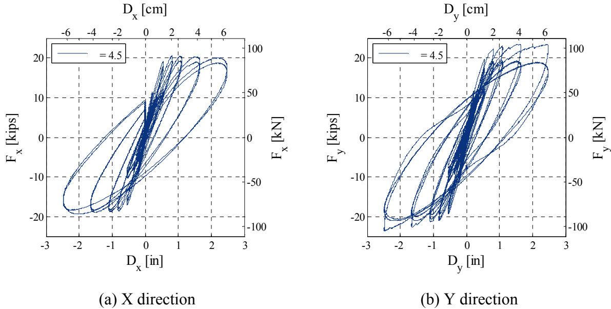
Fig. 2.23 Lateral force-displacement response curves in two major directions (X and Y) for Base45 test.
