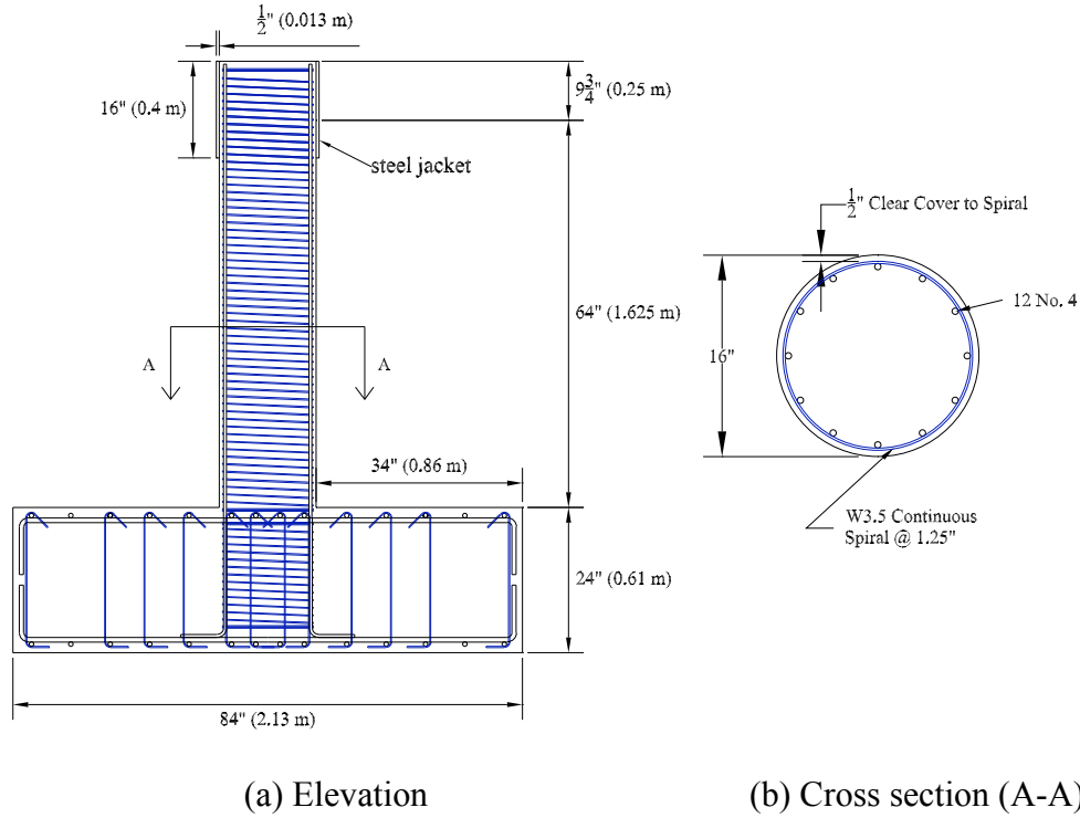
Fig. 2.2 Geometry and reinforcement of Base-Column specimen.
