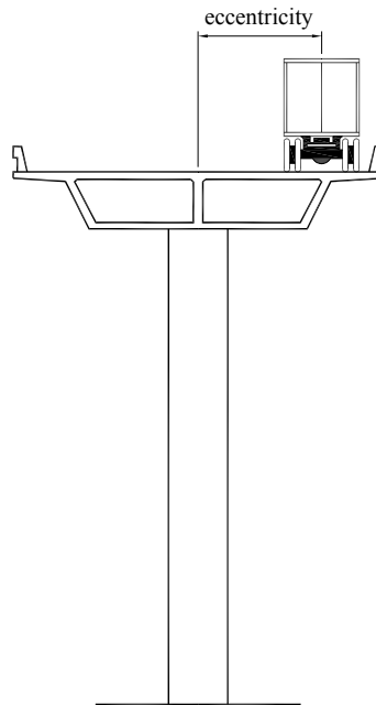
Fig. 3.9 Eccentric position of truck with respect to superstructure centerline.
