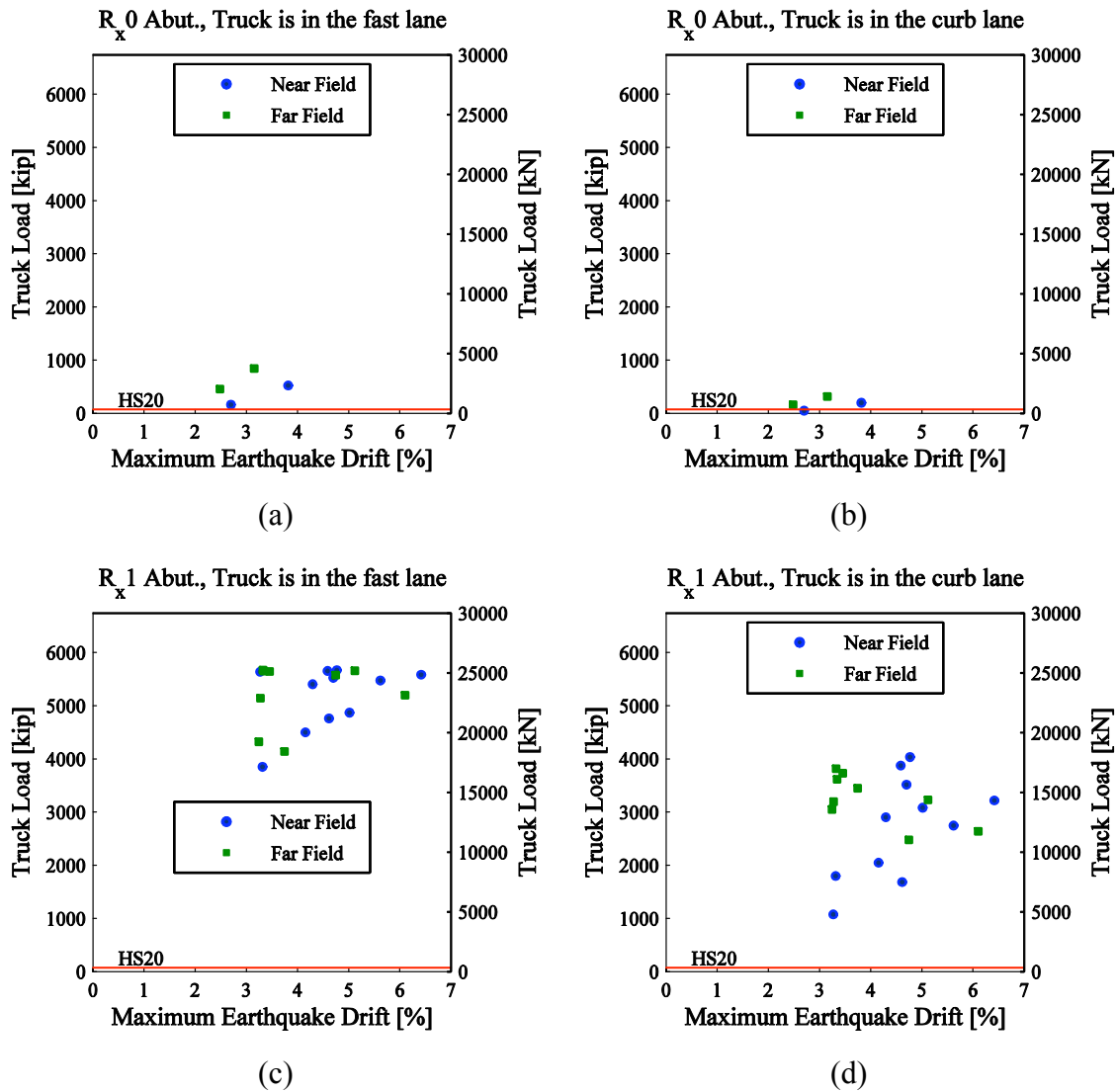
Fig. 5.18 Post-earthquake bridge truck load capacity vs. maximum earthquake drift for residual drift of 2.0% and the following cases: (a) R_x 0 abutment, truck is in fast lane; (b) R_x 0 abutment, truck is in curb lane; (c) R_x 1 abutment, truck is in fast lane; (d) R_x 1 abutment, truck is in curb lane.
