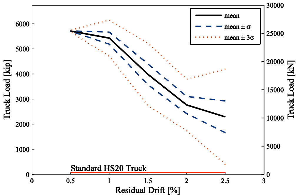
Fig. 5.12 Degradation of post-earthquake bridge truck load capacity with increase in residual drift for case of Rx1 abutments when truck load is in curb lane.
