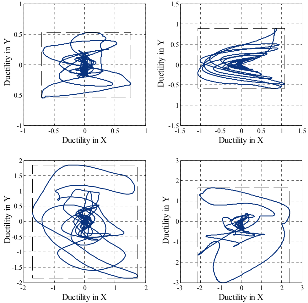
Fig. B.1 Displacement orbits at top of column for strike-slip earthquake; component of motion normal to fault is aligned with transverse direction of bridge.
