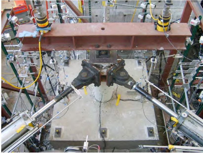
Fig. C.6 Experimental setup.
