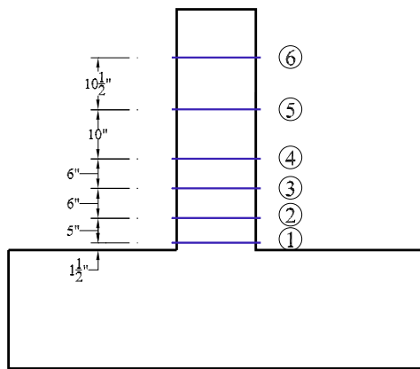
(a) Shear-Short Column specimen
