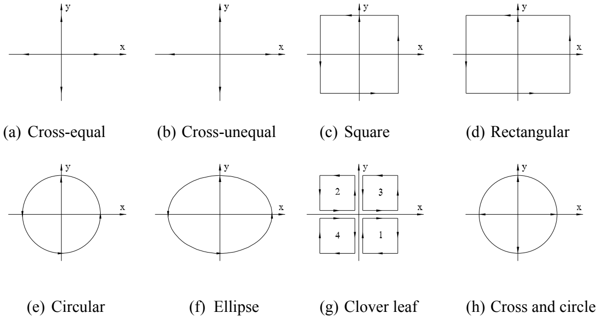
Fig. 2.4 Loading pattern matrix.
