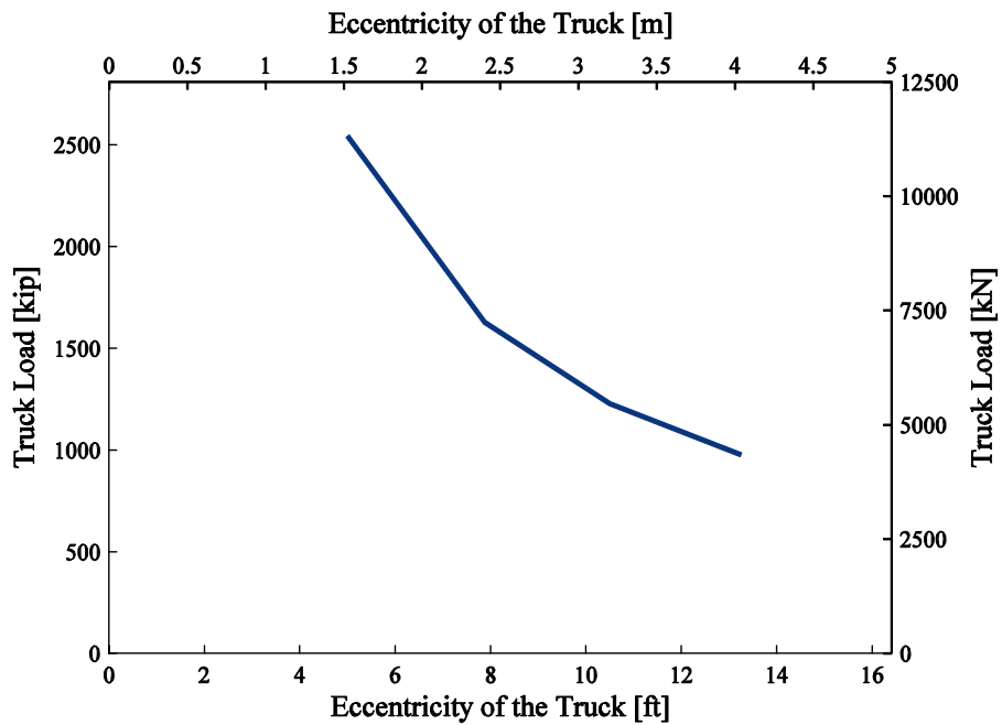
Fig. 5.10 Relation between eccentricity of truck relative to superstructure centerline and post-earthquake bridge truck load capacity (Rx0 abutment, residual drift of 1.0%, earthquake vvnuy from Van Nuys earthquake bin).
