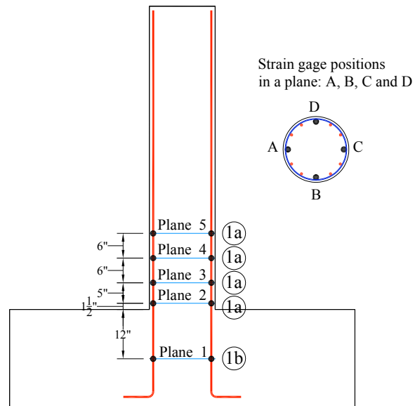
Fig. 2.13 Strain gage locations.
