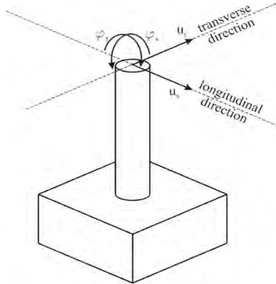
Fig. 3.11 Four DOFs controlled at top of experimental element during hybrid simulations.
