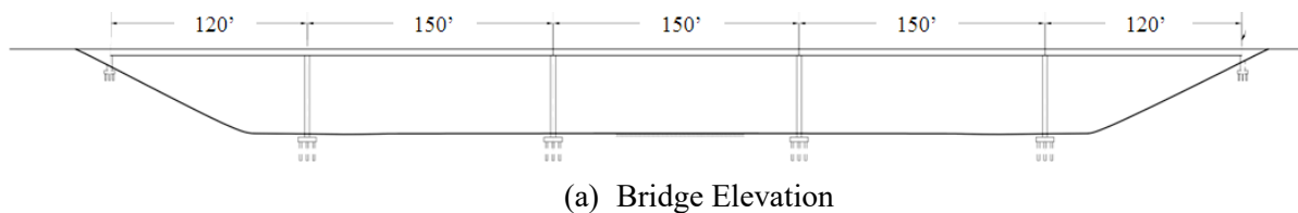
Fig. 2.1 Prototype Caltrans bridges (Ketchum et al. 2004).
