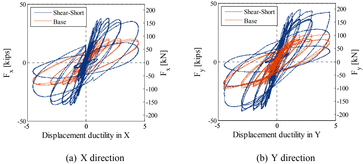
Fig. 2.35 Lateral force-displacement response curves in two major directions (X and Y) for ShearShort45 and Base45 tests.
