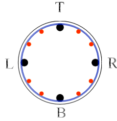
Fig. C.13 Positions of strain gages in section.
