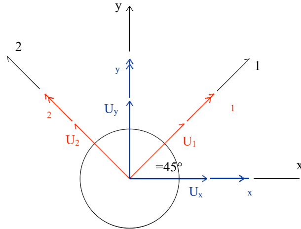
Fig. 3.16 Coordinate transformation.
