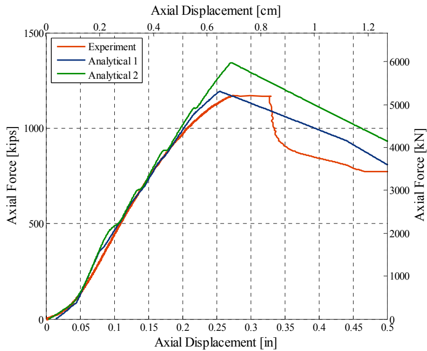
Fig. 4.17 Axial force-displacement relationships: experimental vs. analytical relationships for the axial sequence of Base 45 test.
