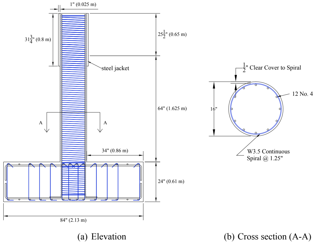
Fig. 3.3 Geometry and reinforcement of specimens tested in hybrid simulation.
