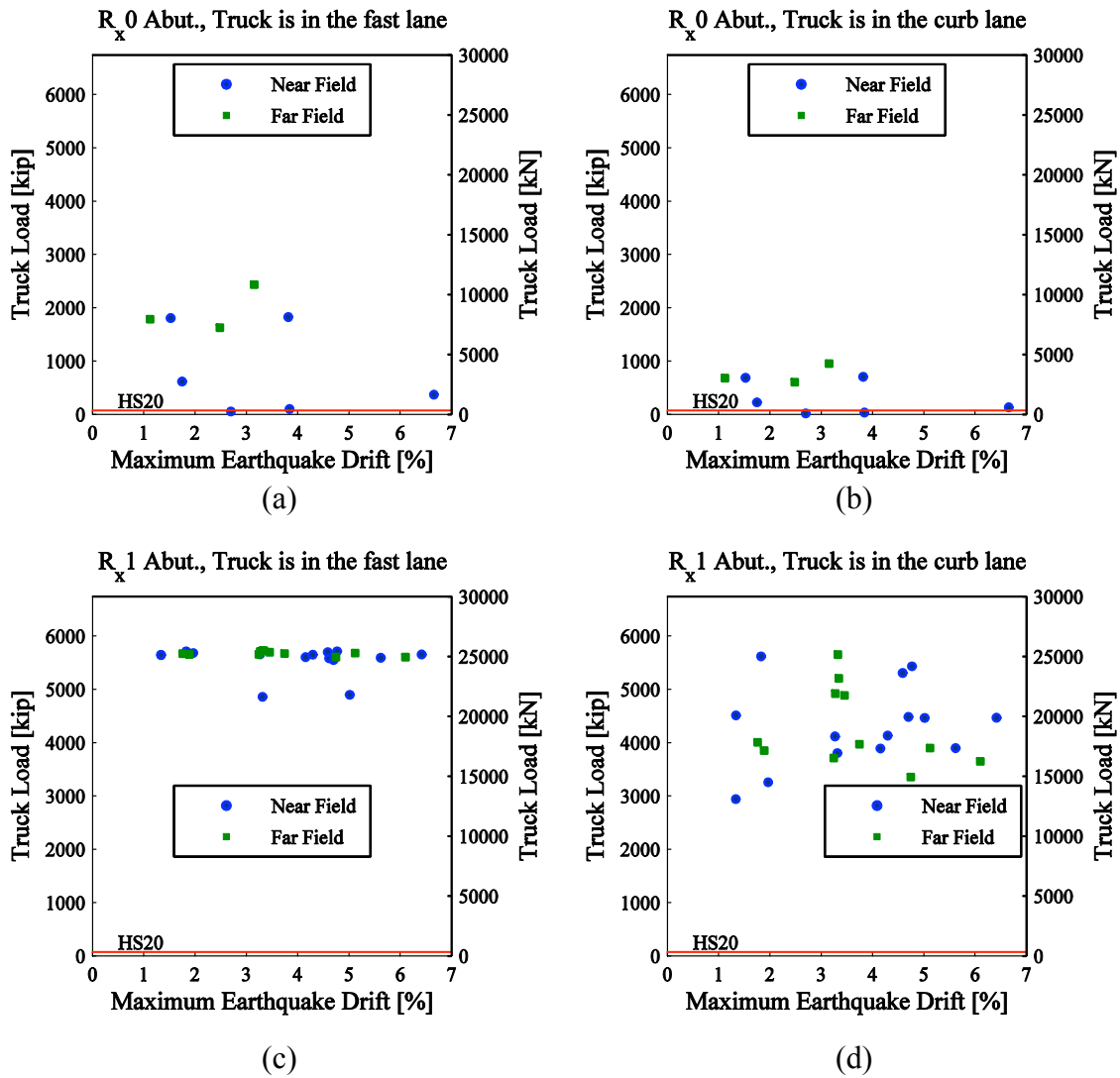
Fig. 5.16 Post-earthquake bridge truck load capacity vs. maximum earthquake drift for residual drift of 1.0% and the following cases: (a) Rx0 abutment, truck is in fast lane; (b) Rx0 abutment, truck is in curb lane; (c) Rx1 abutment, truck is in fast lane; (d) Rx1 abutment, truck is in curb lane.
