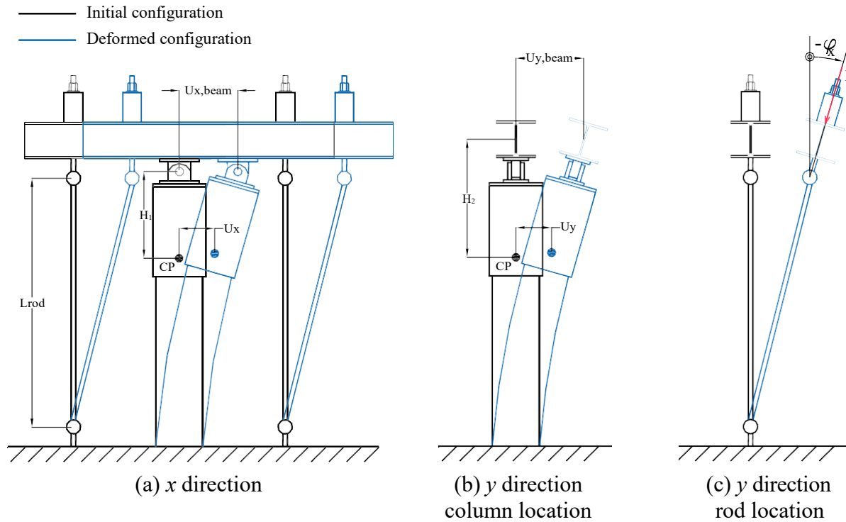
Fig. 3.19 Initial vs. deformed configuration of axial test setup in x and y directions.
