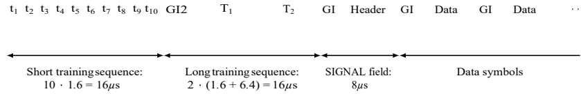
Figure 5.8: OFDM training structure
