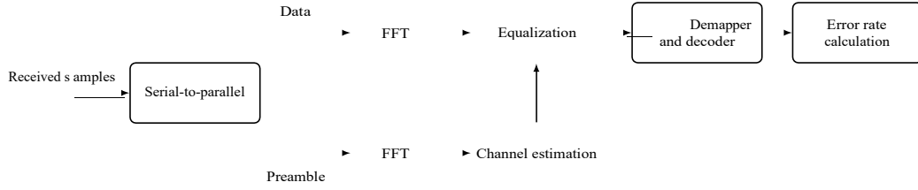
Figure 5.9: Block diagram of the receiver
