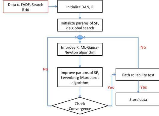
Figure 4.1: RiMAX code flow
