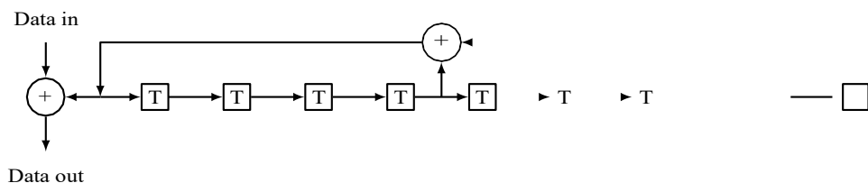
Figure 5.2: Data scrambler
