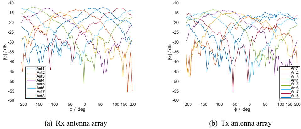
Figure 2.11: Radiation patterns of the antenna array elements, calibrated with the corresponding RF switch
