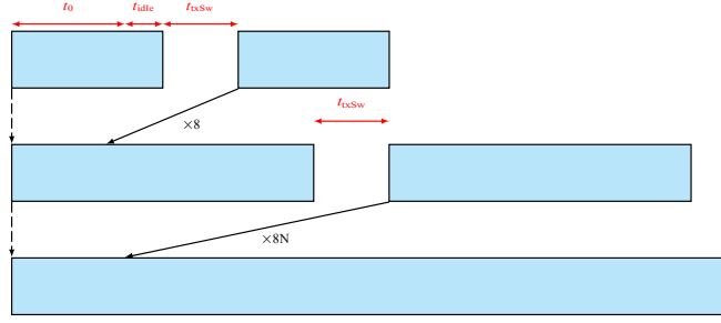
Figure 2.6: Frame structure of MIMO sounding signal
