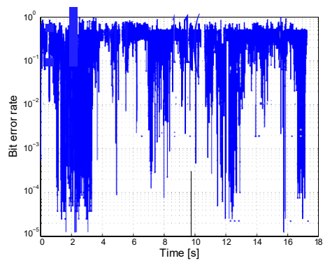
Figure 6.1: Time-varying BER for truck-to-truck communications on a freeway, with the LOS obstructed by other trucks
