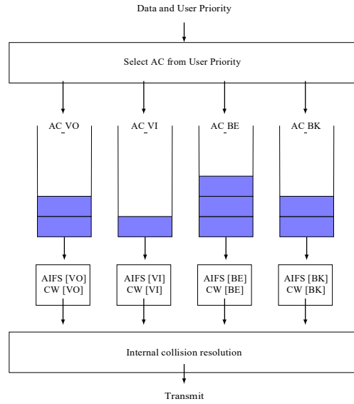
Figure 5.13: EDCA QoS queues
