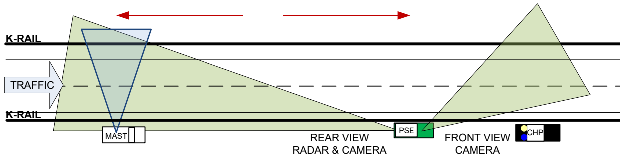
Figure 21. Layout for Field Testing of PSE Technology near Stockton, California.
