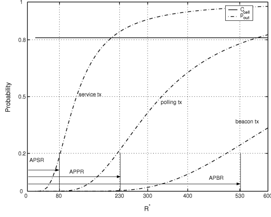
Fig. 20. Cell coverage and outage probability with shadowing, P_{min} = -120dBm , \sigma = mR + n
