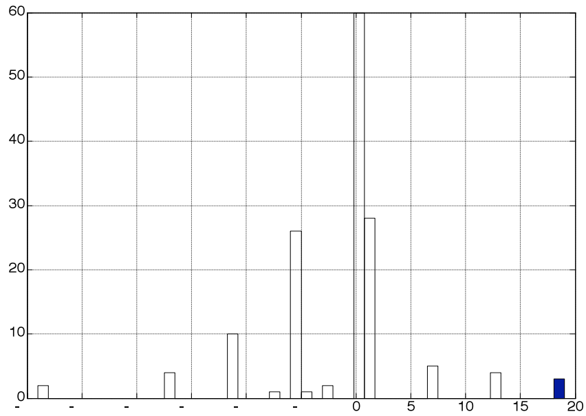
Figure 5-11 Changes on phase 4 (trolley) at 7 th Street
