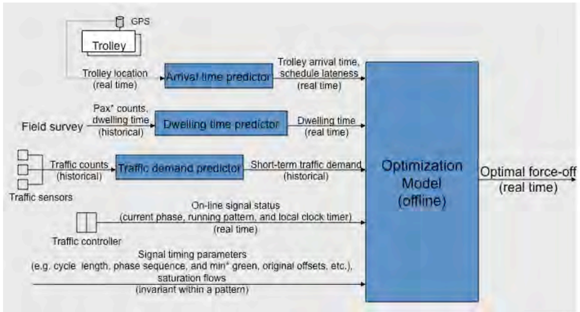
Figure 1-3 Input output diagram for the priority request generator
