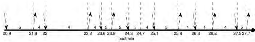
Figure 2.2. Road geometry of I-880N between Decoto Rd. (postmile 20.9) to the south and Winton Ave. (postmile 27.7) to the north. Arrows represent ramp entrance and exit locations, numbers represent the number of lanes on each of the 13 links.
