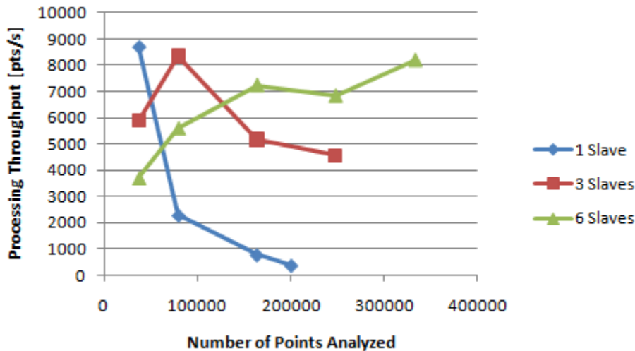
Figure 4.1. Graph of the Processing Throughput on NERSC using the local database on NERSC
