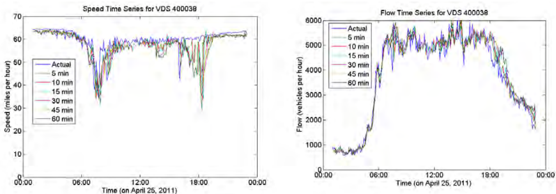
Figure 5.3. Speed and Flow values for VDS 400038. Each line represents a different prediction level.
