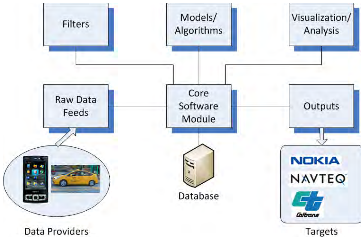
Figure 5.1. Overview of the Mobile Millennium system architecture.
