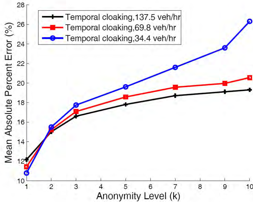
Figure 5.2. Travel Time Accuracy versus Anonymity Level using 10 VTLs/mile.
