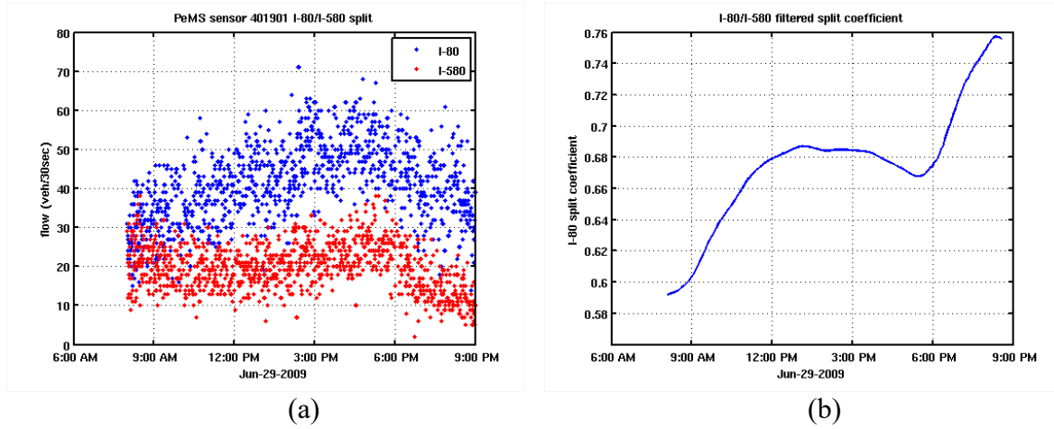
Figure 4.2. (a) Vehicle flows for the I80 – I580 diverge near Berkeley, California, obtained from the PeMS system; (b) filtered time-varying allocation parameter for flow to I80.
