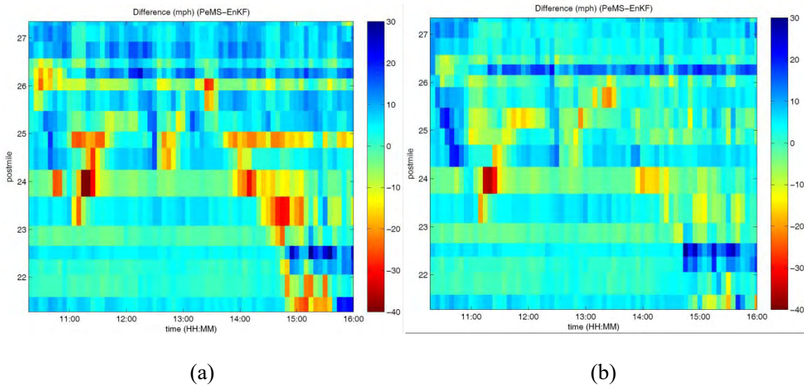
Figure 2.4. PeMS and EnKF CTM-v comparison. Color denotes speed difference between PeMS and EnKF CTM-v with (a) 10 VTLs and (b) 40 VTLs, in mph. Color denotes speed in mph. x -axis: time of day. y -axis: postmile.
