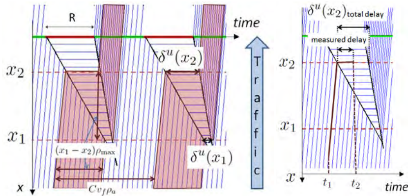
Figure 3.1. (Left) The proportion of delayed vehicles \eta_{x_1, x_2}^u is the ratio between the number of vehicles joining the queue between x_1 and x_2 over the total number of vehicles entering the link in one cycle. The trajectories highlighted in purple represent the trajectories of vehicles delayed between x_1 and x_2 . (Right) The vehicles reporting their location during a stop at x_2 experience a delay \delta \in [0, \delta^u(x_2)] in the time interval [t_1, t_2] . This delay is less than or equal to the total delay ( \delta^u(x_2) ) experienced on the trajectory.
