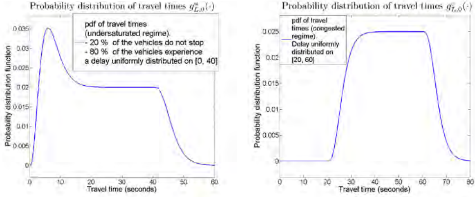
Figure 4.1. Probability distributions of link travel times. Left: Undersaturated regime. The figure represents pdf for a traffic light of duration 40 seconds when 80% of the vehicles stop at the light ( \eta_{L,0}^u = .8 ). Right: Congested regime. The figure represents the pdf for a traffic light of duration 40 seconds when all the vehicles stop in the triangular queue and 50% of the vehicles stop once in the remaining queue. Both figures are produced for a link of length 100 meters. The free flow pace is a random variable with Gamma distribution. The mean free flow pace is 1/15 s/m and the standard deviation is 1/30 s/m. We recall that the probability distribution \gamma of a Gamma random variable x \in \mathbb{R}^+ with shape \alpha and inverse scale parameter \beta is given by \gamma(x) = \frac{\beta^\alpha}{\Gamma(\alpha)} x^{\alpha-1} e^{-\beta x} , where \Gamma is the Gamma function defined on \mathbb{R}^+ and with integral expression \Gamma(x) = \int_0^{+\infty} t^{x-1} e^{-t} dt .
