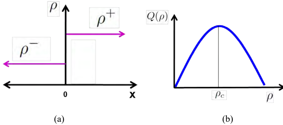
Figure 3.1. (a) Initial data for the Riemann problem; (b) quadratic flux function.
