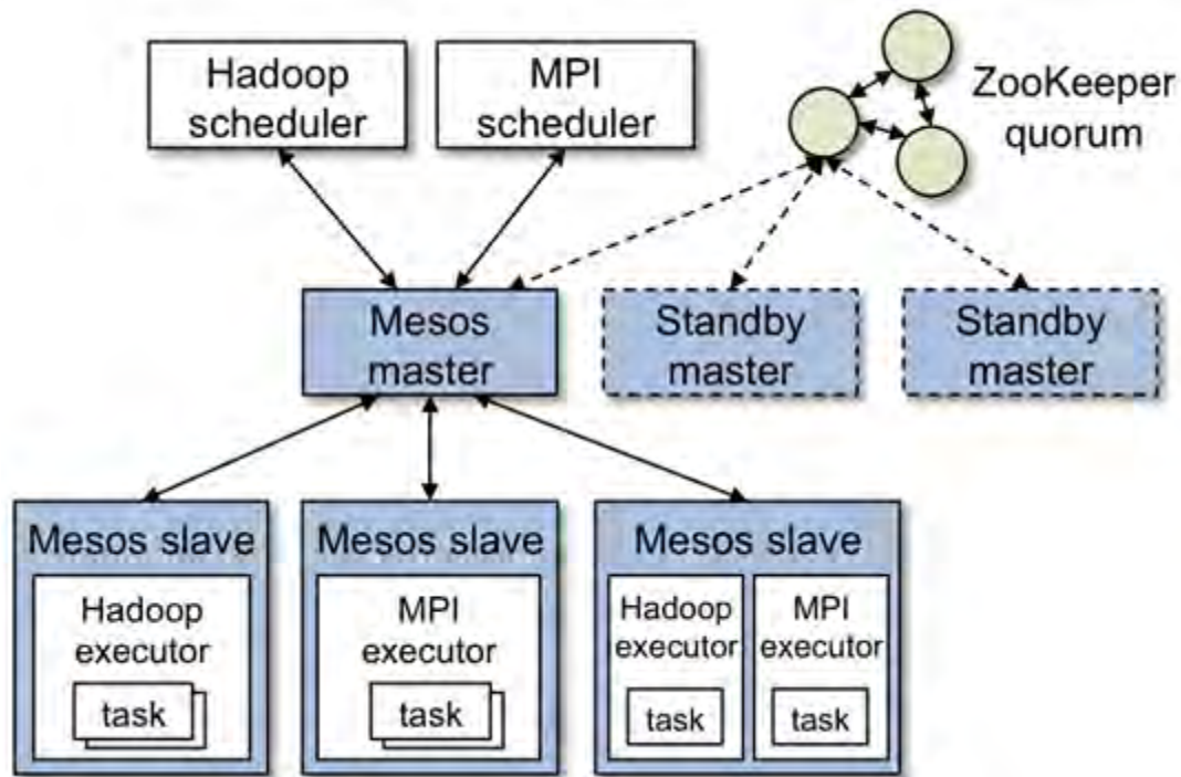
Figure 3.3. Mesos Structure [13]
