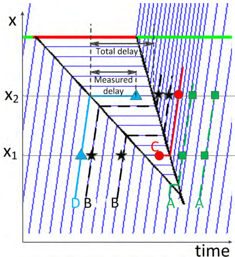
Figure 3.2. Classification of the trajectories depending on the stopping location. We consider vehicles traveling between the two measurement points x_1 and x_2 , sampled uniformly in time.
