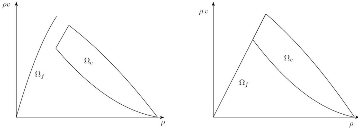
Figure 3.3. Different free-flow phases. Left: Fundamental diagram from the original Colombo phase transition model. Right: Fundamental diagram of the derived model in the particular case of a Newell-Daganzo standard state flux in the congestion phase.
