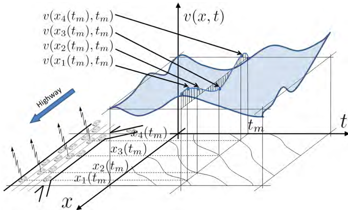
Figure 2.1. Illustration of the distributed velocity field v(x, t) to be reconstructed from GPS samples. Four samples v_i(x_i(t), t) are shown at t = t_m , from vehicles i transmitting their data (indicated by up-arrows above the vehicles).
