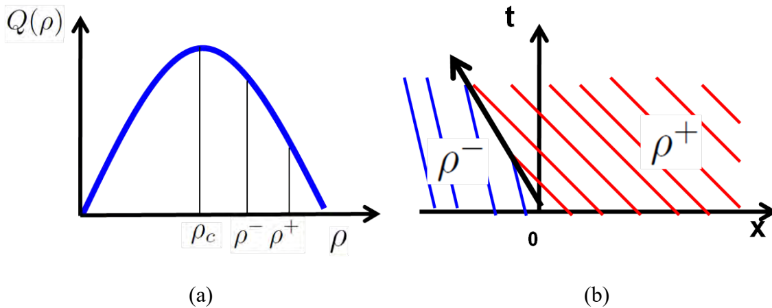
Figure 3.4. Riemann problem solved by a small shock wave moving back. (a) initial data; (b) evolution of the characteristic curves.
