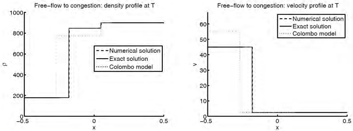
Figure 5.2. Exact solution (continuous line), computed solution (dashed line), and solution to the Colombo model (dotted line) for density (left) and speed (right). Between the two initial states appears a state \mathbf{u}_m = (847.4, -0.24) which corresponds to the intersection of the lower bound of the diagram in congestion with the 2-Lax curve going through \mathbf{u}_r . In this graph T = 1 and \Delta x = 0.0013 .
