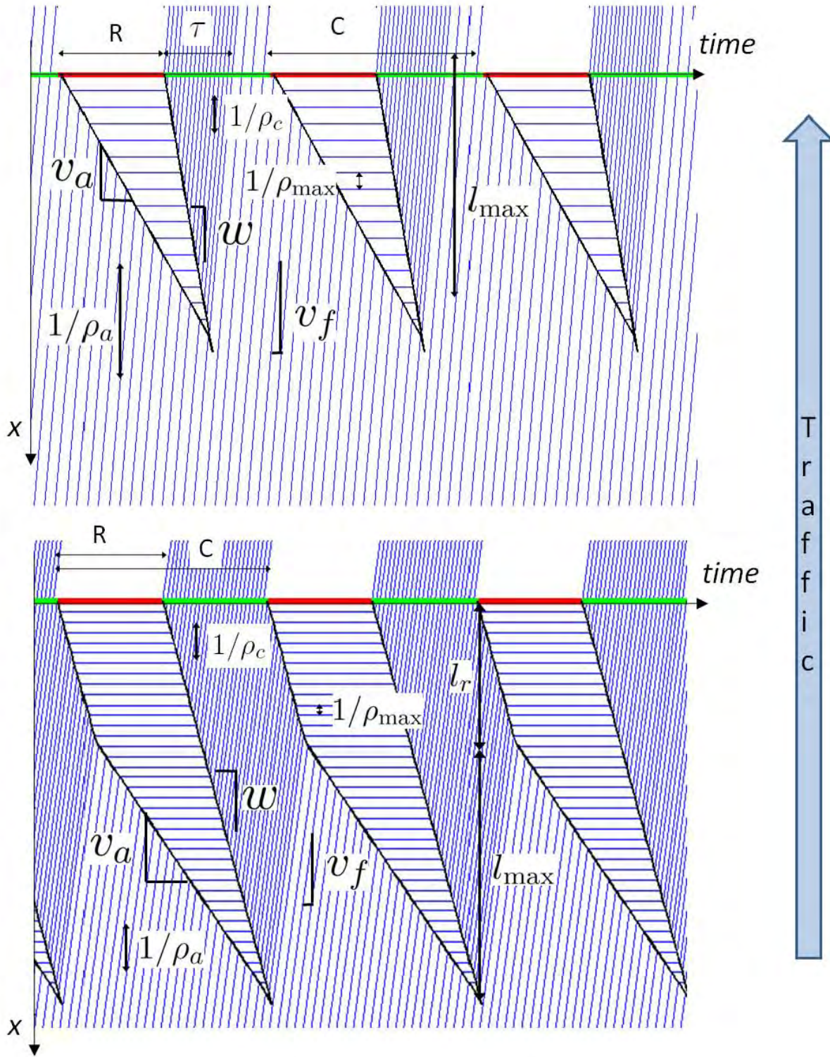
Figure 1.2. Space time diagram of vehicle trajectories with uniform arrivals under an undersaturated traffic regime (top) and a congested traffic regime (bottom).
