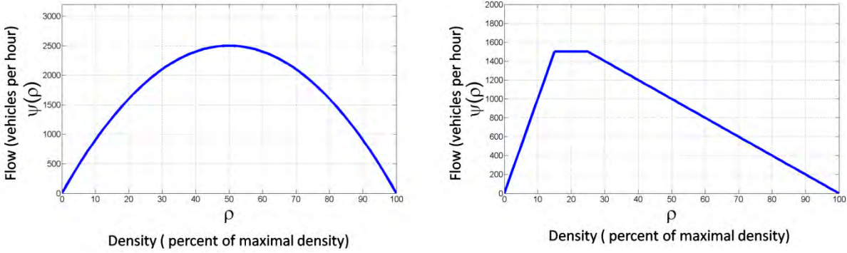
Figure 1.2. Illustration of the Greenshields and trapezoidal Hamiltonians.
