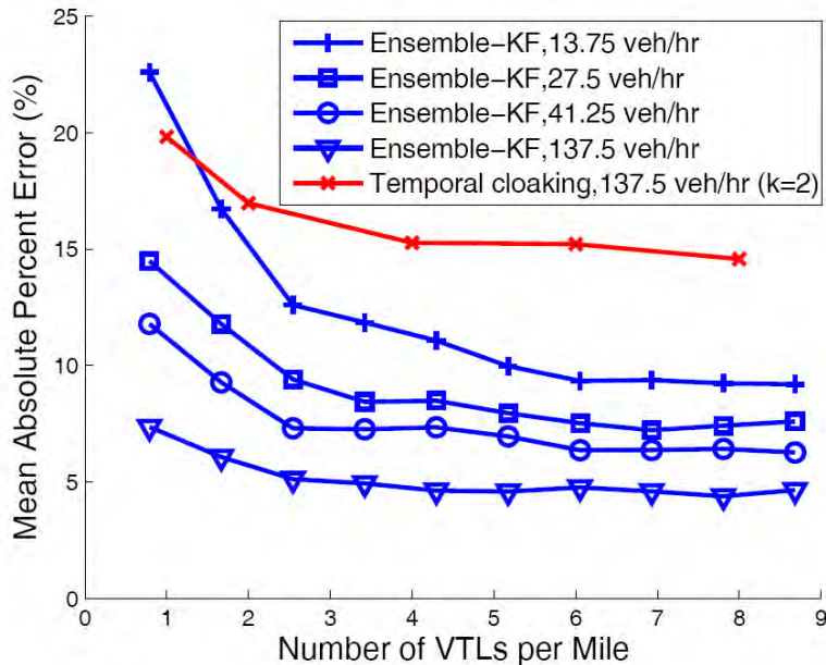
Figure 5.4. Tradeoffs between number of virtual trip lines per mile and the travel time error for different values of the number of equipped vehicles sending measurements per hour.
