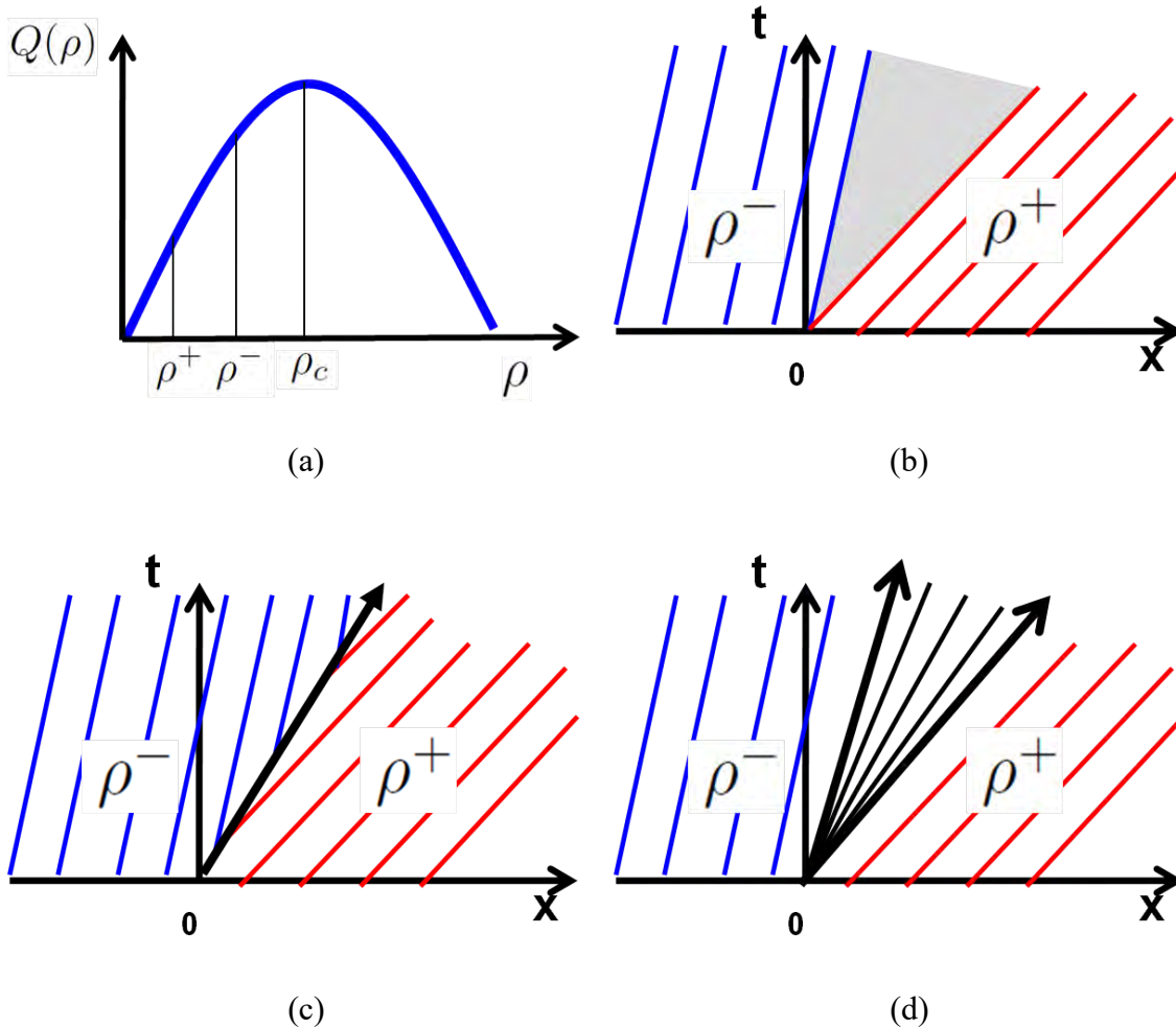
Figure 3.3. Riemann problem solved by a rarefaction wave moving forward. (a) initial data; (b) an envelope appears which is not determined by characteristic curves emanating from the initial data; (c) a weak (but not entropy admissible) evolution of the characteristic curves; (d) entropy admissible evolution of the characteristic curves.
