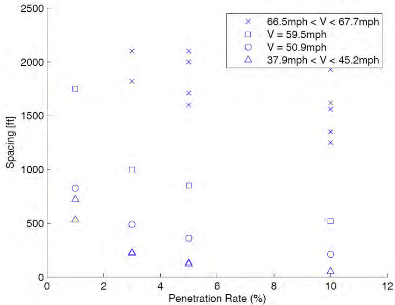
Figure 4.2. Minimum Spacing Constraints for Straight Highway Section.
