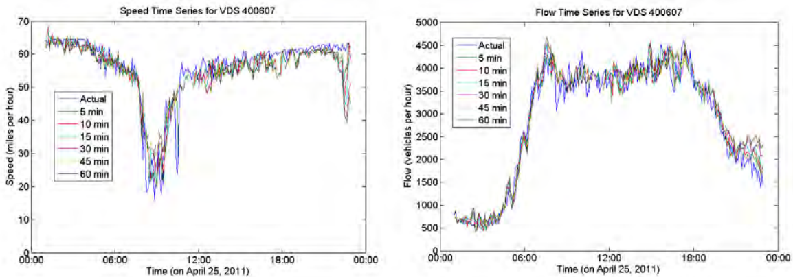
Figure 5.4. Speed and Flow values for VDS 400607. Each line represents a different prediction level.
