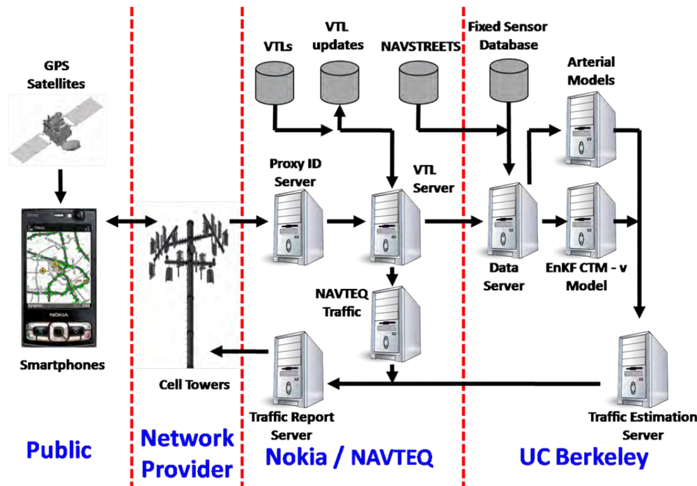
Figure 1.1. Mobile Millennium System Architecture (Nokia and Berkeley)
