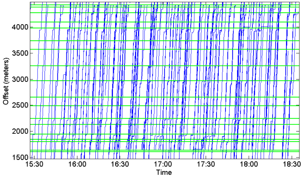
Figure 1.3. Vehicle trajectories from the Mobile Millennium evaluation experiment on San Pablo Avenue in Berkeley, Albany and El Cerrito, California. The high-frequency GPS data in this figure is represented as distance (meters) from an arbitrary start point upstream of the experiment location. The horizontal lines represent the locations of the traffic signals along the route.
