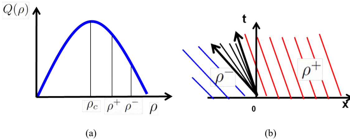
Figure 3.5. Riemann problem solved by a rarefaction wave moving back. (a) initial data; (b) evolution of the characteristic curves.
