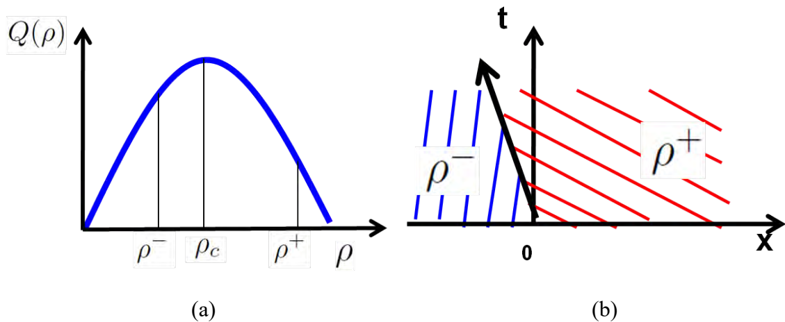
Figure 3.7. Riemann problem solved by a big shock moving back. (a) initial data; (b) evolution of the characteristic curves.
