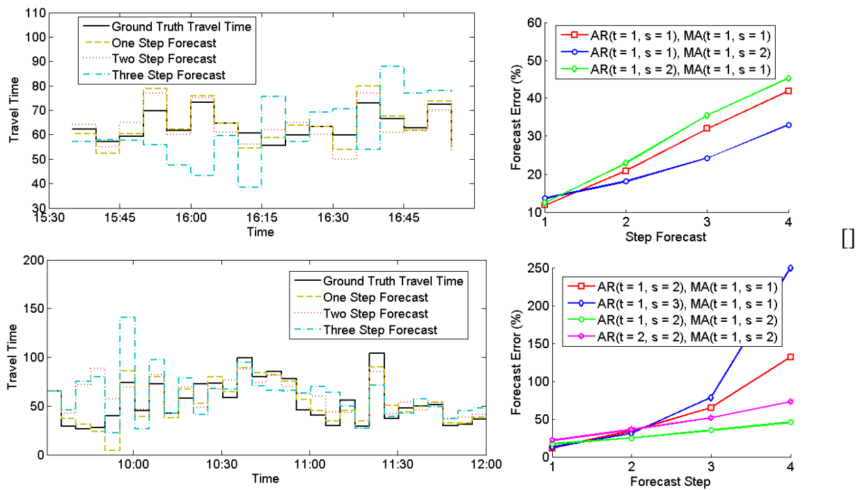
Figure 1.6. Forecast accuracy. (a) and (c): Forecast error for a VTL pair in the Paramics and New York networks, respectively. (b) and (d): Average forecast error as a function of the number of forecast steps into the future, Paramics and New York networks, respectively. One step is 5 minutes. In (b) and (d), t represents the temporal dependency and s represents the spatial dependency.
