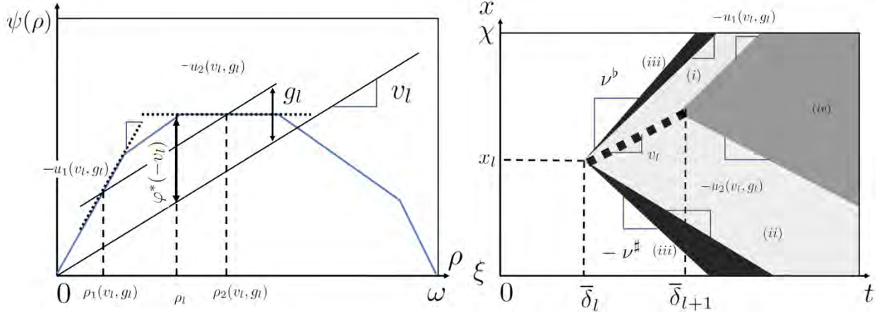
Figure 5.4. Construction of the solution associated with an affine internal condition.
