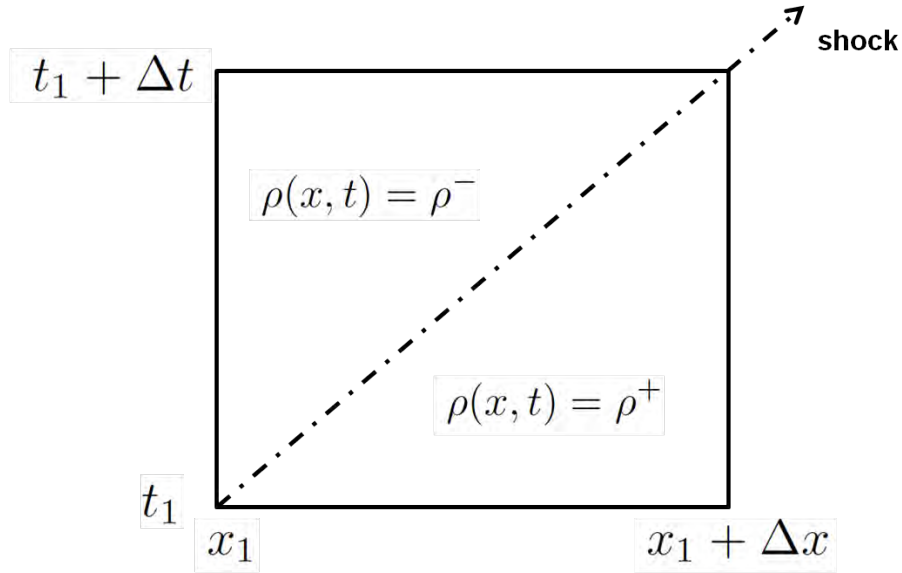
Figure 1.2. A shock traveling at speed S connects the states \rho^- and \rho^+ over a small interval x \in [x_1, x_1 + \Delta x] in space and t \in [t_1, t_1 + \Delta t] in time.
