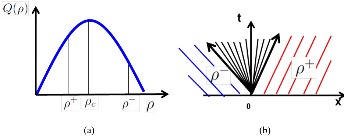
Figure 3.6. Riemann problem solved by a rarefaction wave moving back and forward. (a) initial data; (b) evolution of the characteristic curves.
