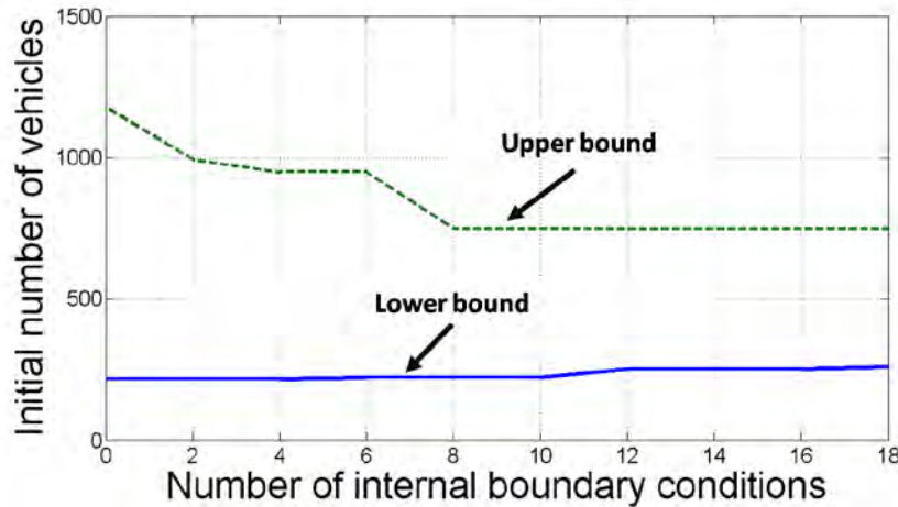
Figure 5.1. Initial number of vehicles estimation using linear programming.
