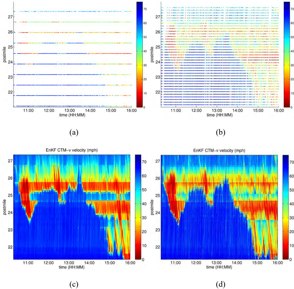
Figure 2.3. VTL measurements with (a) 10 VTLs and (b) 40 VTLs, and EnKF CTM-v velocity contour plots with (c) 10 VTLs and (d) with 40 VTLs. Color denotes speed in mph. x -axis: time of day. y -axis: postmile. The congestion resulting from the morning accident also highlights some of the differences between the EnKF CTM-v estimates created with 10 VTLs and 40 VTLs. Because the model does not predict accidents, measurements are needed to drive the ensemble states into congestion. Because the congestion is recorded on VTLs earlier and more frequently than with the coarser VTL spacing, the ensembles converge to the slower state more quickly. Additionally, because the congested state is slower, the difference in fluxes surrounding the discontinuity is increased, which in turn causes the shockwave speed to increase. Particularly around postmile 25, the decrease in velocity from the shockwave causes the difference between PeMS and EnKF CTM-v velocity measurements to increase with additional VTLs (Figure 2.4(a)–2.4(b)).
