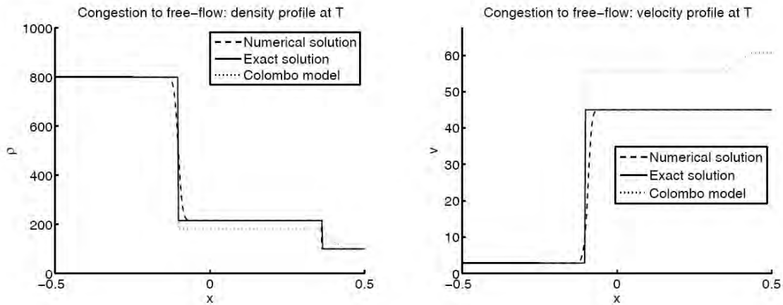
Figure 4.1. Exact solution (continuous line), computed solution (dashed line), and exact solution for the Colombo model (dotted line) for density (left) and speed (right). Between the two initial states, for the class of models presented here, appears a state u_m = (215.4, -0.03) which corresponds to the intersection of the 1-Lax curve going through u_l with the metastable phase. In this graph T = 0.4 and \Delta x = 0.0013 .
