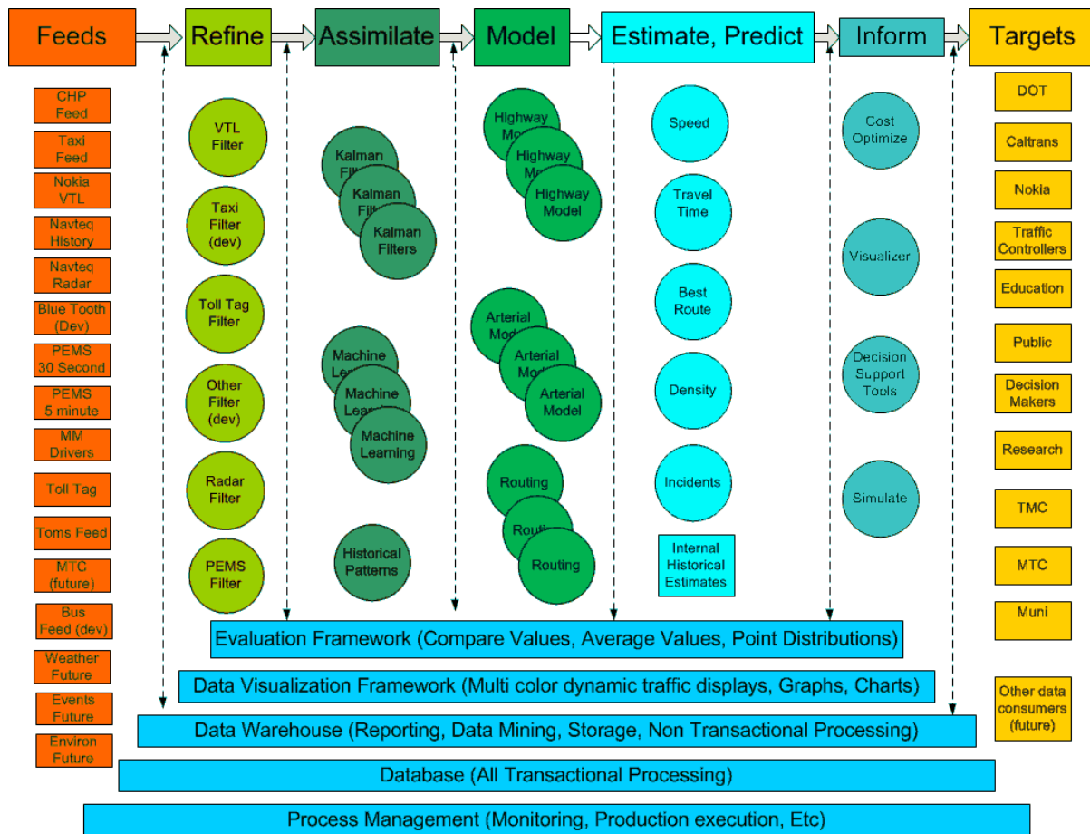
Figure 1.3. Mid-project Mobile Millennium based traffic data collection and processing system
