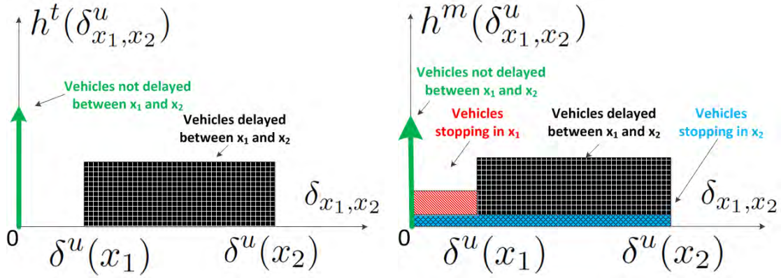
Figure 3.3. (Left) Probability distribution of the total delay between x_1 and x_2 in the undersaturated regime. (Right) Probability distribution of the measured delay between x_1 and x_2 in the undersaturated regime. Vehicles are assumed to be sampled uniformly in time.
