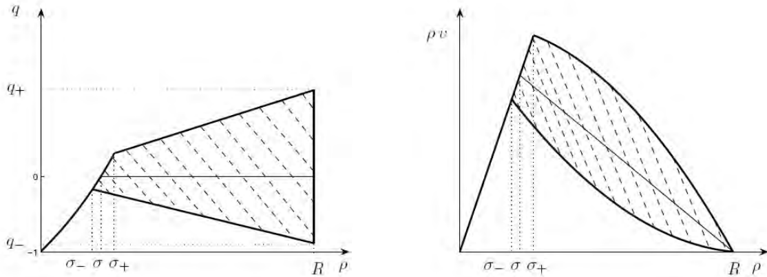
Figure 3.2. Newell-Daganzo standard flux function. Left: Fundamental diagram in state space coordinates. Right: Fundamental diagram in flux-density coordinates. The standard state is the usual triangular diagram. The congestion phase is two-dimensional (striped domain).
