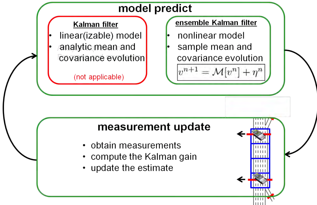
Figure 1.1. Illustration of the difference between extended Kalman filtering and ensemble Kalman filtering, and the iterative process predict–update.
