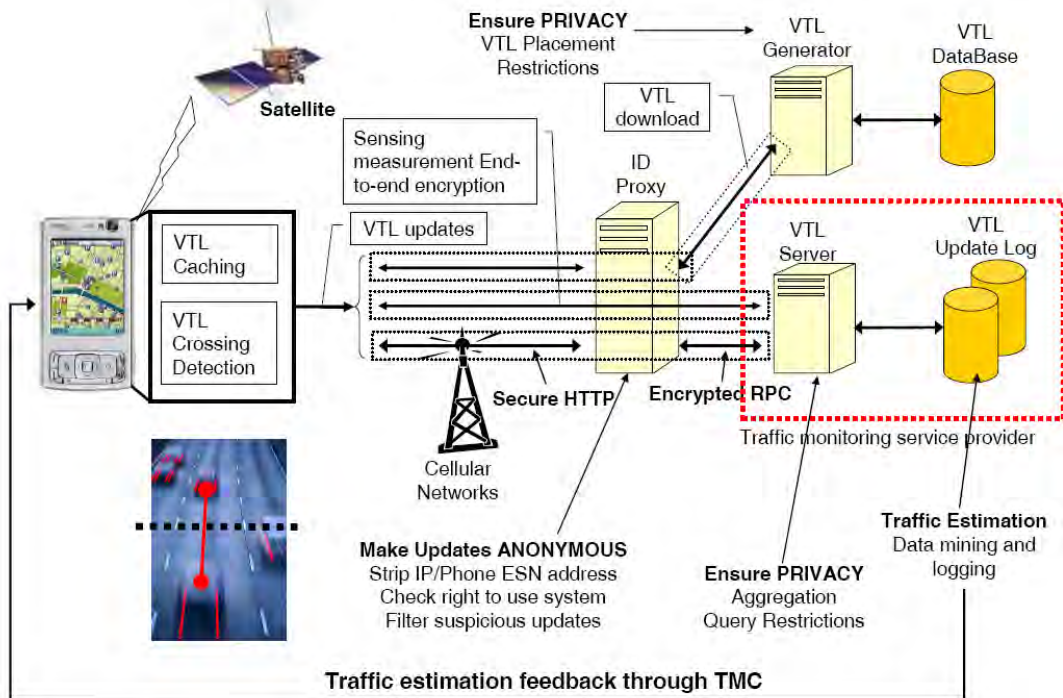
Figure 3.1. Virtual Trip Line: Privacy-Preserving Traffic monitoring System Architecture.
