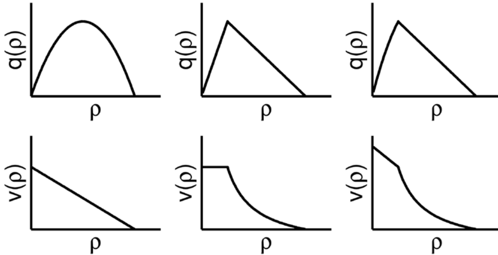
Figure 1.1. Fundamental diagrams (top row) and velocity functions (bottom row) for Greenshields (left), Daganzo-Newell (center), and Smulders (right).
