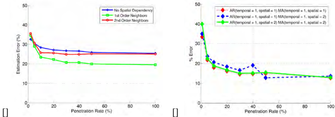
Figure 1.5. Average one-step forecast error vs. penetration rate for all VTL pairs in the Paramics dataset. (a) Logistic Regression Forecast Classification Error. (b) STARMA Travel Time Forecast Error.
