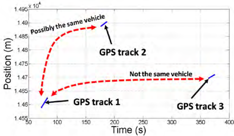
Figure 7.4. Vehicle reidentification using linear programming.
