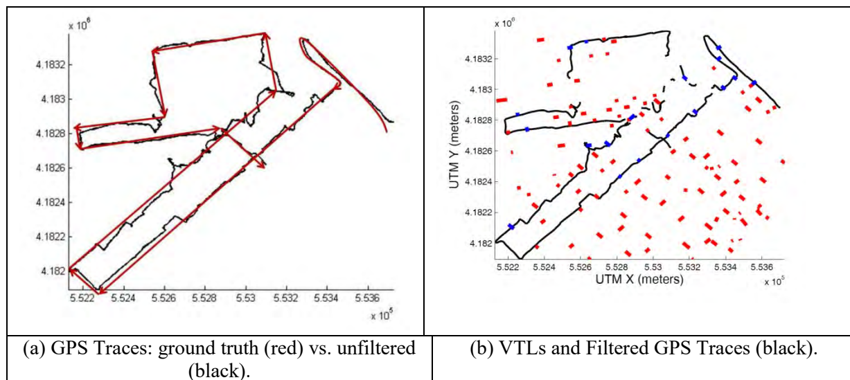
Figure 5.1. In the right figure, red colored lines denote VTLs placed in downtown while blue lines denote detected VTL crossings.
