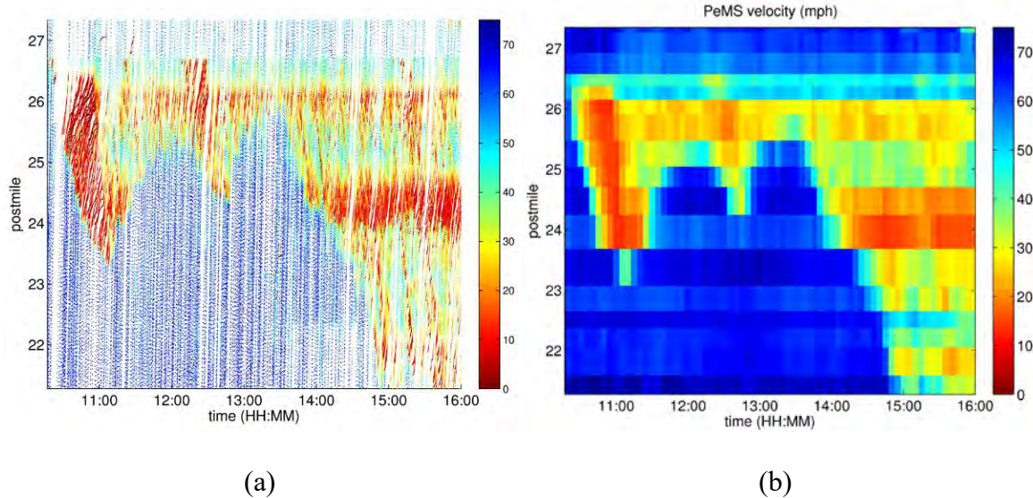
Figure 2.1. I-880N experiment data. (a) Vehicle GPS logs stored locally on the phone. (b) PeMS velocity contour plot. Color denotes speed in mph. x -axis: time of day. y -axis: postmile.
