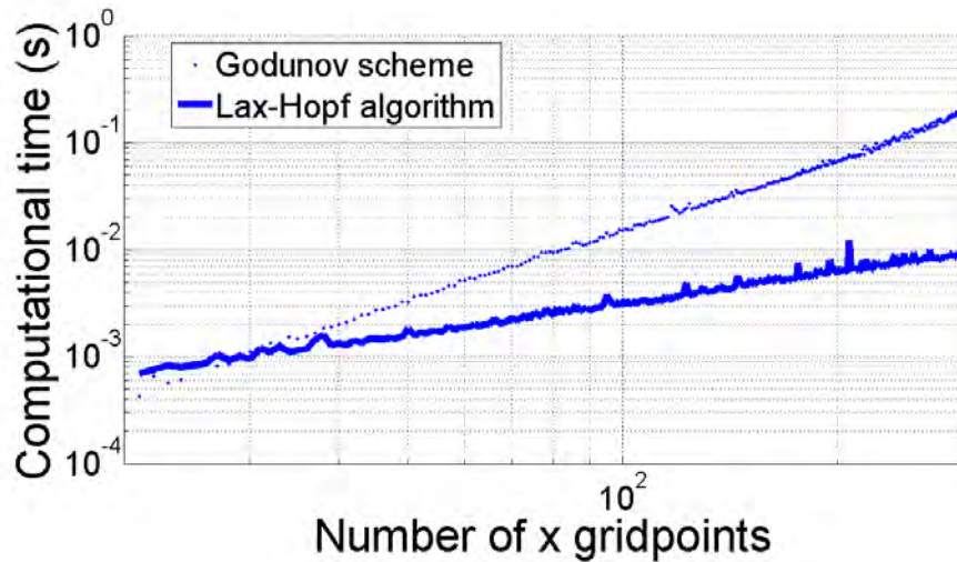
Figure 8.3. Computational time comparison between the Lax-Hopf algorithm and the Godunov scheme (287).
