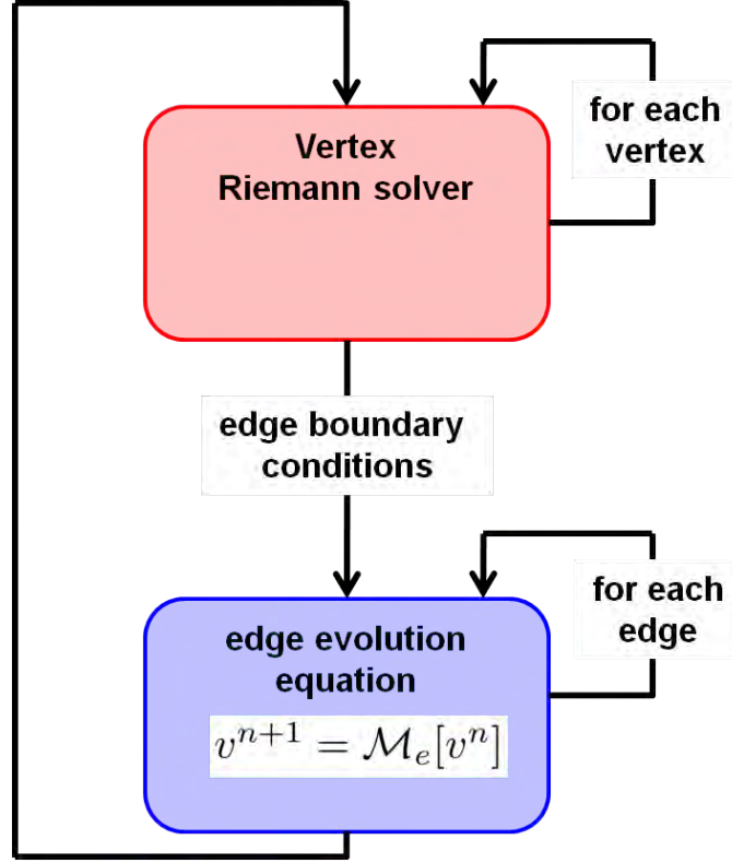
Figure 4.3. The discrete network velocity evolution equation proceeds in two steps. First, the Riemann problem at each vertex is solved to determine the strong boundary conditions for each edge. Then, for each edge the velocity is evolved according to (50).
