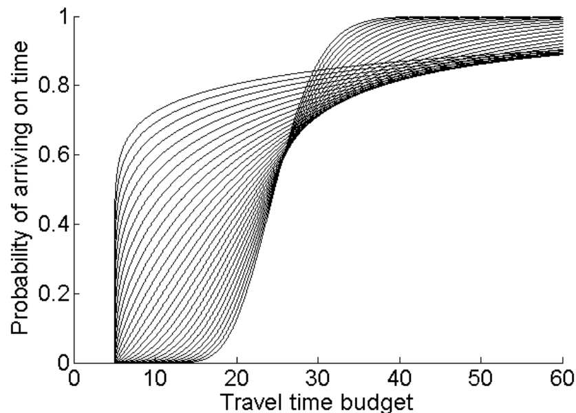
Figure 5.6. A family of travel-times distributions modeled using 30 shifted gamma distributions, each with the same mean travel time of 25 minutes and a minimum travel time of 5 minutes. The shape parameter of the distributions ranges from 4 to 0.13 and the scale parameter of the distributions ranges from 5 to 150. The SOTA policy will be the upper envelope of all the curves. The LET path could be any of the curves and in the worst case even be the path that minimizes the probability of arriving on time for a given budget.
