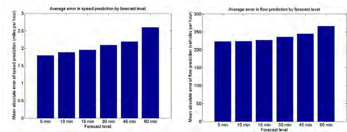
Figure 5.1. Average speed and flow errors by prediction level.
