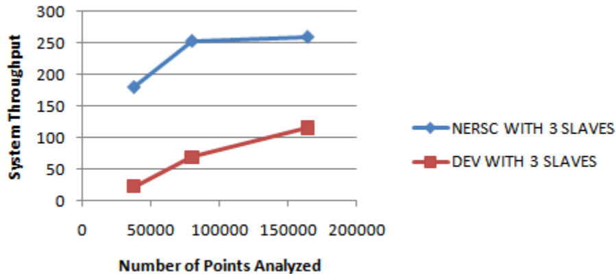
Figure 4.4. Graph of the System Throughput on NERSC using different DBs
