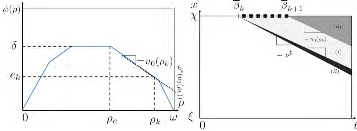
Figure 5.3. Construction of the solution associated with an affine downstream boundary condition.
