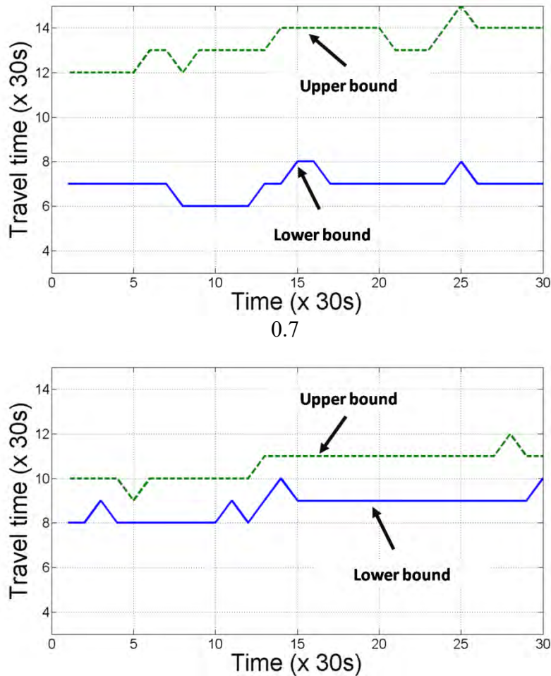
Figure 5.2. Travel time estimation using linear programming.
