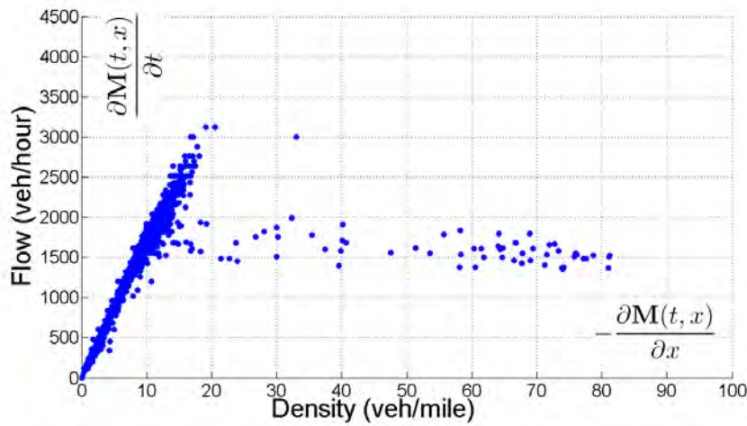
Figure 1.1. Illustration of the flow-density relationship.
