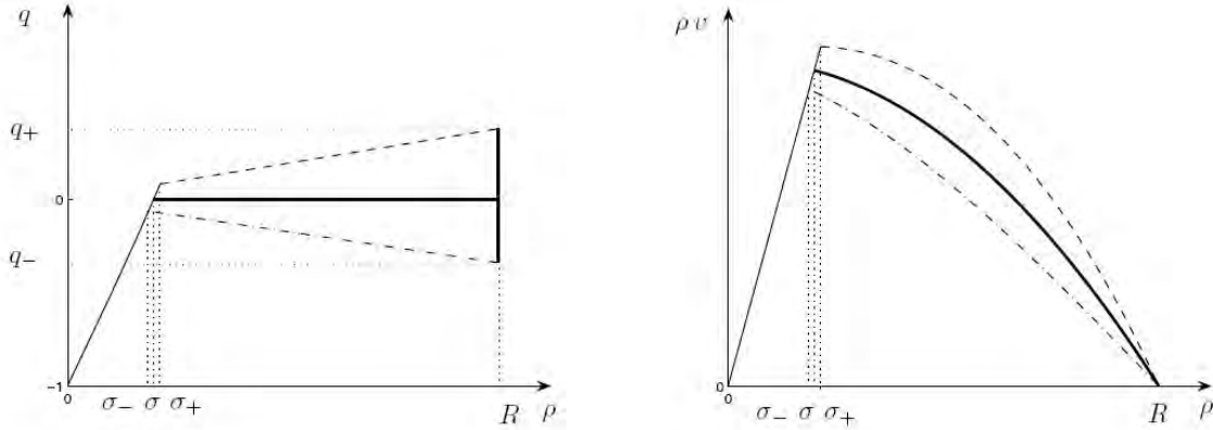
Figure 5.1. Phase transition model with a Greenshields standard state. Left: State-space coordinates. Right: Flux-density coordinates. Thin solid line: Free-flow. Bold solid line: Congestion standard state. Thin dashed line: Upper bound of congestion. Thin dot-dashed line: Lower bound of congestion. The standard flux is concave, and all the 1-Lax curves are concave in (\rho, \rho v) coordinates. In (\rho, q) coordinates the free-flow phase is not a straight line but has a very light convexity.
