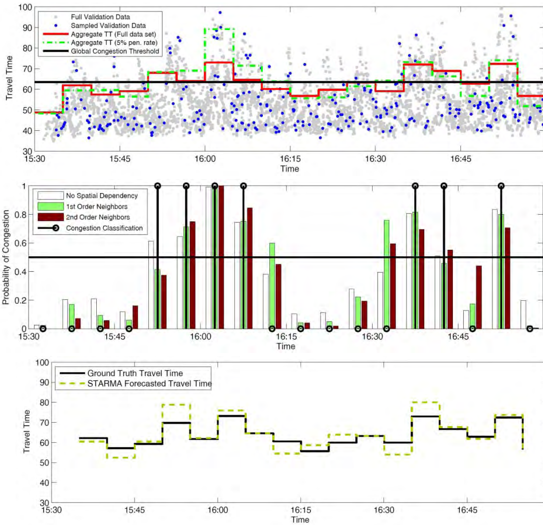
Figure 1.3. One-step forecast validation results on a given VTL pair of the Paramics simulation network (penetration rate: 5%). (a) Travel time data of the VTL pair and its aggregate value on 5-minute intervals. Both the data and the aggregate value are shown for the whole data set and for a 5% penetration rate. (b) Onestep forecast of the congestion state produced by the logistic regression algorithm. The bars represent the probability of congestion estimated by the models for different levels of spatial dependency. The real state of congestion is represented with circles. (c) One-step forecast of travel time produced by the STARMA algorithm.
