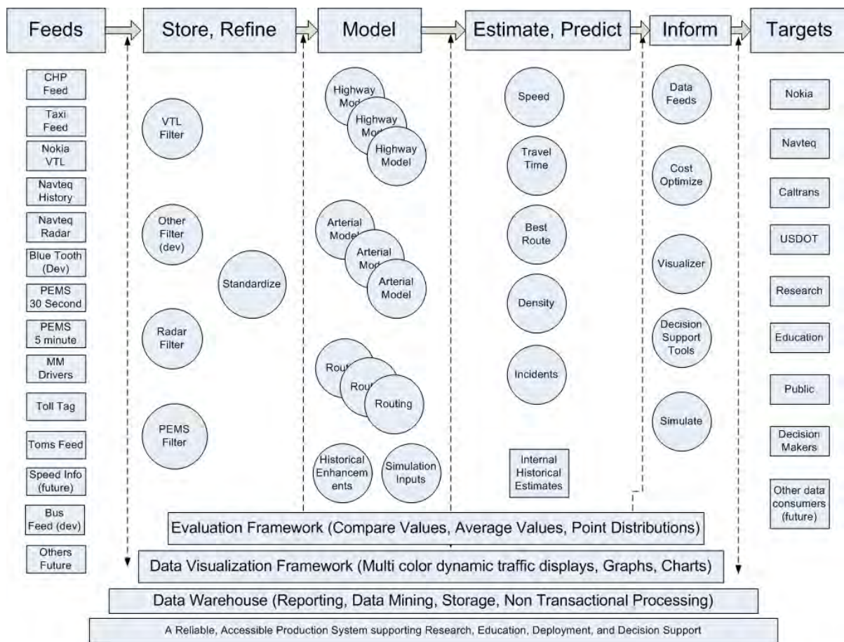
Figure 3.2. An overview of the Mobile Millennium system.
