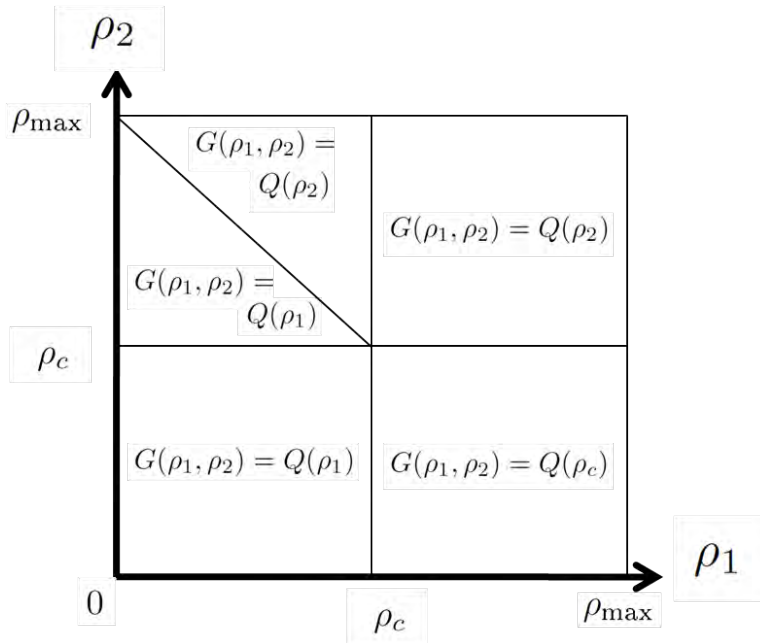
Figure 4.1. Graphical representation of the numerical flux function equation (32) as a function of \rho_1 and \rho_2 . Note that the line connecting (\rho_c, \rho_c) and (0, \rho_{\max}) may have different shapes depending on the flux function Q(\cdot) .
