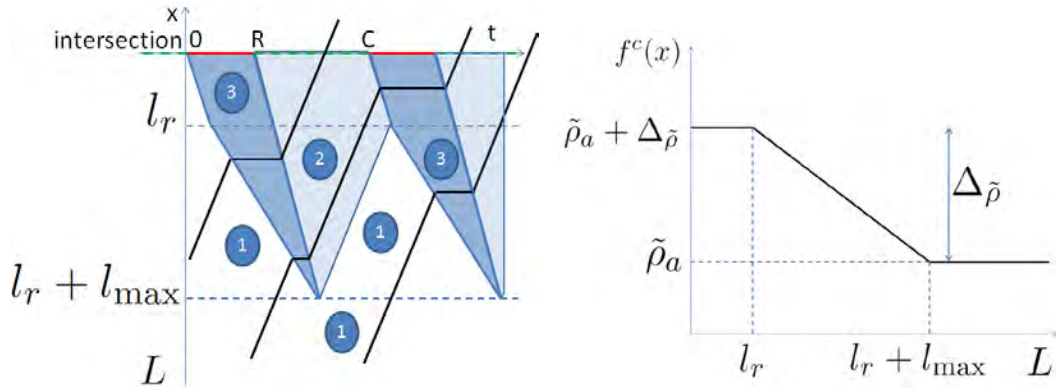
Figure 2.1. Left: The estimation of vehicle spatial distribution on a link is derived from the queue dynamics of the traffic flow model. The space-time plane represents the space-time domain in which density of vehicles is constant. Domain 1 represents the arrival density \rho_a , domain 2 represents the critical density \rho_c and domain 3 represents the maximum density \rho_{\max} . Right: Using the stationarity assumption, we compute the average density at location x and normalize to derive the probability distribution of vehicle locations on the link.
