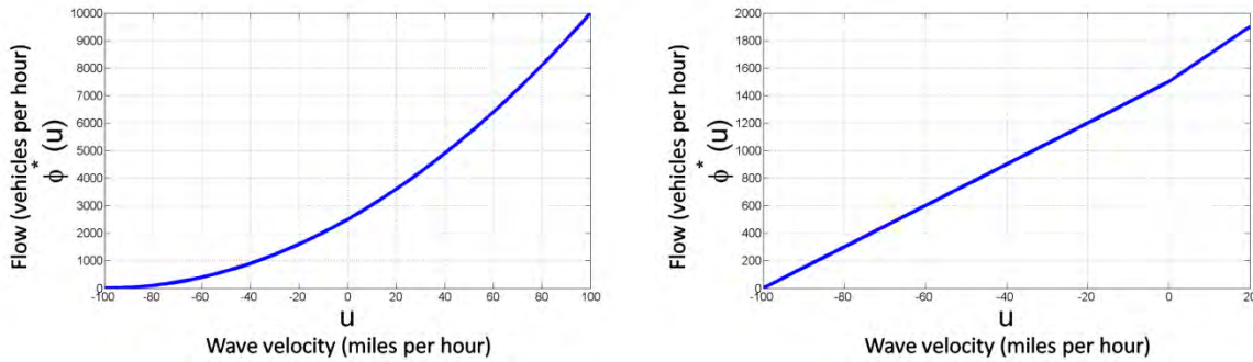
Figure 3.1. Illustration of the convex transforms associated with the Greenshields and trapezoidal Hamiltonians.
