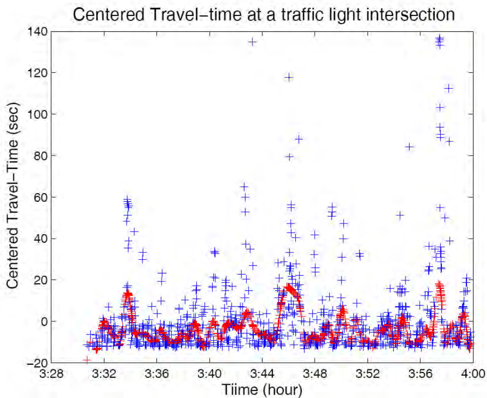
Figure 4.1. Observed travel-times (blue sparse points) and estimated travel-times (red smooth curve) for a linear combination of a gaussian kernel (with \sigma = 100 ) and a linear kernel.
