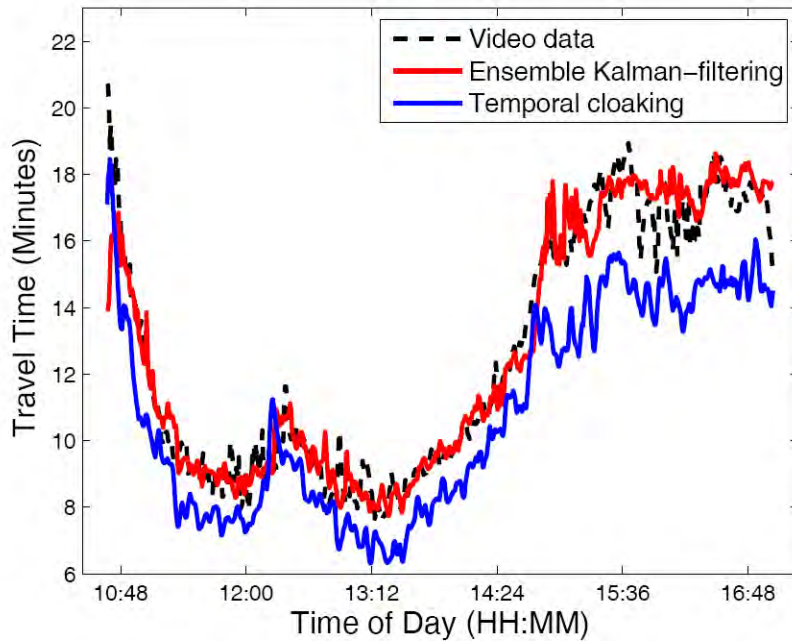
Figure 5.5. Comparison between mean travel time obtained from video data, mean travel time obtained from temporal cloaking, and mean travel time obtained from the accuracy centric architecture.
