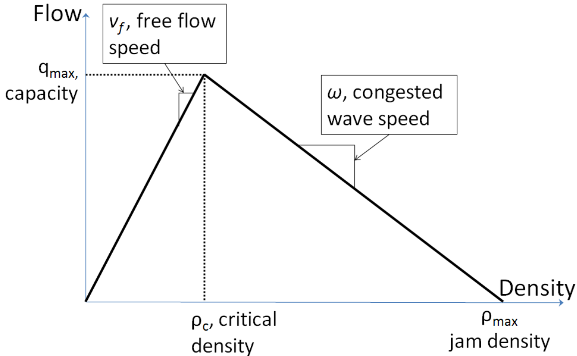
Figure 1.1. The fundamental diagram: empirically constructed relation between flow and density of vehicles.
