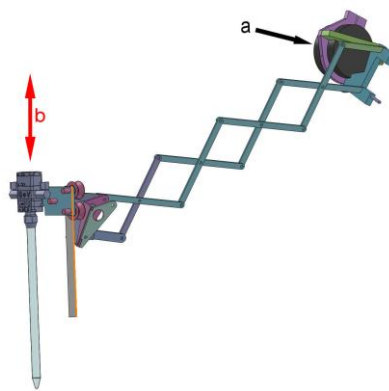
Figure 41. Injection Linkage
