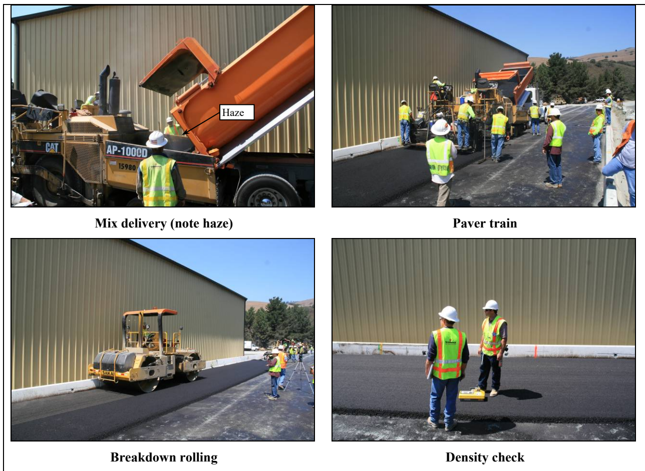
Figure 2.29: Control: Placement of first lift of asphalt concrete.
