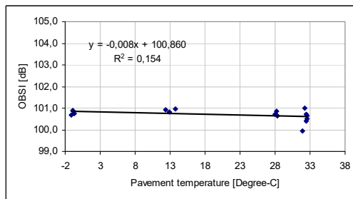
Figure 4.14. RAC-O pavement eastbound to the left and westbound to the right. Normalized OBSI noise measurement results with SRTT versus pavement temperature.
