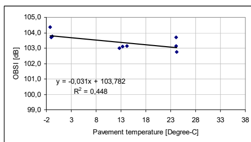
Figure 4.16. DGAC pavement westbound. Normalized OBSI noise measurement results with SRTT versus pavement temperature.
