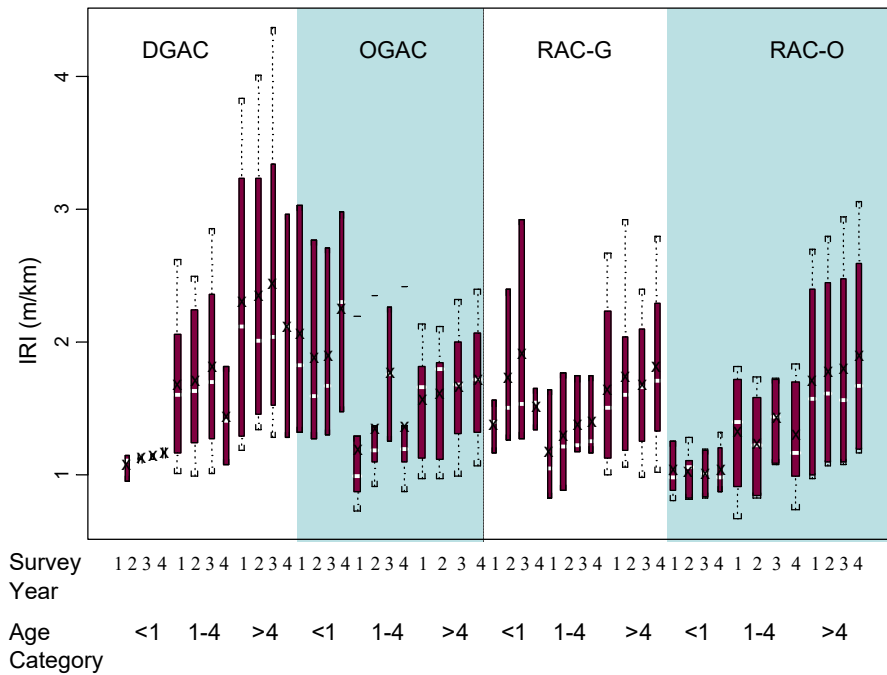
Figure A.3: Comparison of IRI values for different mix types at different ages for four years of data collection. (Note: 1 m/km = 63 in./mi; 2 m/km = 127 in./mi; 3 m/km = 190 in./mi)
