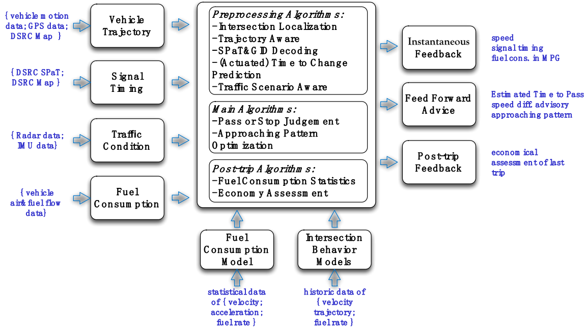
Fig. 3.1 Architecture of algorithm
