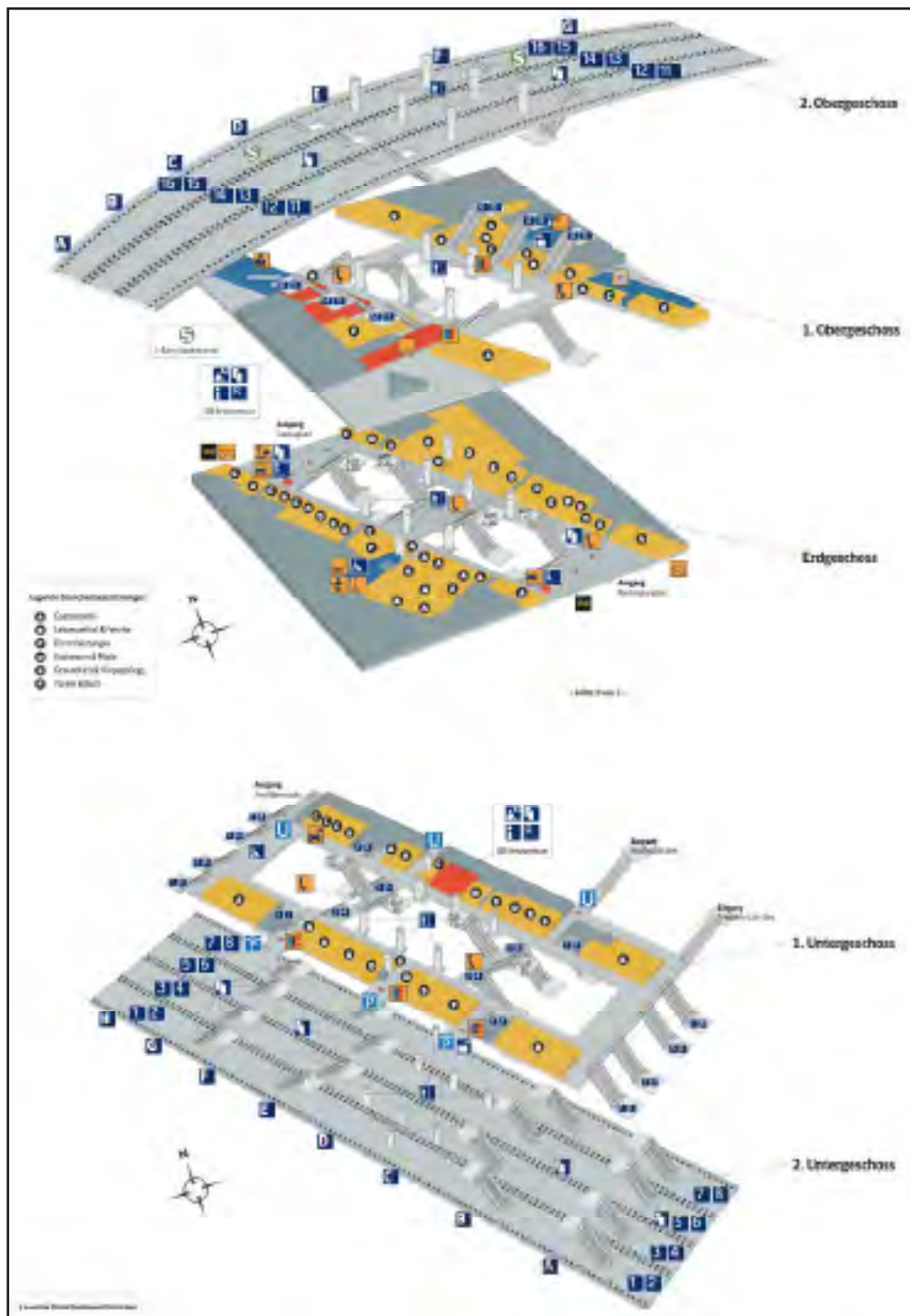
Figure 32. Berlin Central Station Layout
