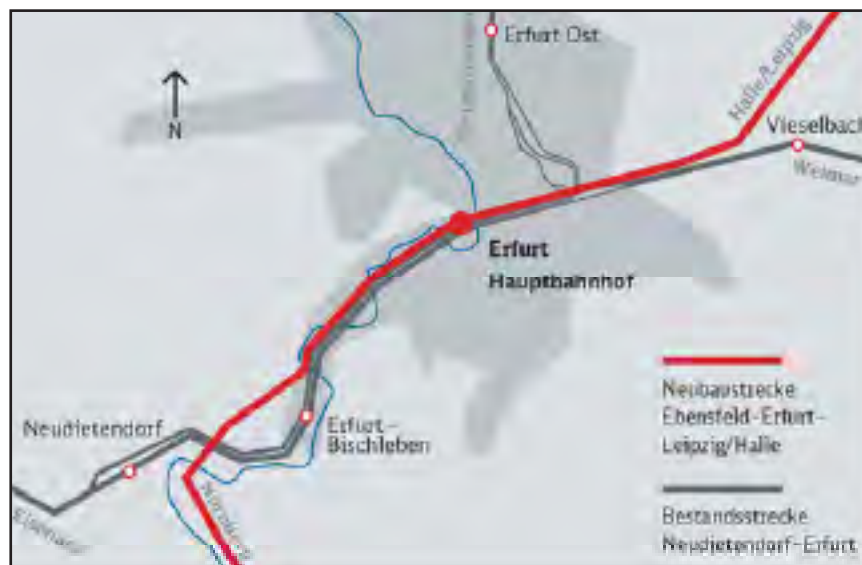
Figure 57. The New High-Speed Corridor's Alignment through Erfurt Main Station
