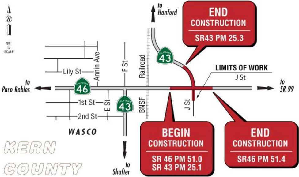
Wasco State Route 43/State Route 46 Intersection Improvements
