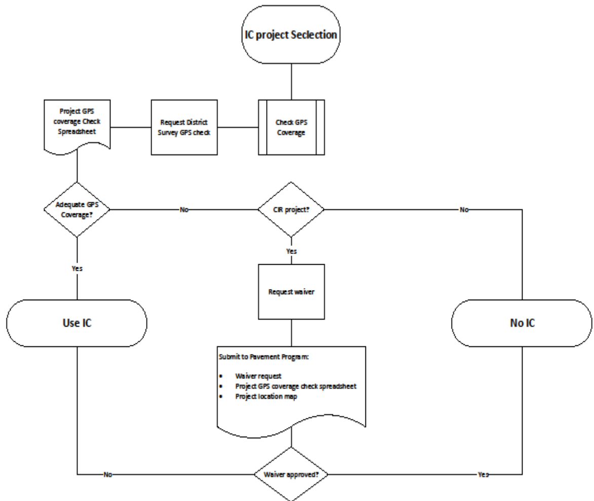
Figure 1- IC project selection GPS coverage Criteria
