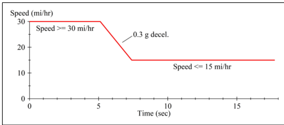
Figure 3. Speed profiles, braking event (section a) (time vs. speed)
