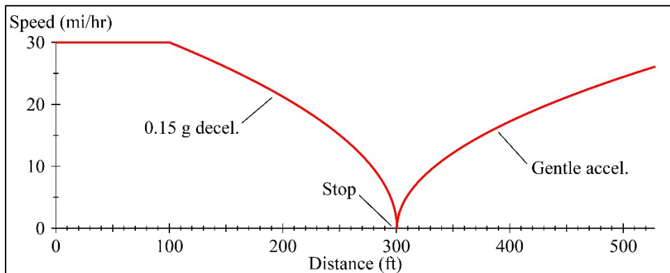
Figure 5. Speed profiles, braking event (section b) (distance vs. speed)
