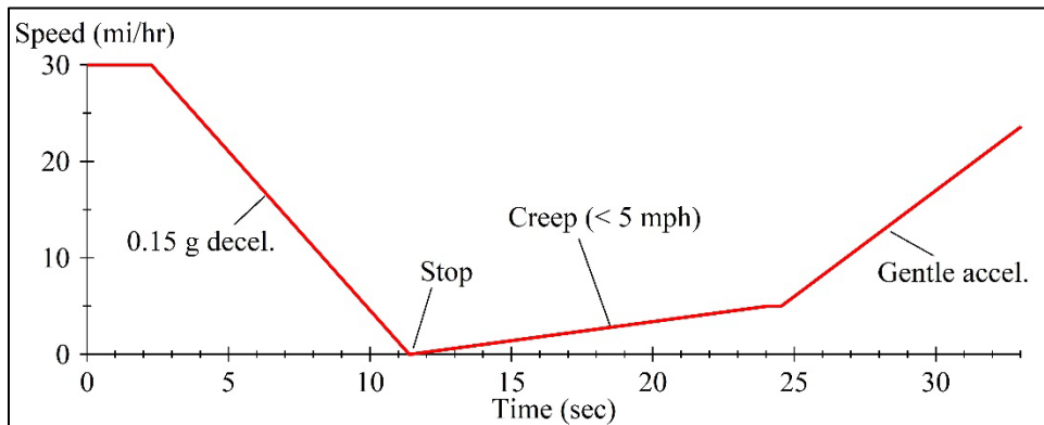
Figure 6. Speed profiles, braking event (section c) (time vs. speed)
