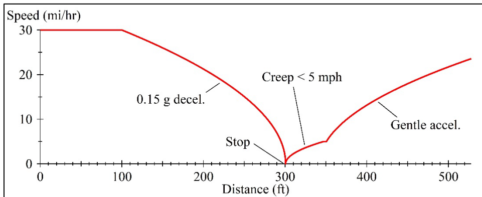
Figure 7. Speed profiles, braking event (section c) (distance vs. speed)
