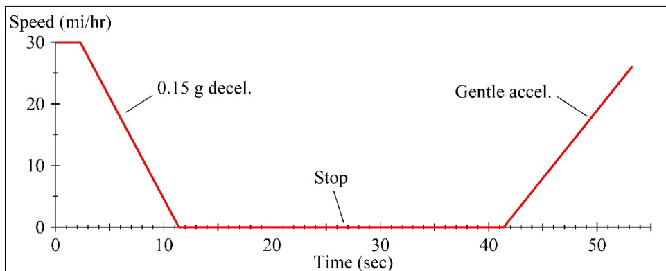
Figure 4. Speed profiles, braking event (section b) (time vs. speed)
