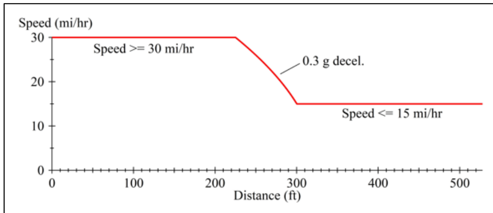
Figure 2. Speed profiles, braking event (section a) (distance vs. speed)
