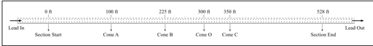
Figure 1. Cone layout 528 ft test section
