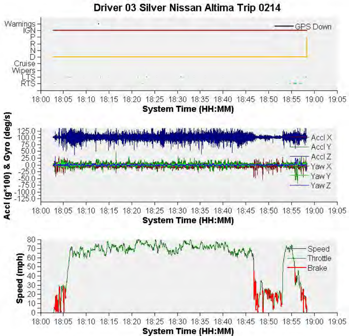
Figure 3.5: Plot Of Key Vehicle Parameters Collected During A Trip.
