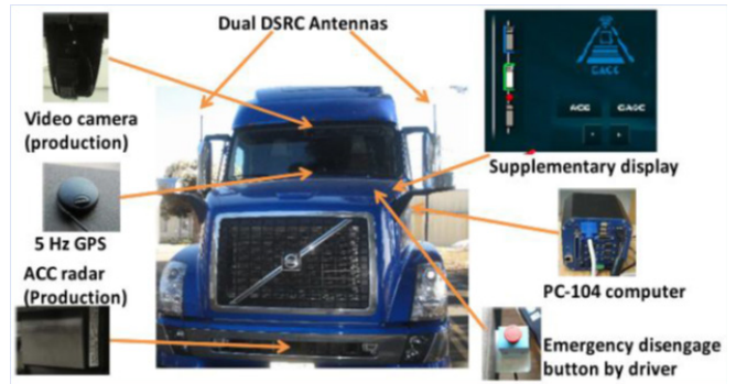
Image 1: Overall Cooperative Adaptive Cruise Control (CACC) Systems Components
