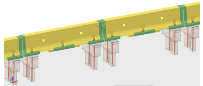
Image 3: Test 616811-01-3 Asphalt Median Configuration 2023_01_19
