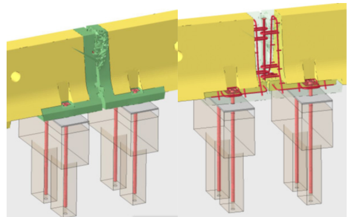
Image 4: Pooled Fund Example Project: Portable Temporary F Shape Concrete Barrier with vertical anchorage Finite Element Model and Simulation Results
