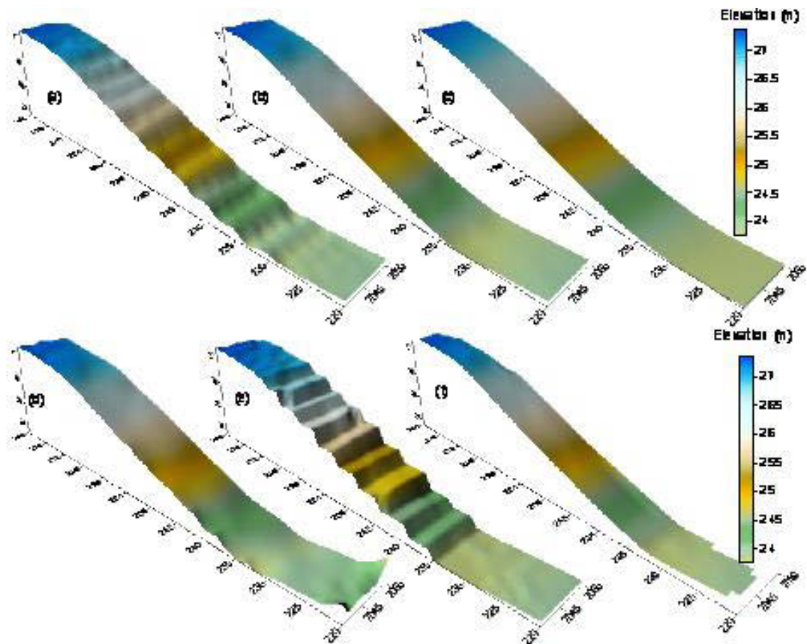
DTMs of a 540m 2 Area using 78 Elevation Data Points using Different Interpolation Methods: (a) Inverse Distance to a Power; (b) Kriging; (c) Local Polynomial; (d) Minimum Curvature; (e) Nearest Neighbor; (f) Triangulated Irregular Network (TIN)
