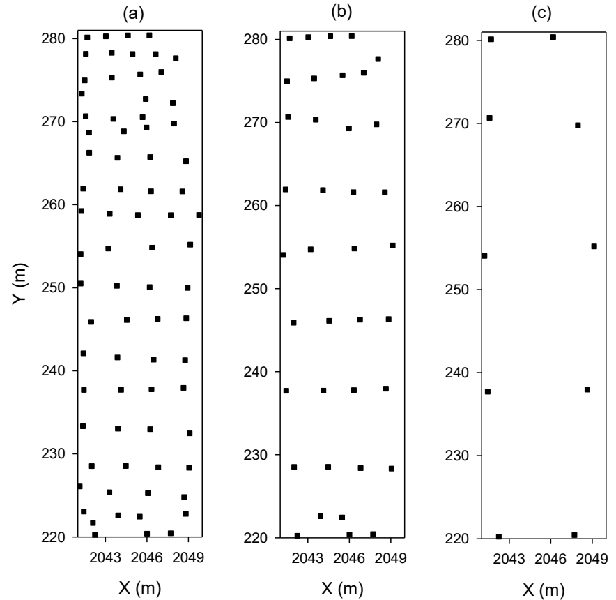
Elevation Data points for Developing DTM over a 540 m 2 Area: (a) 78 Data Points; (b) 38 Data Points; and (c) 11 Data Points
