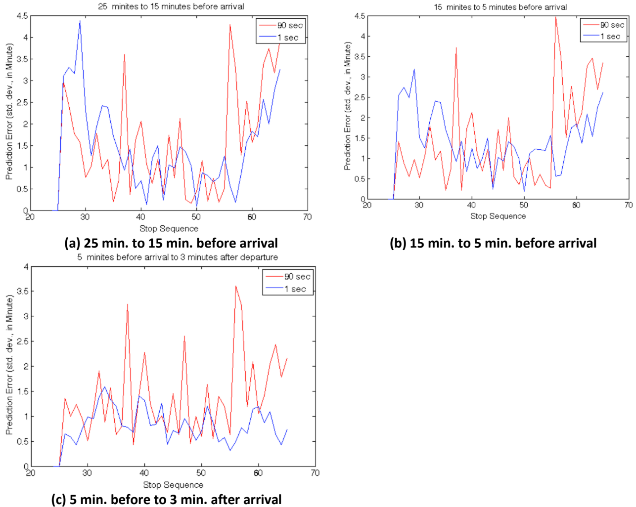
Figure 4-27 Prediction errors of RT location data based PTA for 90 sec. versus 1 sec. update rate
