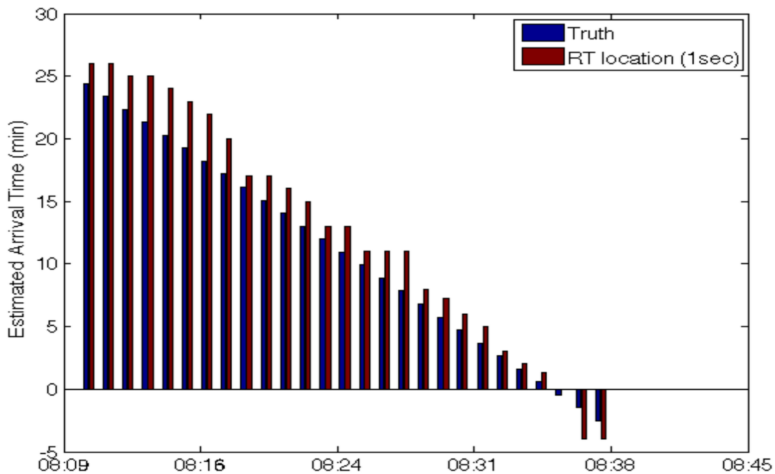
Figure 4-25 Differences of PTA between the real-time location based prediction and the truth
