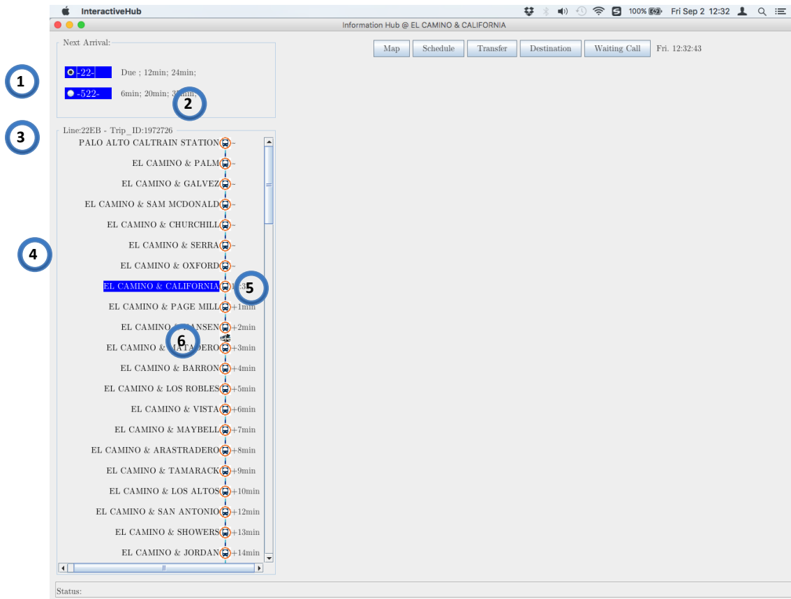
Figure 4-5 Basic Interface Frame (a)
