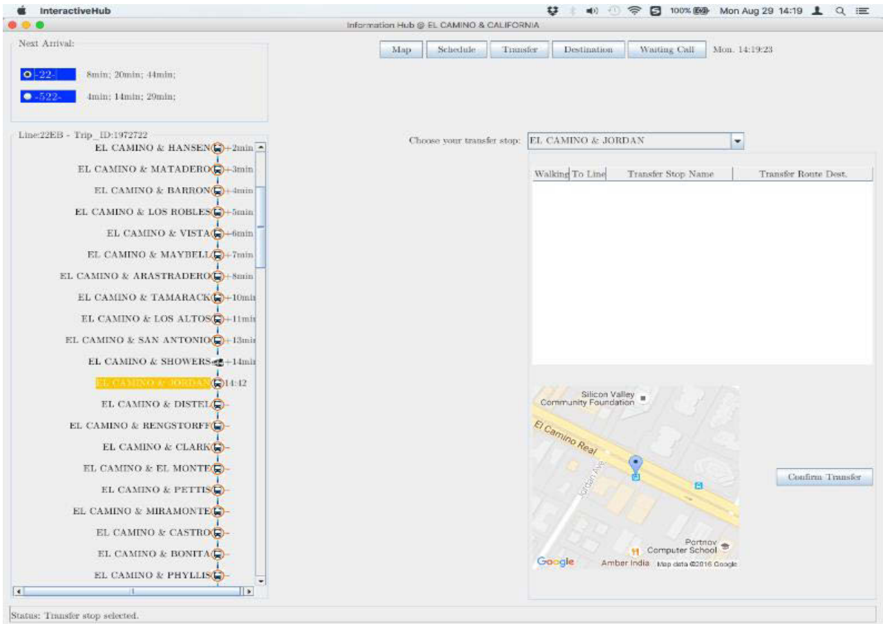
Figure 4-12 Acquire transfer information (d)
