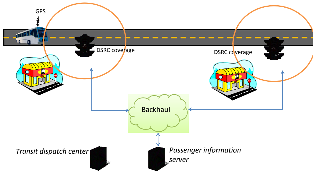
Figure 3-1 DSRC Link and AVL
