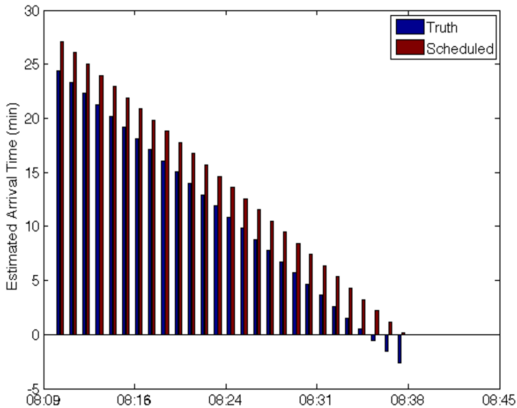
Figure 4-18 Differences between the schedule and the actual arrival along the time (a) Ahead of schedule
