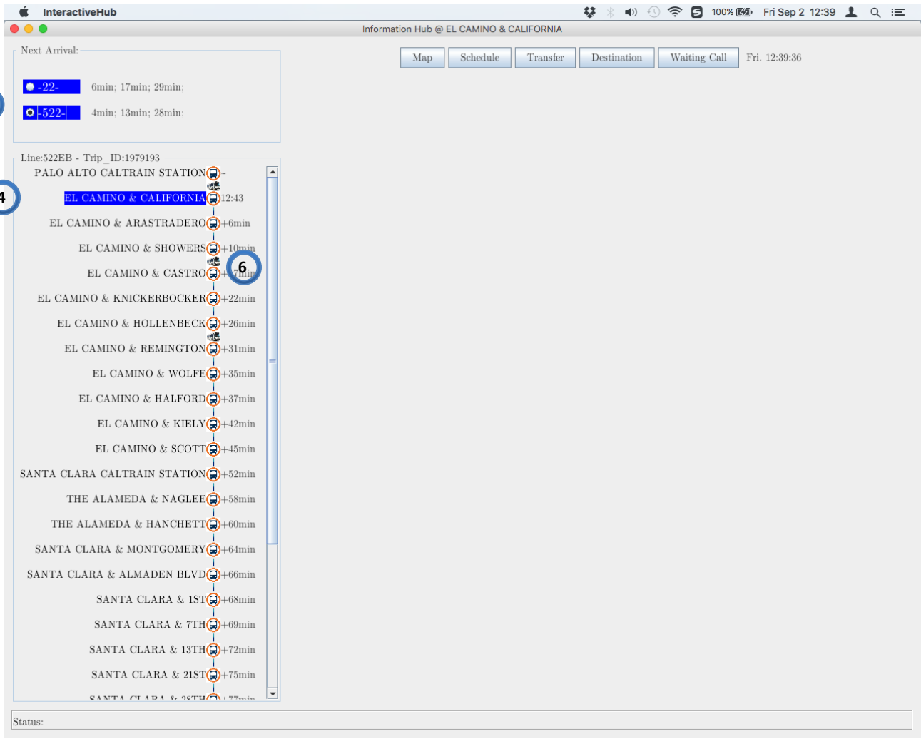
Figure 4-6 Basic Interface Frame (b)
