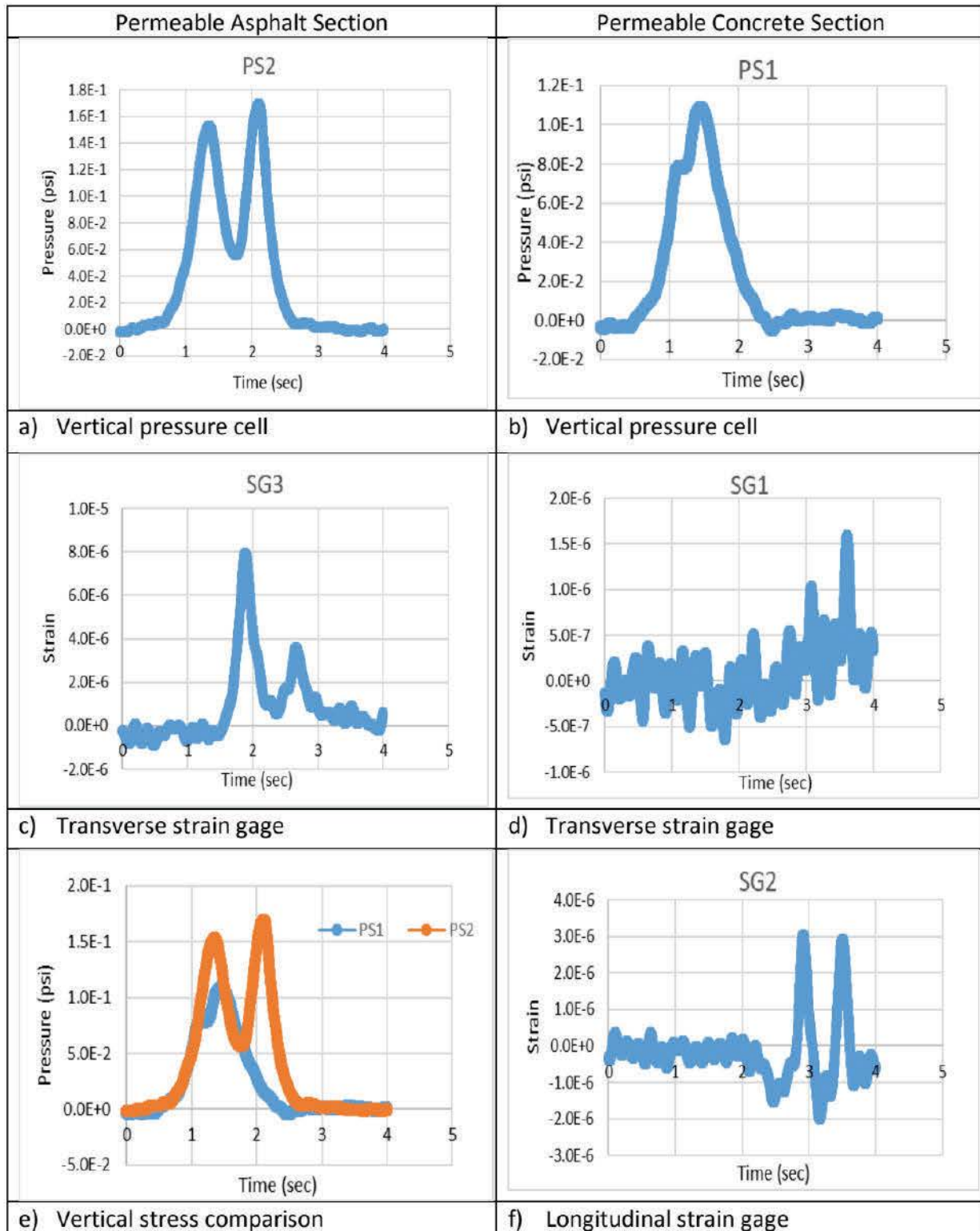
Figure 18. Data comparison of asphalt and concrete sections for vehicle 6
