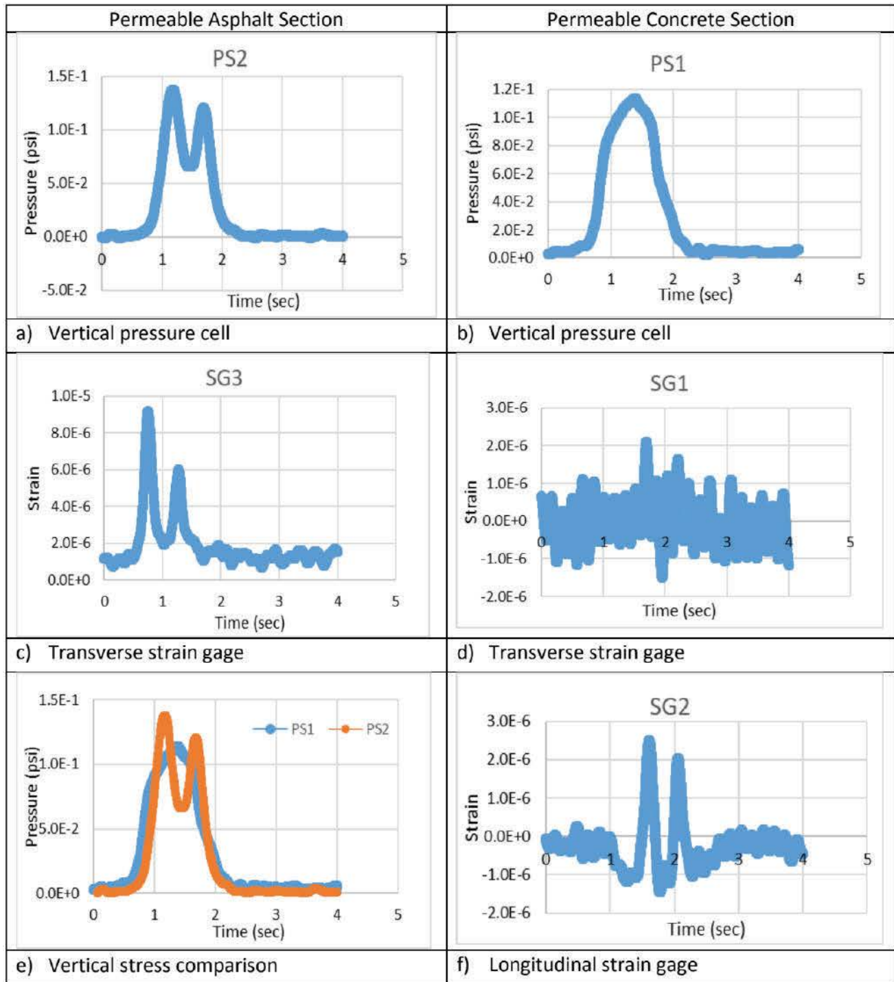
Figure 13. Data comparison of asphalt and concrete sections for vehicle 1
