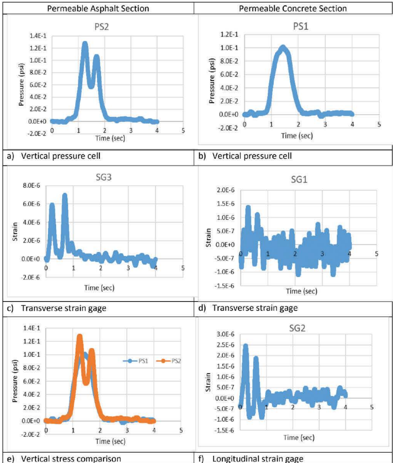
Figure 17. Data comparison of asphalt and concrete sections for vehicle 5
